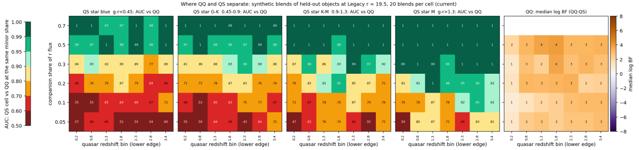
Figure 24: Where QQ and QS separate, at blend Legacy r = 19.5 . First four panels: AUC of log BF between QS blends with a companion of the given g-r stratum and QQ blends at the same minor share, by quasar redshift and companion share of the r flux (20 blends per class per cell, current). Last panel: median log BF of the QQ blends (minor shares up to 0.5).
