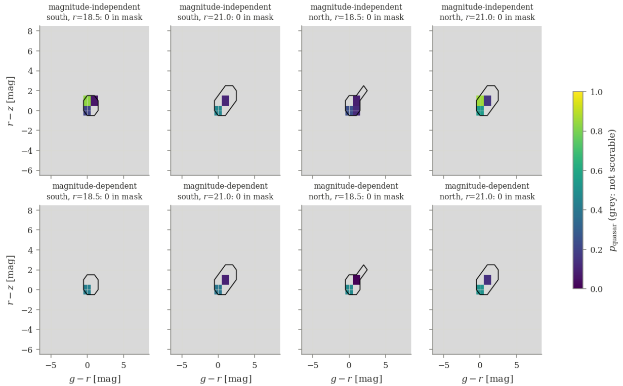
Figure 18: Total quasar probability on artificial Legacy colour grids, South and North, r = 18.5 and 21. Grey cells are not ranked. Black outline: the models' dense core; outside it both the quasar and the background intensity are below 1% of their grid maximum.
