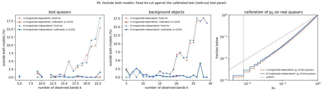
Figure 11: Outside both models, against the number of observed bands k , for the earlier fixed 4\sigma cut (dotted) and the calibrated test at \alpha = 2/256 (solid), for held-out test quasars (left) and background objects (middle), both models. Right: cumulative distribution of p_Q for the test quasars (dotted: uniform; dashed: \alpha ).
