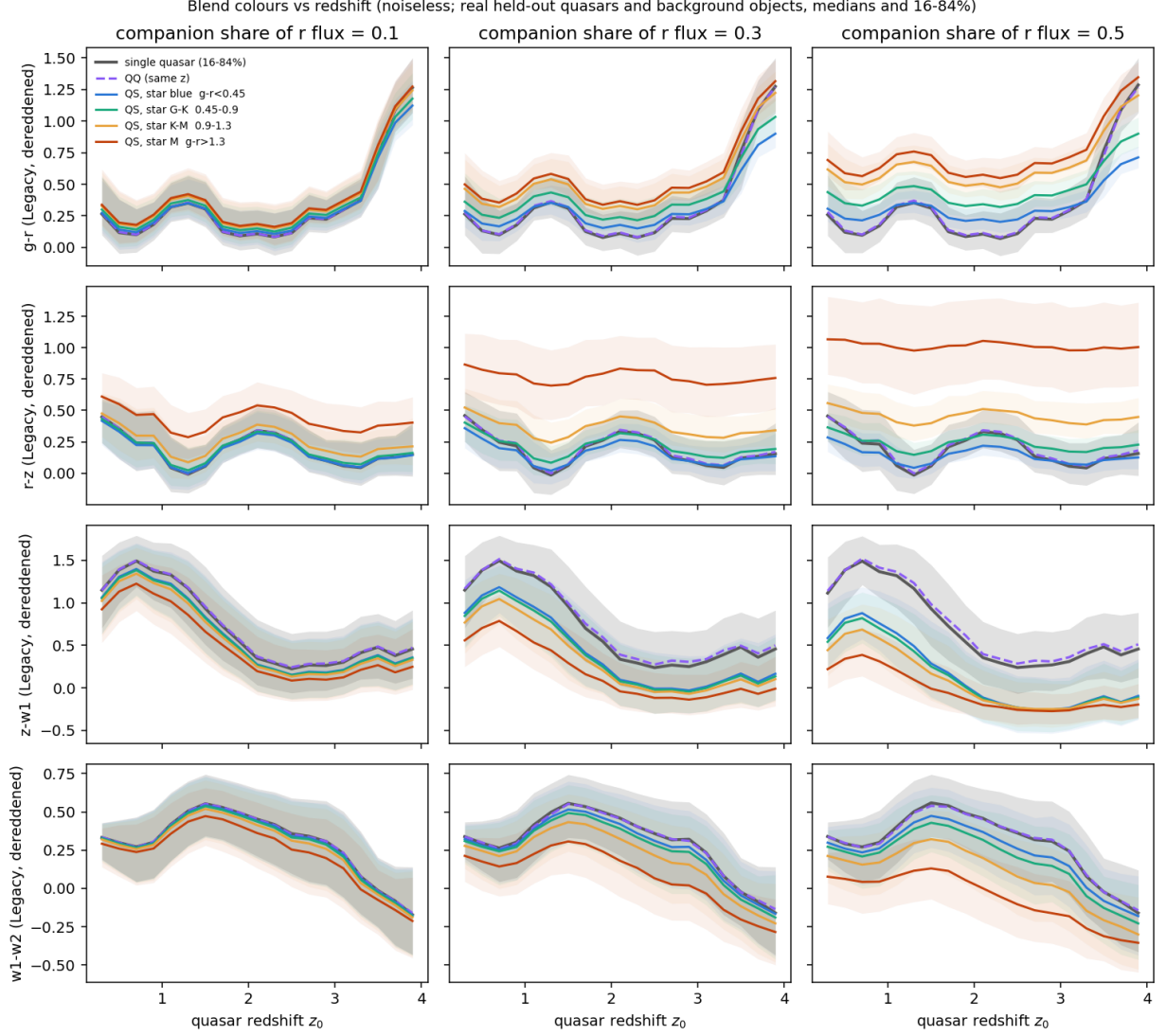
Figure 22: Blend colours (Legacy, dereddened, noiseless) against quasar redshift for companion shares of the r flux of 0.1, 0.3 and 0.5. Grey: single quasars (median and 16–84%). Dashed purple: QQ blends at the same redshift. Coloured: QS blends for the four g - r strata of background objects (median, 16–84% shaded).
