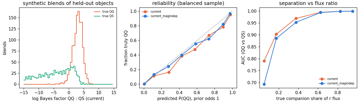
Figure 21: Blend mode on synthetic blends of held-out objects. Left: Bayes factor QQ:QS for true QQ and true QS blends ( current ). Middle: reliability of P(QQ) at prior odds 1 on the balanced sample, both models. Right: AUC against the companion’s true share of the r flux.
