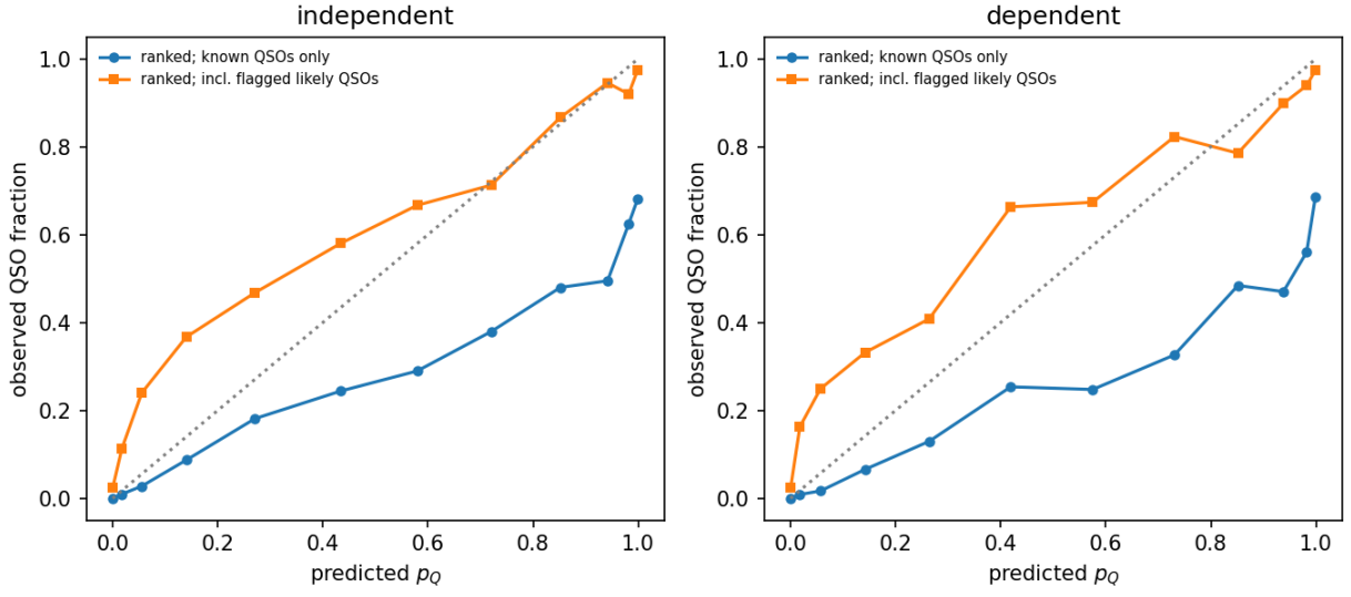
Figure 19: Reliability of p_{\text{quasar}} among ranked objects in the 49 test cones (natural population, weighted), for both models: observed quasar fraction against mean predicted p_{\text{quasar}} in bins, counting known quasars only (blue, lower bound) or also flagged likely quasars (orange, upper bound). Dotted: perfect calibration. Abstention rates are given in the text.
