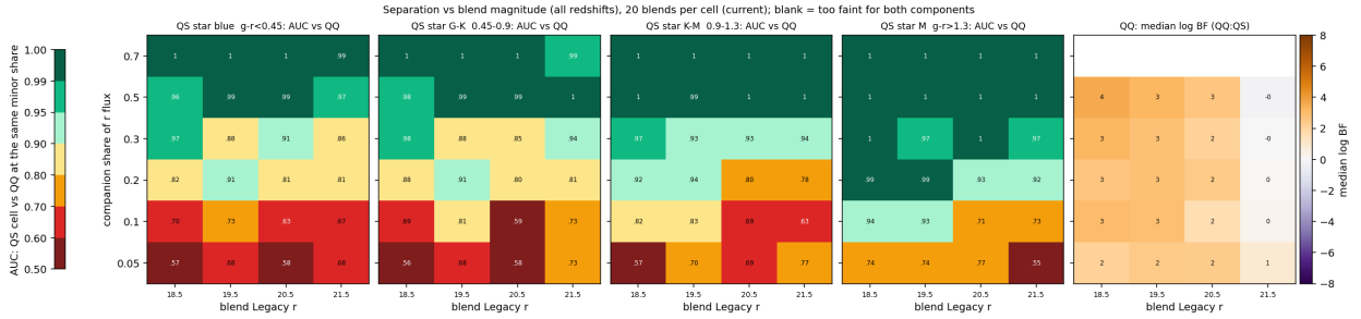
Figure 25: As Fig. 24, against blend Legacy r , with quasar redshifts drawn from the whole test sample.
