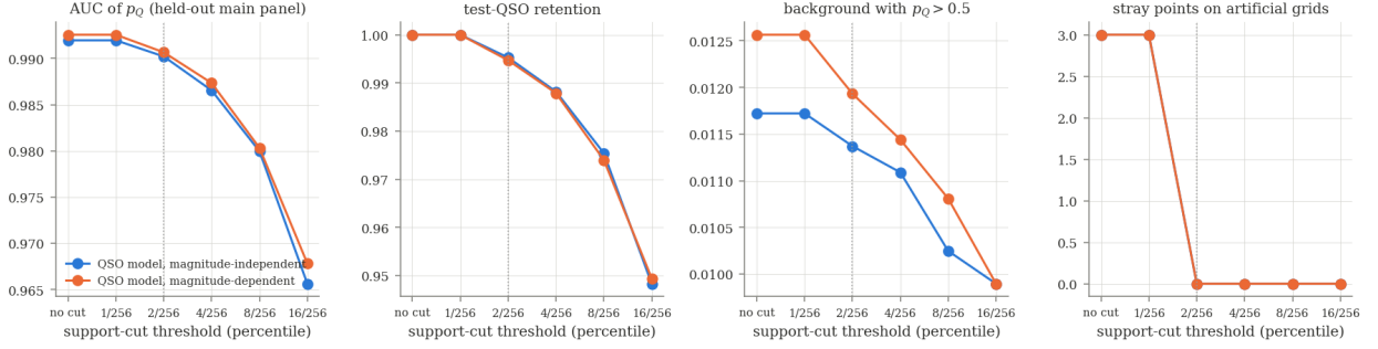
Figure 10: Support-cut threshold (percentile; dotted: the calibrated 2/256 ) on the held-out main panels of Section 10.3 and the artificial grids of Section 10.4: AUC of p_{\text{quasar}} (the scorer does not compute \log \mathcal{R} for rejected objects, so p_{\text{quasar}} ranks all thresholds alike; unranked objects at the bottom), fraction of test quasars kept, fraction of background objects with p_{\text{quasar}} > 0.5 , and grid points with p_{\text{quasar}} > 0.5 in the low-density mask.
