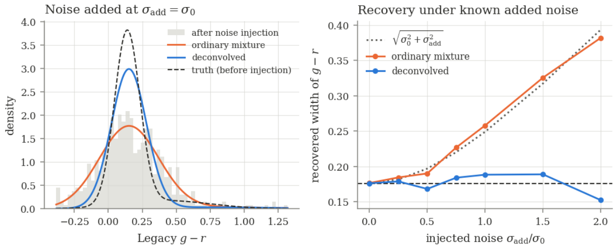
Figure 2: Deconvolution tested by controlled noise injection on real quasar colours: Legacy g - r of the 473 bright quasars ( u_r < 20 , |z - 1.8| < 0.15 ) of the training draw, whose measurement errors are small; fitted width \sigma_0 = 0.176 . Gaussian noise of known size is added and a two-component mixture refitted. Left : at \sigma_{\text{add}} = \sigma_0 the deconvolved mixture (blue) stays close to the pre-injection truth (dashed) while the ordinary mixture (orange) is broadened. Right : the ordinary mixture follows \sqrt{\sigma_0^2 + \sigma_{\text{add}}^2} , reaching 0.382 at \sigma_{\text{add}} = 2\sigma_0 ; extreme deconvolution stays within 8% of \sigma_0 up to 1.5\sigma_0 and returns 0.152 (14% low) at 2\sigma_0 , where the sample of 473 is small for the added noise.
