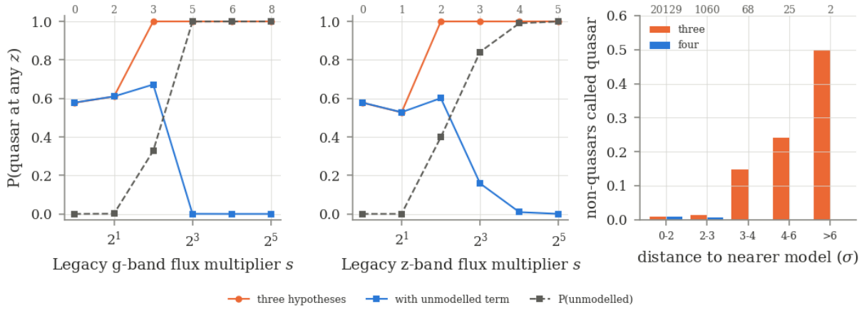
Figure 12: Left, centre: the README candidate with its Legacy g or z flux multiplied by s . Orange: three-hypothesis probability of a quasar at any redshift; blue: the same with U ; grey dashed: P(U) . Numbers along the top are \min(d_Q, d_B) in \sigma . Right: the 21,284 spectroscopic non-quasars of the pair validation, in bins of distance to the nearer model (counts along the top): the fraction called quasars. With U it is zero in every bin beyond 3\sigma .
