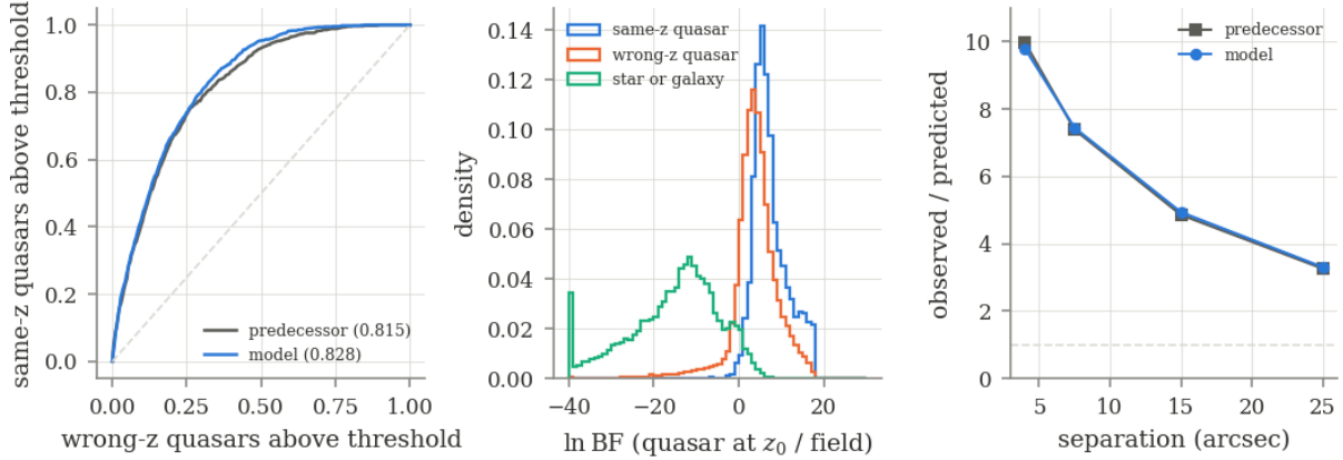
Figure 13: The labelled pairs, scored from Legacy g, r, z, W1, W2 . Left : ROC for same- against wrong-redshift quasar companions in the reserved sky blocks, ranked by \ln R , for the model and its predecessor (AUC in brackets). Centre : the Bayes factor for the three classes (values below -40 are piled at -40 ); the non-quasar class mixes stars with the galaxies DESI targeted. Right : the observed same-redshift fraction among quasar companions divided by the mean predicted p(z \in W \mid \mathbf{u}, Q) , by separation. A defect in the scorer would give a flat ratio; physical clustering gives one that falls with separation.
