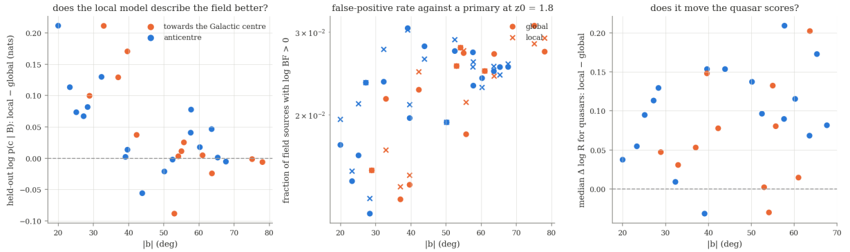
Figure 18: Global against local field model in 30 cones. Left: held-out log density of each cone’s own field sources, local minus global. Centre: fraction of held-out field sources with \log \text{BF} > 0 against a primary at z_0 = 1.8 , under each model. Right: median shift in \log R for the DESI quasars in the cone. Orange: cones facing the Galactic centre; blue: anticentre. Computed with the predecessor Legacy model (Appendix C).
