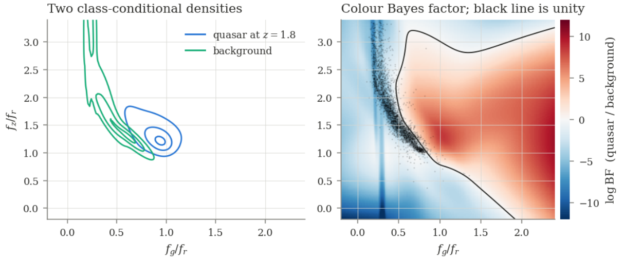
Figure 7: Left : the quasar density at z = 1.8 and the local background density, both fitted to real data, in the same feature plane. Right : the colour Bayes factor (6); the black contour is \text{BF} = 1 , and black points are real catalogue sources at the relevant magnitude. Most of the field population sits where the Bayes factor strongly disfavours the quasar hypothesis, but the two loci are not disjoint. Computed with the predecessor Legacy model (Appendix C).
