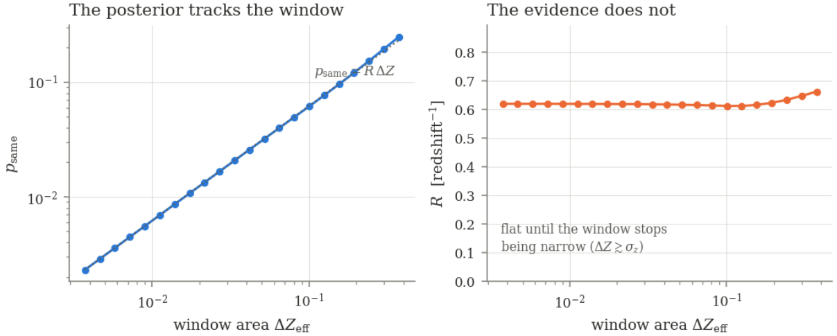
Figure 9: The factorisation on a real quasar. Left: p_{\text{same}} is proportional to the window area over more than a decade, as (17) requires; the dotted line is R \Delta Z with R from the narrowest window. Right: R is flat until the window stops being narrow compared with \sigma_z . Computed with the predecessor model; the factorisation is a property of (1)–(15), not of a particular density.
