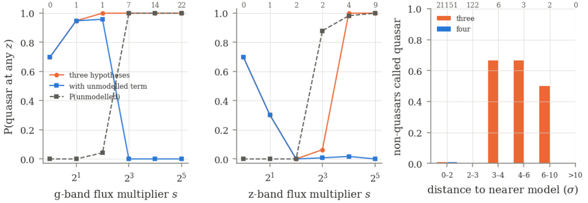
Figure 11: Left, centre: the README candidate with its g or z flux multiplied by s . Orange: the three-hypothesis posterior probability of a quasar at any redshift; blue: the same with the unmodelled term; grey dashed: P(U) . Numbers along the top are \min(d_Q, d_B) in \sigma . Right: the 21,284 spectroscopic non-quasars of the pair validation, in bins of the distance to the nearer model (counts along the top): the fraction called quasars. With U that fraction is zero in every bin beyond 2\sigma . Computed with the predecessor Legacy model (Appendix C).
