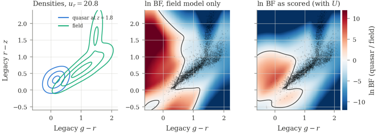
Figure 7: Left : the quasar density at z = 1.8 and the field density in the Legacy g-r , r-z plane, both conditioned on u_r = 20.8 ; the field is the dedicated Legacy g, r, z fit the scorer uses for Legacy-only input (§5.3). Contours at 5, 30 and 80% of each peak. Centre : the Bayes factor against the field model alone, as three hypotheses would have it: far from both loci, where neither density has support, it is set by which Gaussian tail is wider. Right : the Bayes factor as scored, against (1-\eta)p_B + \eta p_U with the Student-t U of §8: positive values remain only on and around the quasar locus. The black contour is \text{BF} = 1 ; black points are field sources within 0.4 of u_r = 20.8 .
