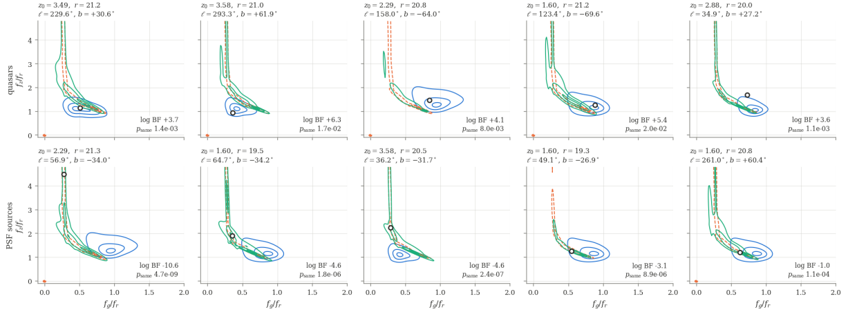
Figure 9: Ten real objects scored on DECaLS colours alone. Top : five DESI DR1 quasars from the model’s reserved sky blocks, never used in fitting. Bottom : five point sources, each from a different random field. Contours are the quasar model at z_0 (blue), the stellar model averaged over the footprint (orange, dashed) and the stellar model fitted in this object’s own neighbourhood (green). Panel titles give the target redshift, reference magnitude and Galactic coordinates; the measured object is the open circle with its error bars. Note that the outermost contour is drawn at 5% of peak density, not at an enclosed probability, so an object outside it is not thereby improbable.
