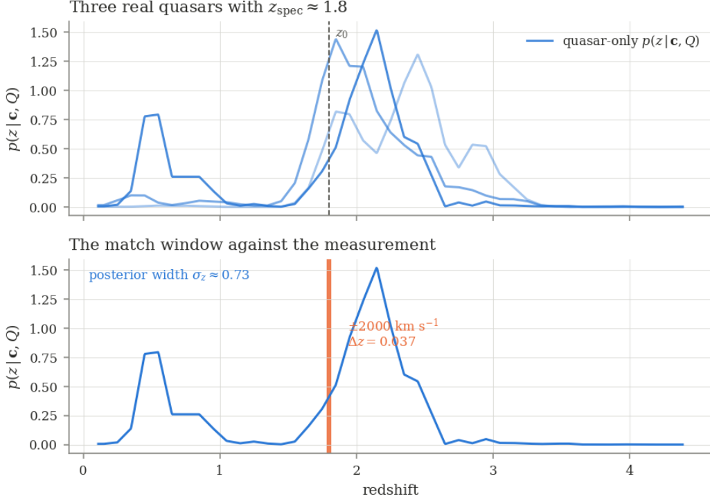
Figure 6: Top : quasar-only redshift posteriors p(z \mid \mathbf{c}, Q) for three real DESI quasars with z_{\text{spec}} \approx 1.8 , showing the width and the secondary solutions that broadband colours cannot resolve. Bottom : the same posterior with a \pm 2000 \text{ km s}^{-1} window drawn to scale. The window is the narrow orange band. The width quoted on the panel is for this object, which is better constrained than most; across 1500 quasars the median width is \sigma_z \approx 0.6 (§7). Note that this is the quasar-only posterior under a flat redshift prior; p_{\text{same}} integrates the same window against \Sigma_Q(z, m) p(\mathbf{c} \mid Q, z) instead. The panel shows the scale of the mismatch between window and measurement, which is what makes p_{\text{same}} small, not the quantity itself.
