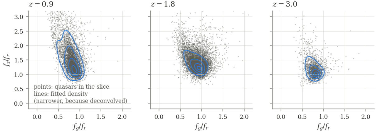
Figure 3: The fitted conditional density p(\mathbf{c} | Q, z) at three redshifts (contours), with the quasars in each slice (points). The locus translates and changes shape with redshift; each slice is a separate deconvolved mixture, so no linear colour–redshift relation is imposed. The contours are visibly tighter than the scatter of the points because the model is the deconvolved density, while the points carry their measurement errors (§4.2). Note also how much the three loci overlap: this is the origin of the weak redshift discrimination quantified in §7.6.
