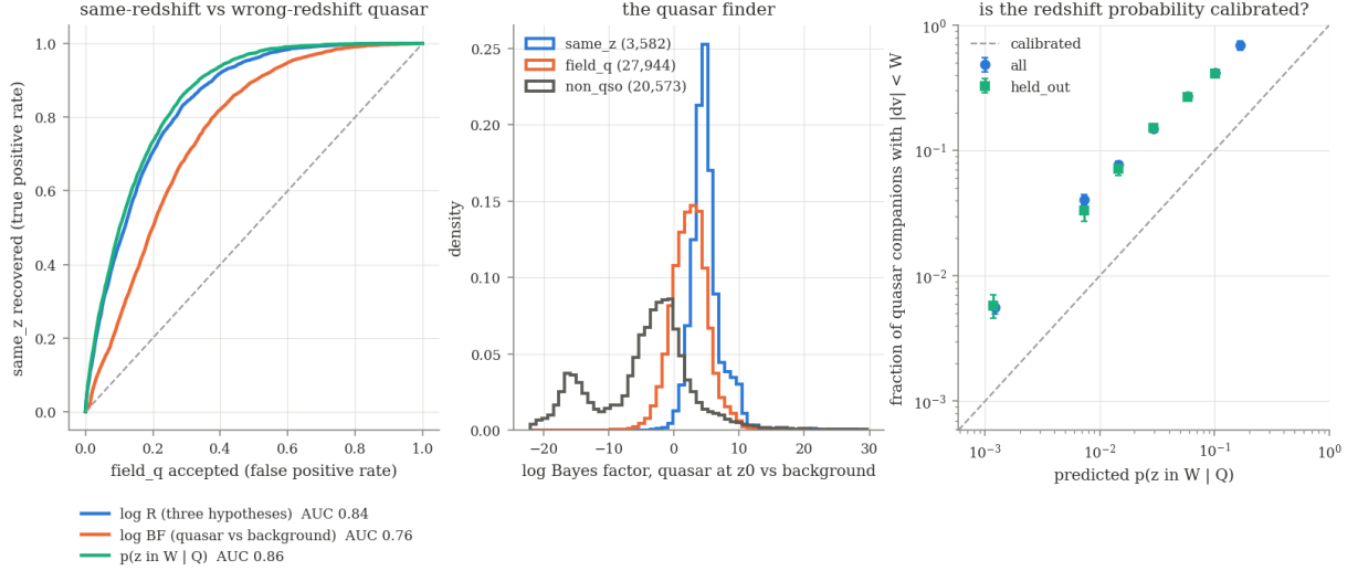
Figure 10: Validation on spectroscopically labelled pairs. Left : ROC for same-redshift against wrong-redshift quasar companions, ranked three ways. Centre : the Bayes factor against background for the three classes; the non_qso class is bimodal because it mixes stars (left peak) with the galaxies DESI targeted (right peak, overlapping the quasars). Right : reliability of p(z \in W | \mathbf{c}, Q) among quasar companions. The points lie on a line parallel to the diagonal: the predicted probability is right in shape and low by a constant factor, which is the signature of physical clustering that the scorer deliberately does not model.
