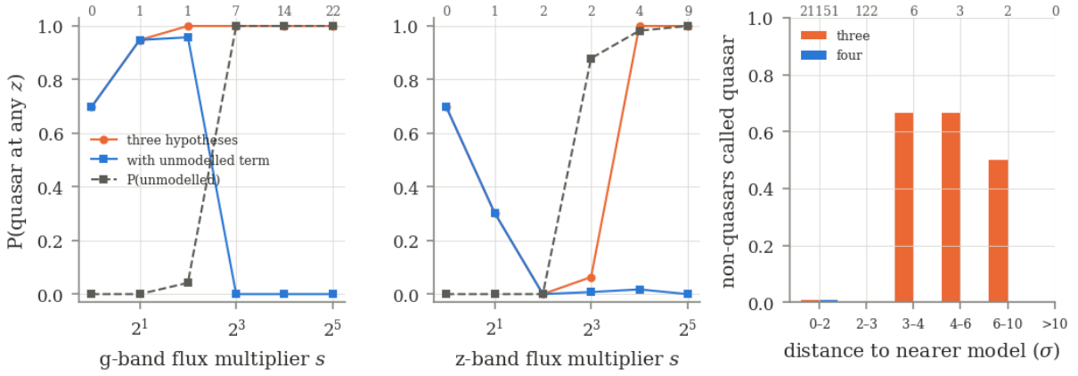
Figure 7: Left, centre: the README candidate with its g or z flux multiplied by s . Orange: the three-hypothesis posterior probability of a quasar at any redshift; blue: the same with the unmodelled term; grey dashed: P(U) . Numbers along the top are \min(d_Q, d_B) in \sigma . Right: the 21,284 spectroscopic non-quasars of the pair validation, in bins of the distance to the nearer model (counts along the top): the fraction called quasars. With U that fraction is zero in every bin beyond 2\sigma .
