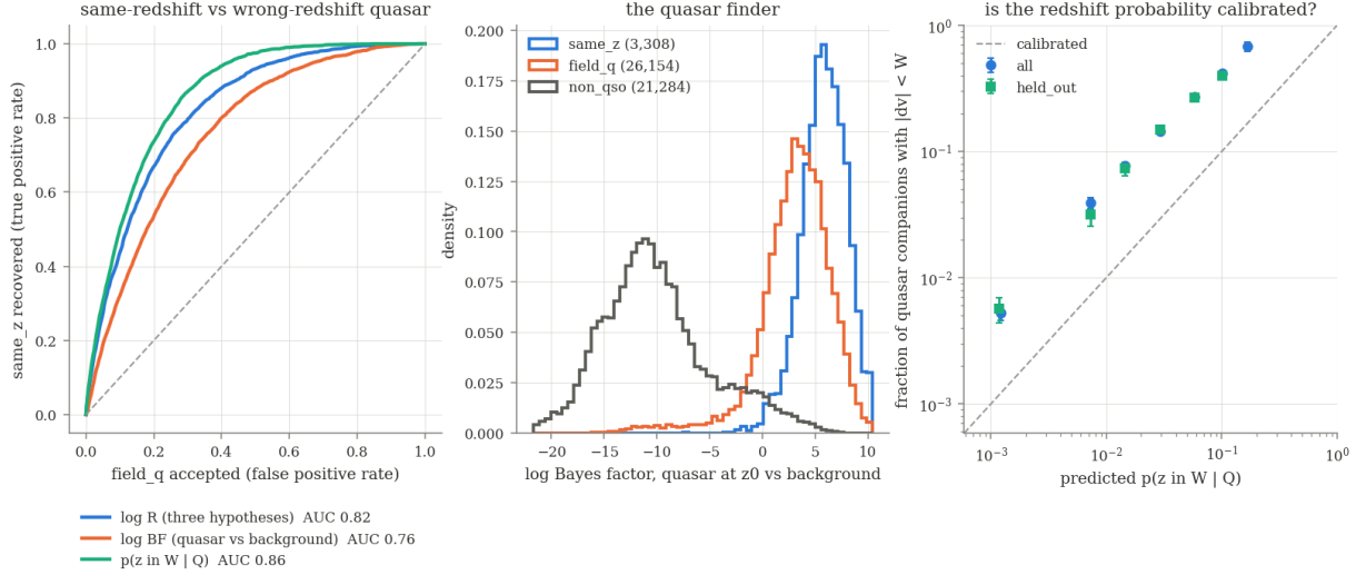
Figure 15: Validation on spectroscopically labelled pairs. Left : ROC for same-redshift against wrong-redshift quasar companions, ranked three ways. Centre : the Bayes factor against background for the three classes; the non_qso class is bimodal because it mixes stars (left peak) with the galaxies DESI targeted (right peak, overlapping the quasars). Right : reliability of p(z \in W | \mathbf{c}, Q) among quasar companions. The points lie on a line parallel to the diagonal: the predicted probability is right in shape and low by a constant factor, which is the signature of physical clustering that the scorer deliberately does not model.
