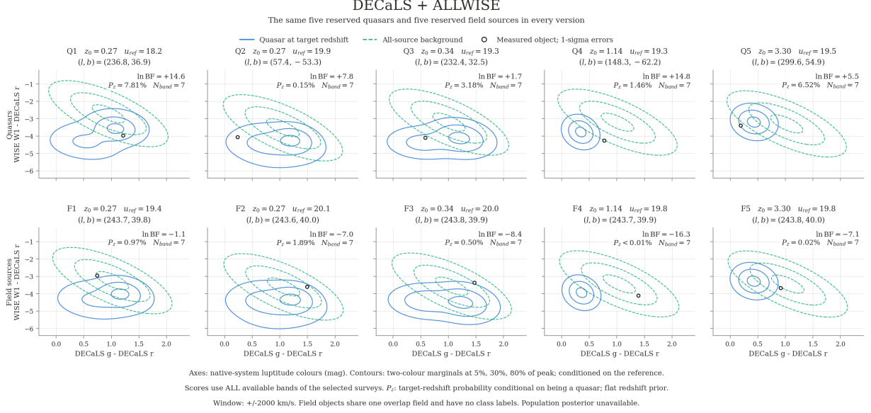
Figure 12: One of the twelve survey-combination versions: DECaLS+ALLWISE. The fixed quasars Q1–Q5 and field sources F1–F5 recur in every version. Contours show two-colour marginals conditional on the reference; panel scores use all seven available bands in this combination. The upper and lower panels in a column share the same target redshift. P_z assumes the object is a quasar and is not p_{\text{same}} . Full-size versions, including ALLWISE-only and VHS-only, are in the accompanying atlas.
