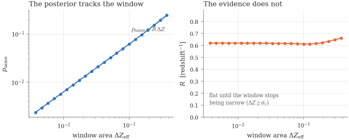
Figure 9: The factorisation, on a real quasar. Left: p_{\text{same}} is proportional to the window area over more than a decade, exactly as (21) requires; the dotted line is R \Delta Z with R taken from the narrowest window. Right: R itself is flat, departing only when the window stops being narrow compared with \sigma_z and the approximation in (18) is no longer appropriate.
