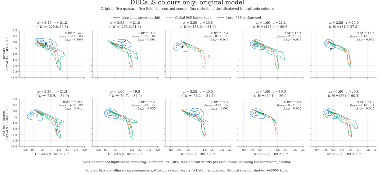
Figure 11: Ten real objects scored on DECaLS colours alone. Top : five DESI DR1 quasars from the model’s reserved sky blocks, never used in fitting. Bottom : five point sources, each from a different random field. Contours are the quasar model at z_0 (blue), the stellar model averaged over the footprint (orange, dashed) and the stellar model fitted in this object’s own neighbourhood (green). Panel titles give the target redshift, reference magnitude and Galactic coordinates; the measured object is the open circle with its error bars and covariance ellipse. The axes now show dereddened luptitude colours u_g - u_r and u_z - u_r , using the southern Legacy softening parameters saved with the seven-survey model. The original flux-ratio model densities are transformed at each object’s measured reference flux, including the change-of-variables Jacobian. The objects, trained models and scores are unchanged. These contours remain intrinsic densities, before measurement-noise convolution. Note that the outermost contour is drawn at 5% of peak density, not at an enclosed probability, so an object outside it is not thereby improbable.
