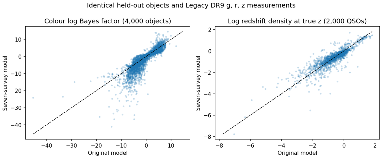
Figure 16: Fresh matched-sample comparison after the background correction. Left: colour Bayes factors for all 4,000 objects. Right: normalised redshift densities at the true redshift for 2,000 quasars. The dashed line is equality. Good agreement in discrimination does not imply equal scores for every object.
