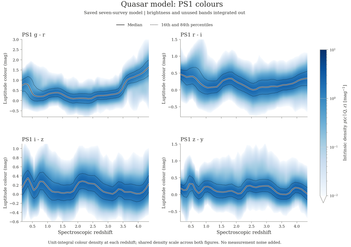
Figure 14: The four adjacent PS1 colours, g-r , r-i , i-z and z-y , against spectroscopic redshift. Normalisation, marginalisation, quantile curves and density scale are identical to Figure 13. These marginals retain the separately labelled PS1 bands of the joint model; they do not substitute DECaLS colours.
