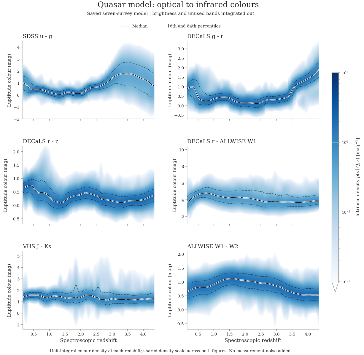
Figure 13: Intrinsic quasar colour densities from the seven-survey model: SDSS u - g , southern DECaLS g - r and r - z , DECaLS r –ALLWISE W1, VHS J - K_s , and ALLWISE W1–W2. Brightness and all unused bands are marginalised. Each redshift column is a unit-integral colour density; the shading measures density per magnitude, not source counts. Median and central 68% limits are overlaid. The density scale is shared with Figure 14.
