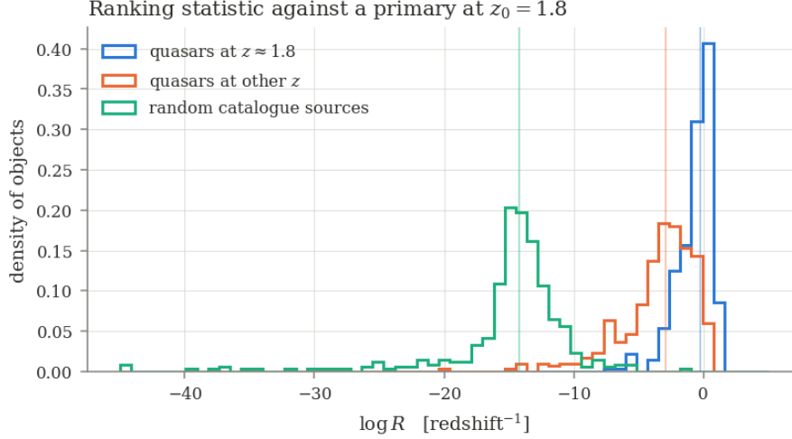
Figure 10: The ranking statistic evaluated against a primary at z_0 = 1.8 , for real quasars at that redshift ( |z - z_0| < 0.05 ), real quasars at other redshifts ( |z - z_0| > 0.6 ), and random catalogue sources. Vertical lines mark the medians. Two limits of this comparison: the “same” class extends to 2.7 times the window half-width, so not all of it lies inside the window being scored; and nothing populates the gap between 0.05 and 0.6, which is where discrimination is genuinely hardest. The quasars are drawn from the sixteen sky blocks the model reserved before fitting (21,826 available in this cone), so the comparison is out of sample. The quasar populations separate from the field by \sim 14 natural logarithms but from each other by only \sim 2.6 : grz + W1W2 photometry identifies quasars far better than it locates them in redshift (§8.6). The figure shows the statistic’s dynamic range, not an operating characteristic.
