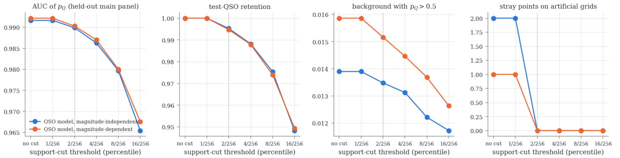
Figure 12: Support-cut threshold (percentile; dotted: the calibrated 2/256 ) on the held-out main panels of Section 10.3 and the artificial grids of Section 10.4: AUC of p_{\text{quasar}} (the scorer does not compute \log \mathcal{R} for rejected objects, so p_{\text{quasar}} ranks all thresholds alike; unranked objects at the bottom), fraction of test quasars kept, fraction of background objects with p_{\text{quasar}} > 0.5 , and grid points with p_{\text{quasar}} > 0.5 in the low-density mask.
