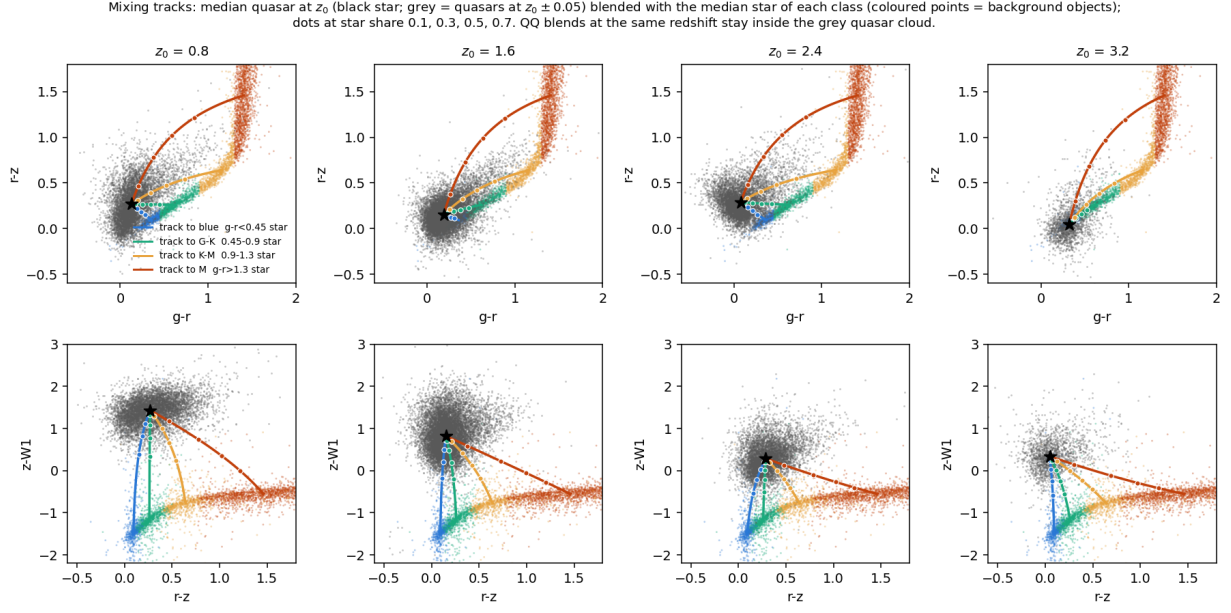
Figure 25: Mixing tracks in g-r against r-z (top) and r-z against z-W1 (bottom) at four redshifts. Grey: quasars at z_0 \pm 0.05 ; black star: their median. Coloured points: background objects by g-r stratum. Lines: blend of the median quasar with the median star of each stratum as the star's share of the r flux goes from 0 to 1; dots at shares 0.1, 0.3, 0.5 and 0.7.
