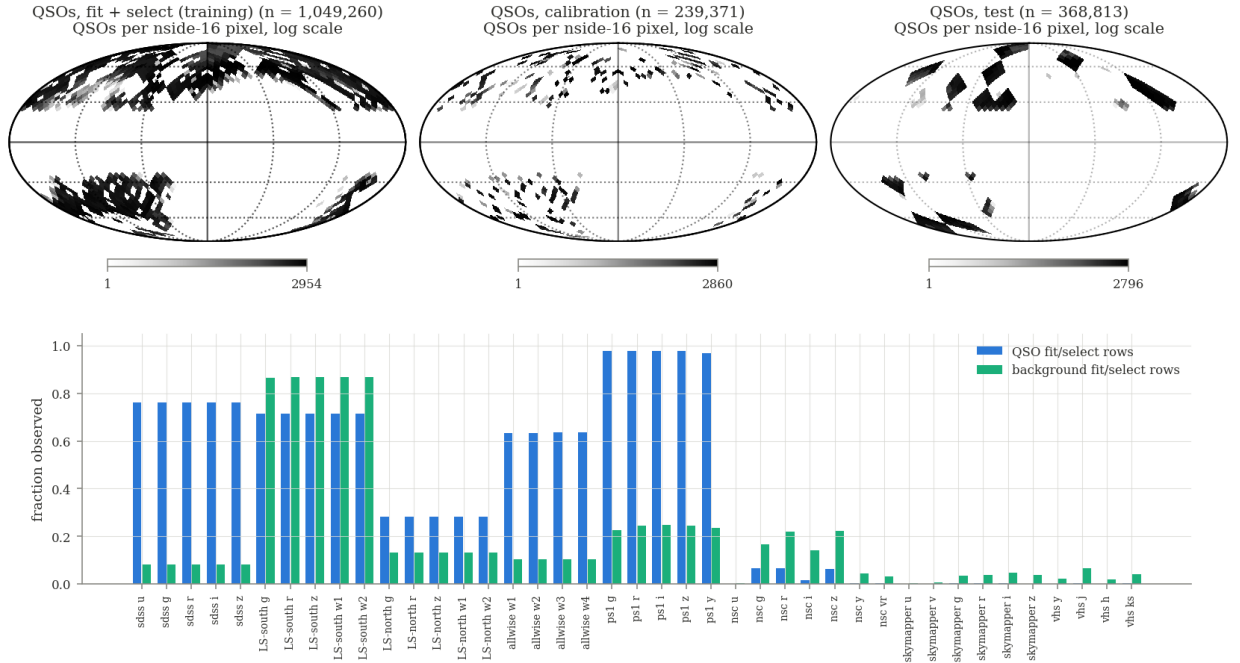
Figure 3: Top: sky distribution of quasars by role, Galactic Mollweide projection, counts per HEALPix n_{\text{side}}=16 pixel (log scale). Bottom: fraction of fit/select rows with each band observed, for quasars (blue) and the background (aqua).
