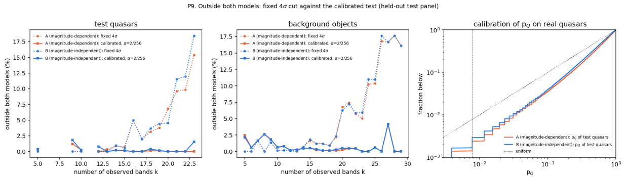
Figure 13: Outside both models, against the number of observed bands k , for the earlier fixed 4\sigma cut (dotted) and the calibrated test at \alpha = 2/256 (solid), for held-out test quasars (left) and background objects (middle), both models. Right: cumulative distribution of p_Q for the test quasars (dotted: uniform; dashed: \alpha ).
