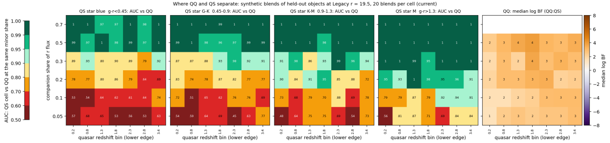
Figure 26: Where QQ and QS separate, at blend Legacy r = 19.5 . First four panels: AUC of log BF between QS blends with a companion of the given g-r stratum and QQ blends at the same minor share, by quasar redshift and companion share of the r flux (20 blends per class per cell, current). Last panel: median log BF of the QQ blends (minor shares up to 0.5).
