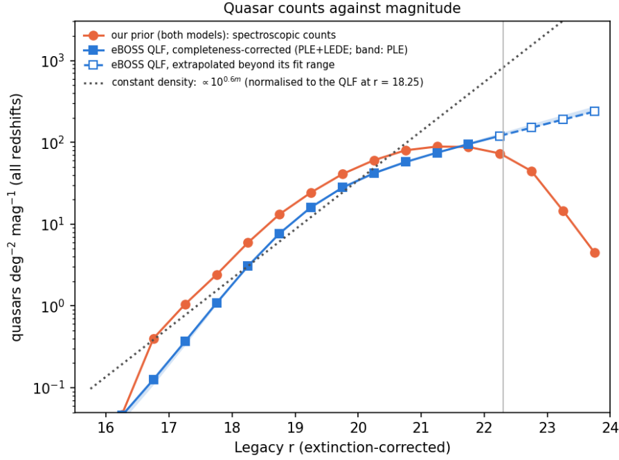
Figure 10: Quasar counts per \text{deg}^2 per magnitude (all redshifts) against extinction-corrected Legacy r : the earlier prior (spectroscopic counts times one constant), the eBOSS luminosity function now used (solid where fitted, dashed where extrapolated; band: PLE against PLE+LEDE), and constant comoving density in Euclidean space ( \propto 10^{0.6m} , normalised at r = 18.25 ).
