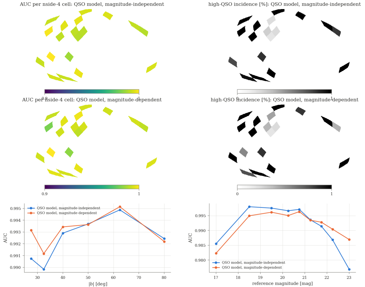
Figure 17: Performance against sky position and magnitude. Top: AUC and high-QSO incidence per HEALPix nside-4 cell (cells with at least 30 objects of each class). Bottom: AUC against |b| and against reference-band magnitude.
