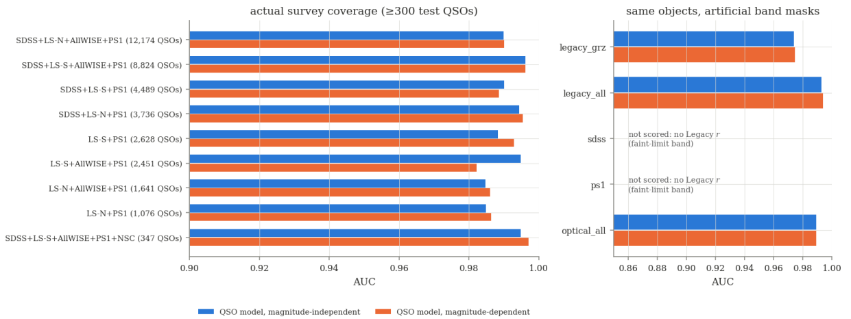
Figure 19: AUC by band coverage. Left: objects grouped by the surveys that observed them (groups with at least 300 test quasars). Right: the same objects scored with artificial band masks; SDSS-only and PS1-only objects have no Legacy r and are not scored.
