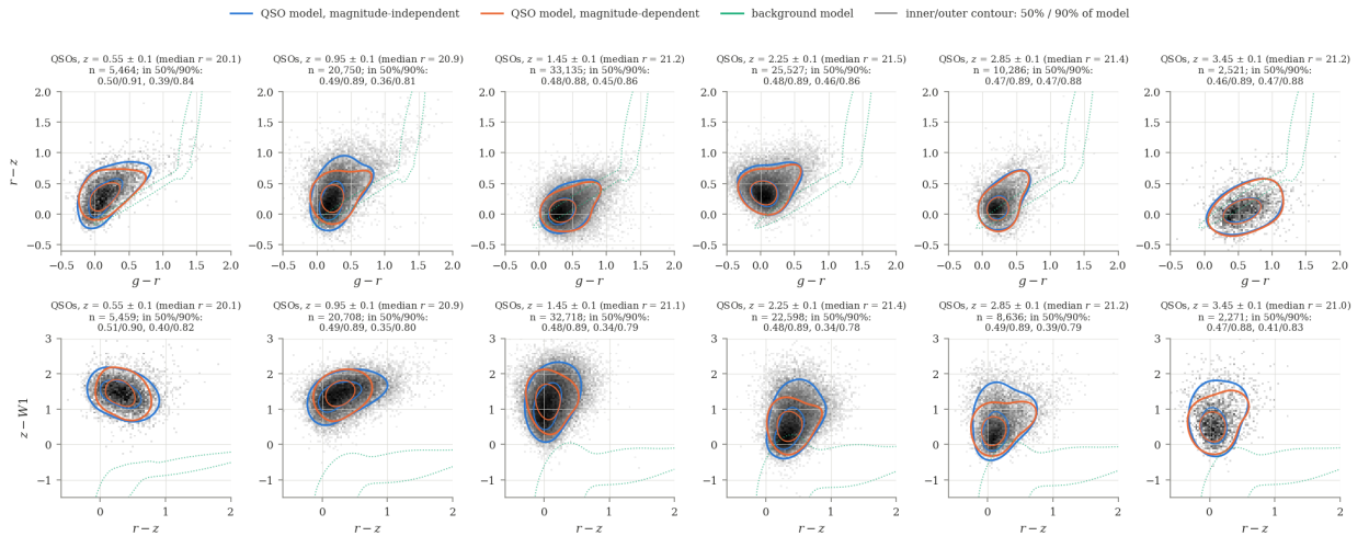
Figure 16: Quasar colour-colour planes in six redshift slices, each conditioned on the slice's median r , with the background model's 90% contour for reference.
