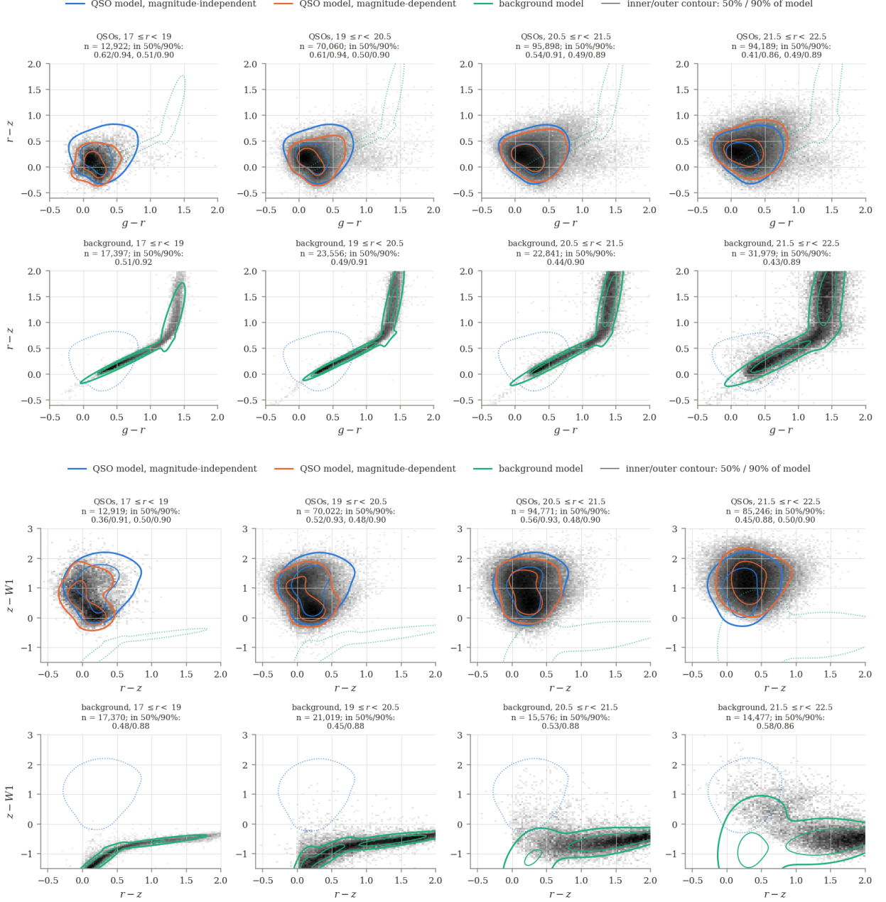
Figure 14: Colour-colour planes in bins of Legacy South r , objects above the faint limit. Top rows of each block: test quasars (grey, log density) with both quasar models (blue, orange; thick and thin contours enclose 90% and 50%) and the background model's 90% contour (dotted aqua). Bottom rows: test background objects (likely quasars removed) with the binned background and the magnitude-independent quasar model's 90% contour (dotted blue).
