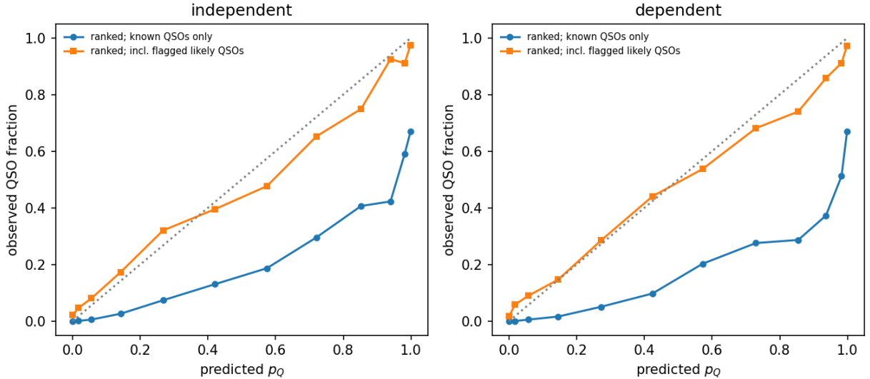
Figure 21: Reliability of p_{\text{quasar}} among ranked objects in the 49 test cones (natural population, weighted), for both models: observed quasar fraction against mean predicted p_{\text{quasar}} in bins, counting known quasars only (blue, lower bound) or also flagged likely quasars (orange, upper bound). Dotted: perfect calibration. Abstention rates are given in the text.
