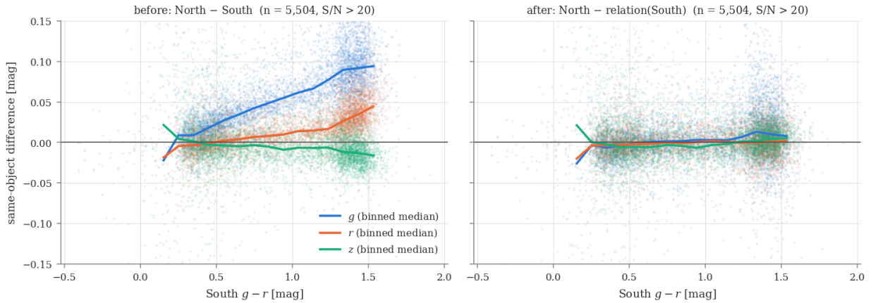
Figure 6: Same-object North minus South luptitudes in overlap fields ( S/N > 20 in all six bands), against South g - r . Left: raw difference. Right: after applying the DESI relation to the southern values. Lines: binned medians.
