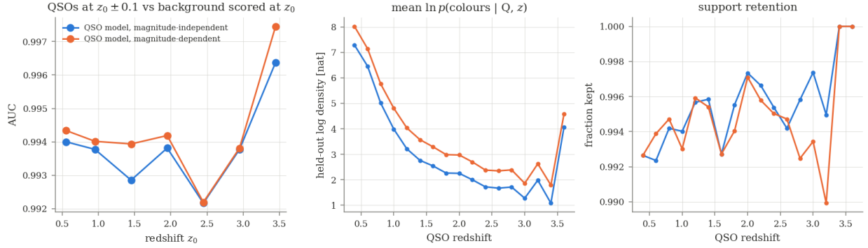
Figure 18: Performance against redshift. Left: AUC of quasars at z_0 \pm 0.1 against background objects scored at z_0 . Middle: mean held-out log density of quasars, in bins of their redshift. Right: support retention.
