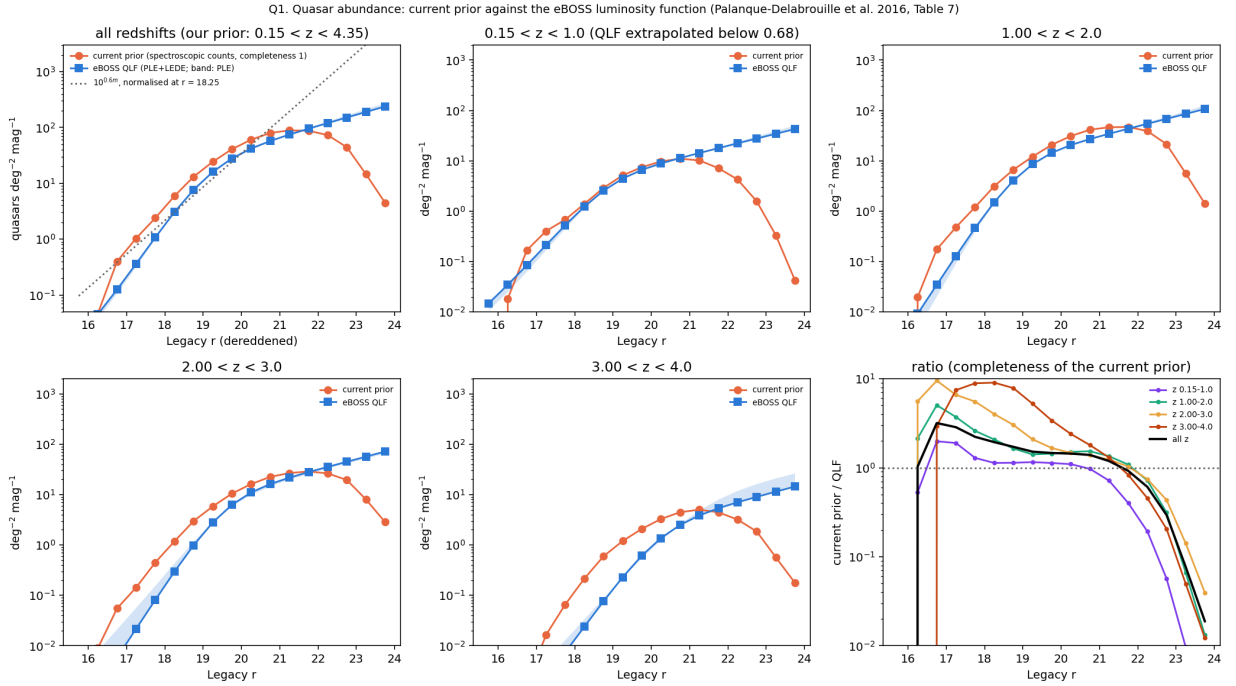
Figure 11: The earlier prior against the eBOSS luminosity function in redshift bins, and their ratio (bottom right), which is the completeness the single constant was meant to correct.
