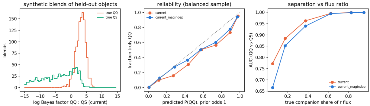
Figure 23: Blend mode on synthetic blends of held-out objects. Left: Bayes factor QQ:QS for true QQ and true QS blends ( current ). Middle: reliability of P(\text{QQ}) at prior odds 1 on the balanced sample, both models. Right: AUC against the companion’s true share of the r flux.
