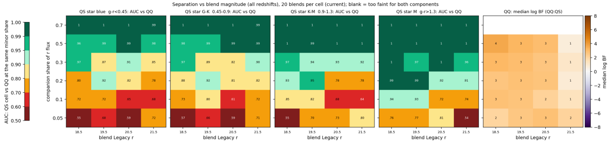
Figure 27: As Fig. 26, against blend Legacy r , with quasar redshifts drawn from the whole test sample.
