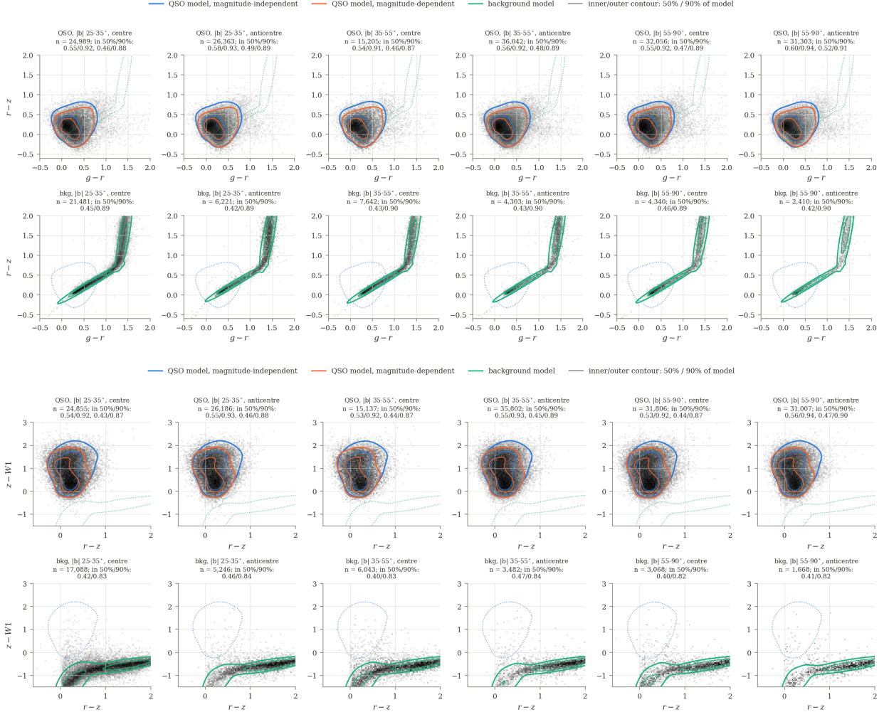
Figure 15: As Fig. 14, in bins of Galactic latitude and of longitude towards ( |l| < 90^\circ ) or away from the Galactic centre, at 19 \leq r < 21.5 . Background contours use the spatial component weights averaged over each bin's objects.
