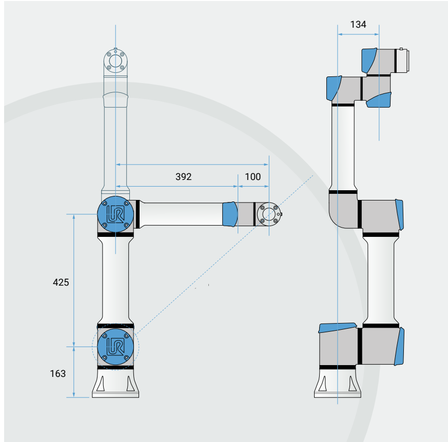
Figure 1: UR5e robot arm dimensions in millimeters.
