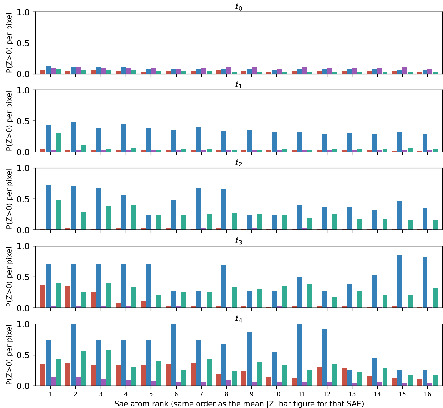
SAE atom fire rate P(Z>0) (SAEatom order as in the atom magnitude |Z| figure)
