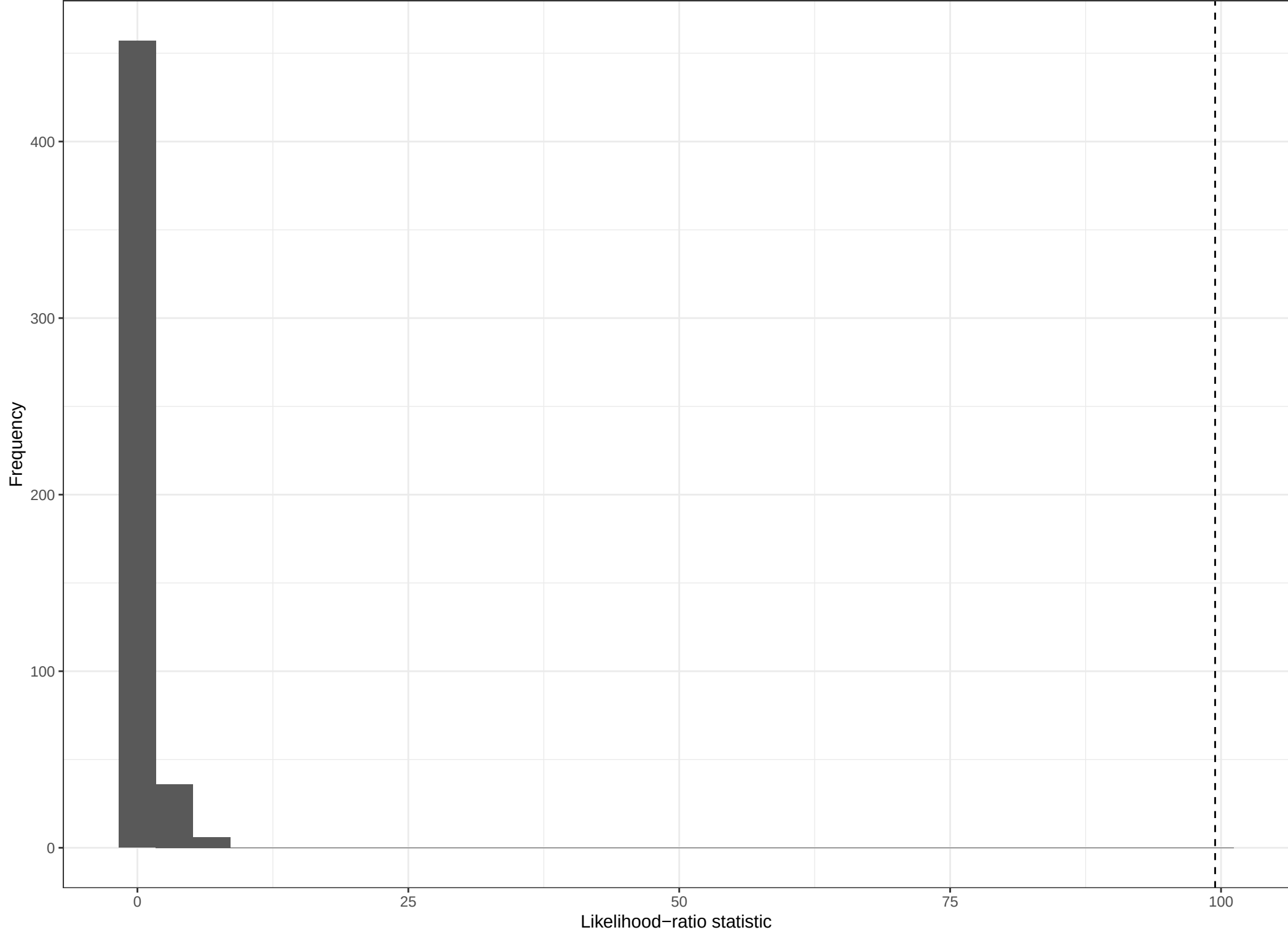
Parametric-bootstrap null distribution for the stage-spell LR statistic Dashed line marks the observed statistic
