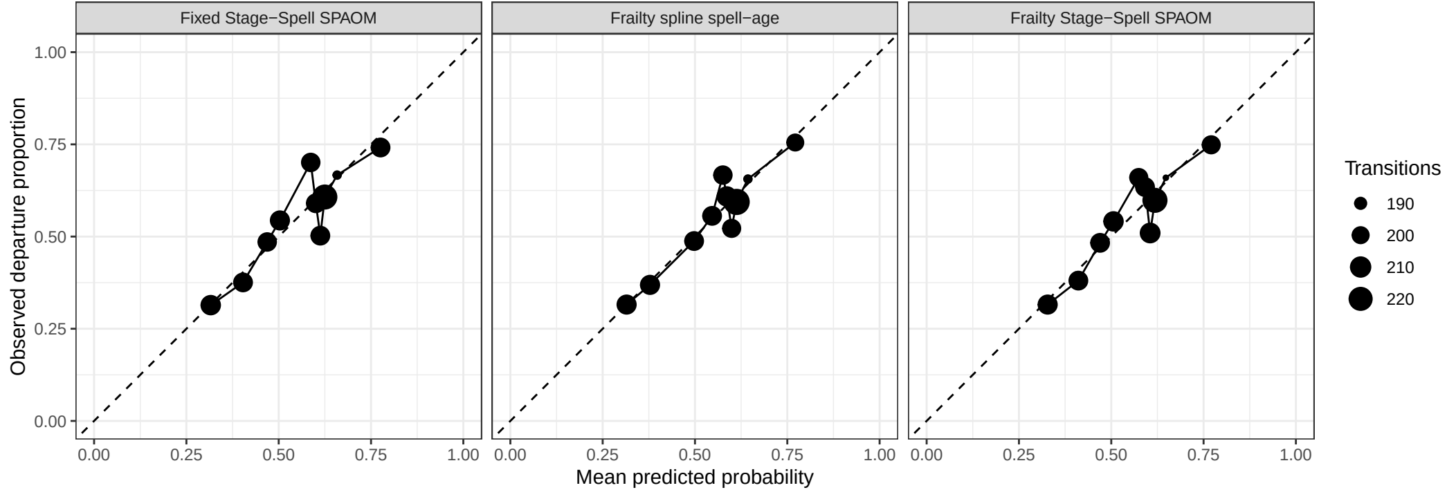
Marginal cross-validated departure calibration
