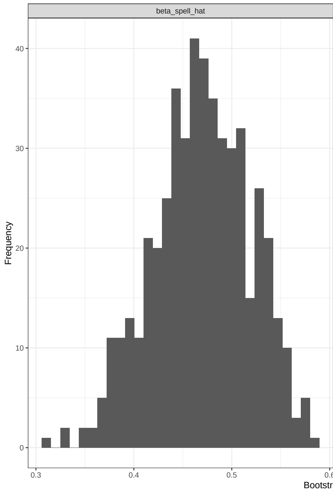
Process-bootstrap distributions for the frailty sensitivity model
