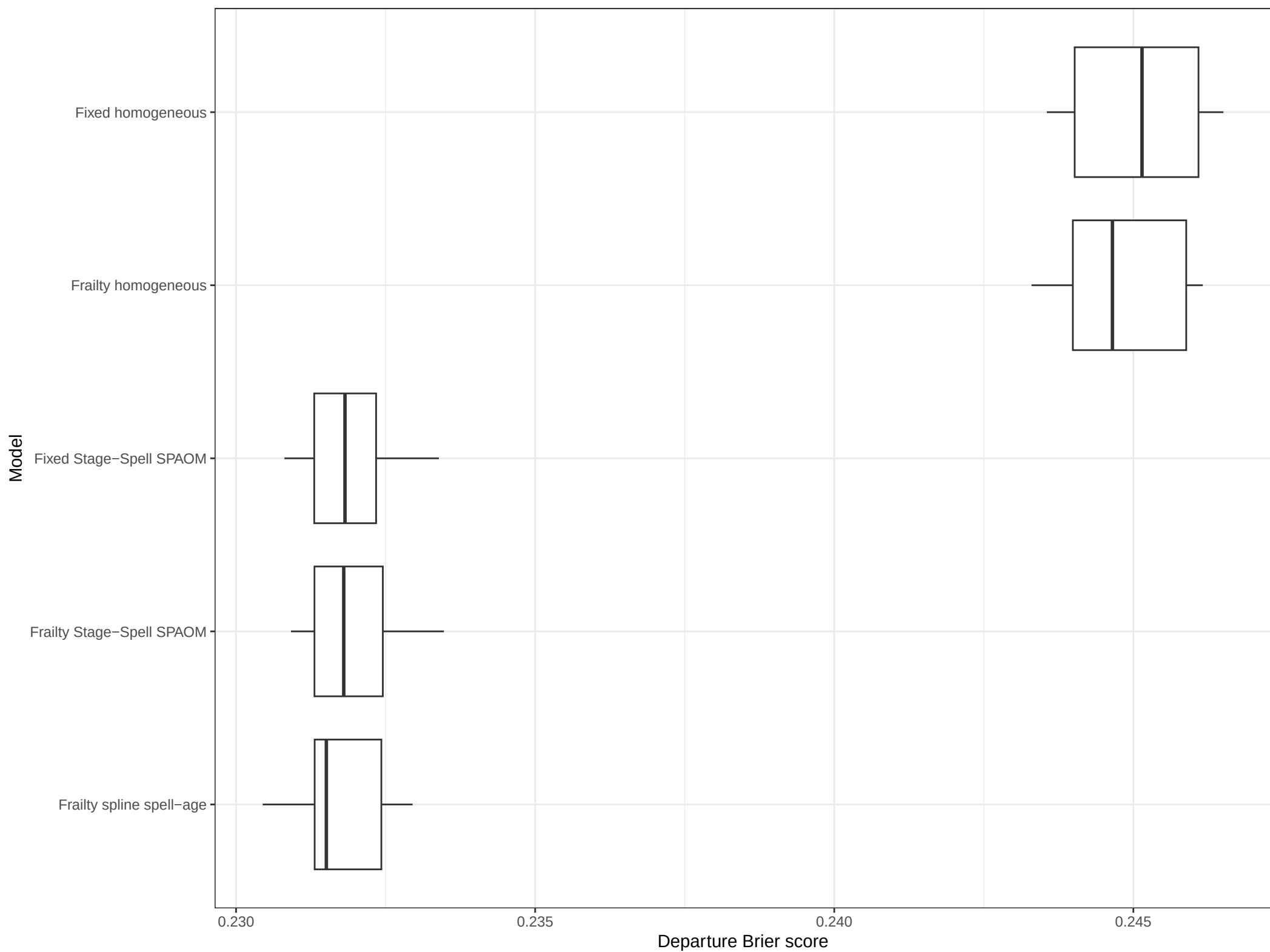
Grouped cross-validated departure Brier score
