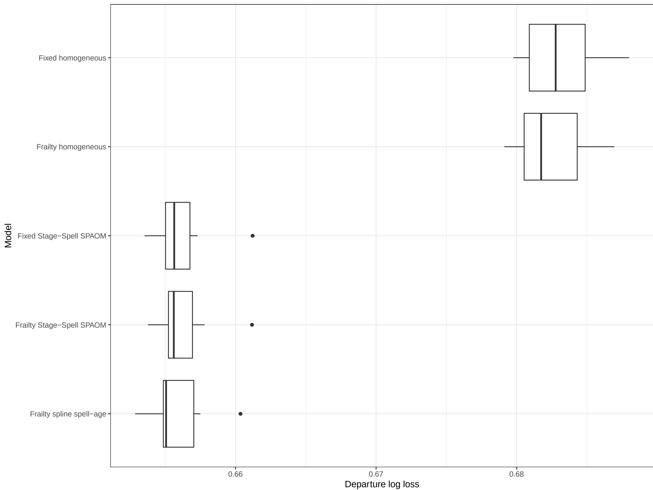
Grouped cross-validated departure log loss
