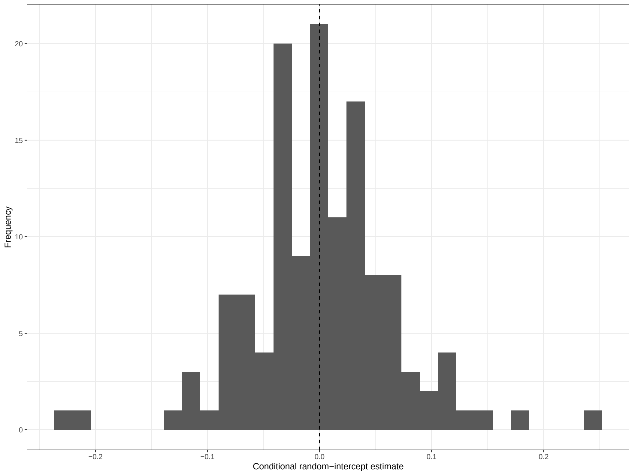
Estimated peace-process random intercepts
