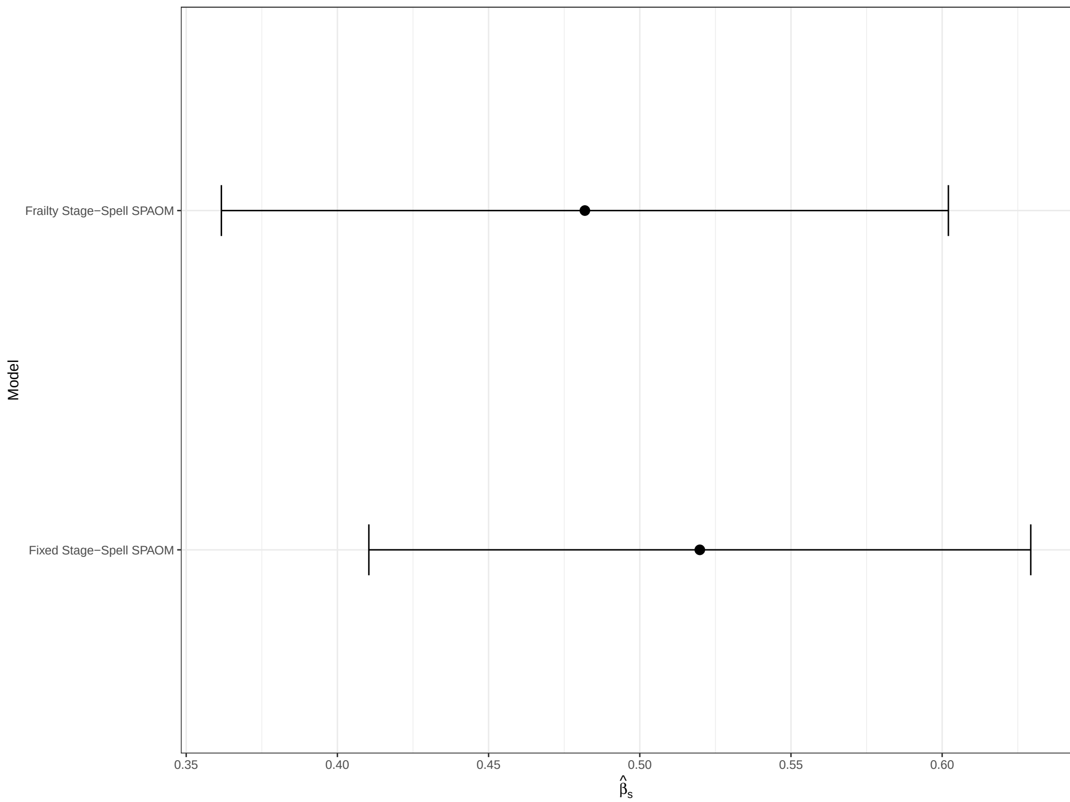
Stage-spell effect before and after process frailty
