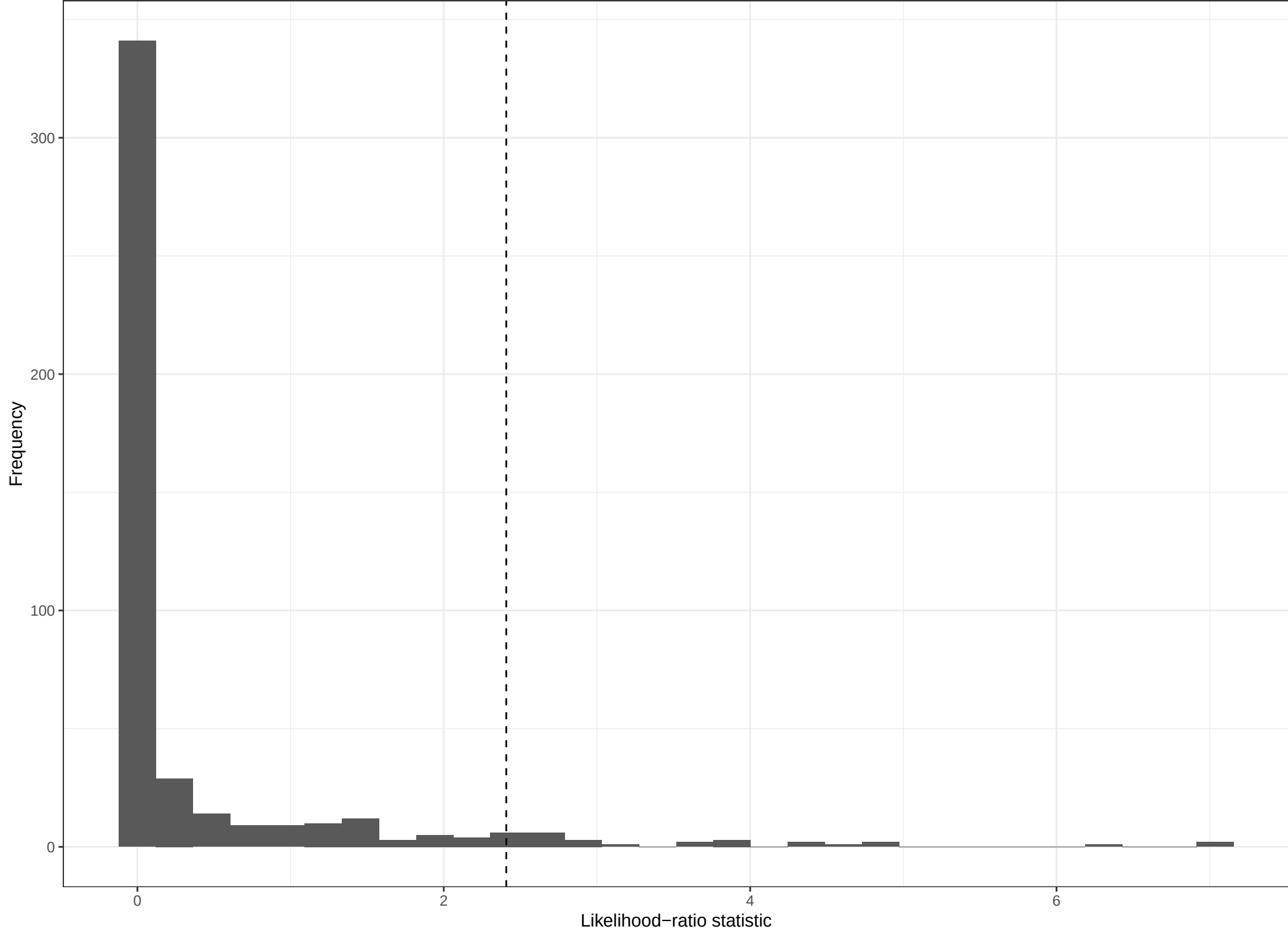
Parametric-bootstrap test of the process-frailty variance Dashed line marks the observed likelihood-ratio statistic
