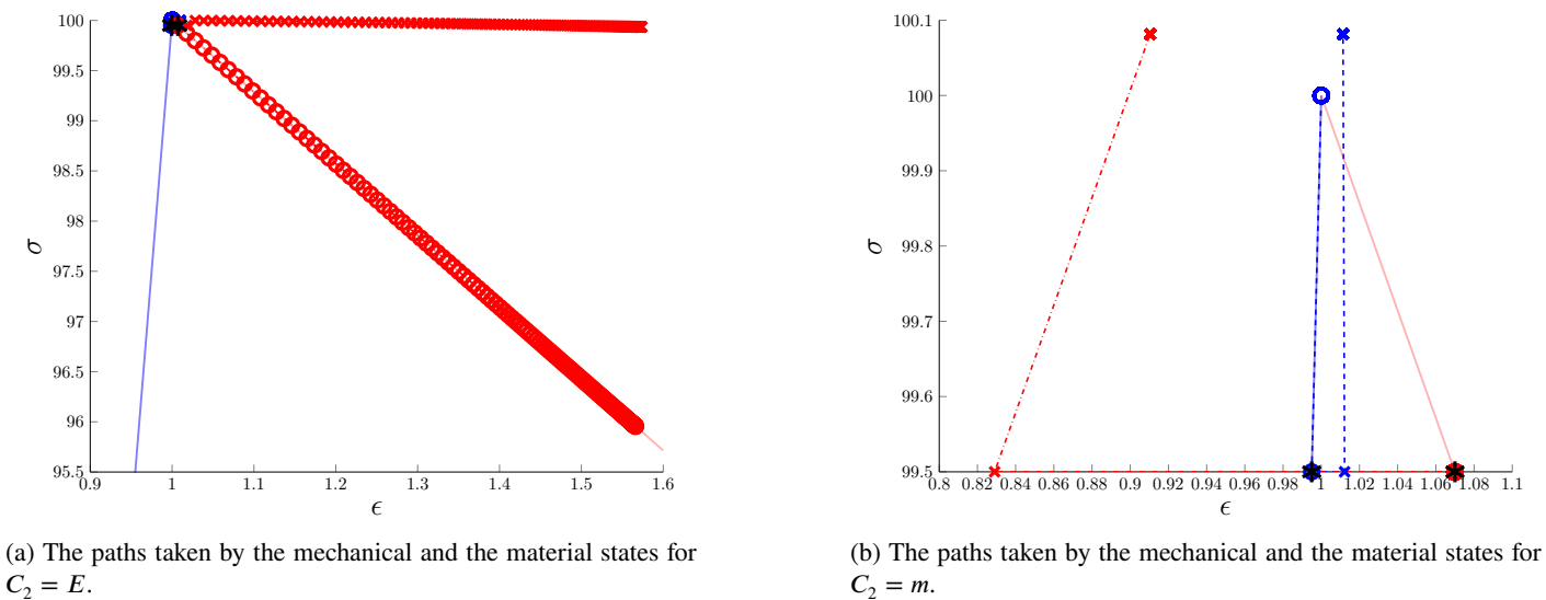
Figure 6: Transition of the mechanical and the material states. Case 3 with snap back, using displacement control.
