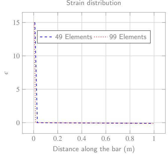
(b) Strain distribution along the bar corresponding to the final load step in the force-displacement response in Figure 8a.
