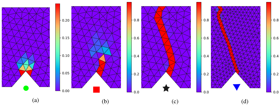
Figure 10: Damage distributions without regularization, each shown at its final converged load step, marked by respective symbols in Figure 9 for the corresponding load-displacement curves. (a) Coarse mesh - Damaged elastic modulus used for hyper-parameter and no AL (scenario 1), (b) Coarse mesh - Tangent modulus used for hyper-parameter and no AL (scenario 2), (c) Coarse mesh - Tangent modulus used for hyper-parameter with AL solver (scenario 3), (d) Fine mesh - Tangent modulus used for hyper-parameter with AL solver (scenario 3).
