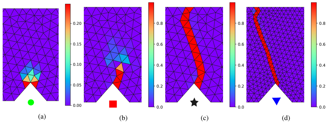
Figure 10: Damage distributions without regularization, each shown at its final converged load step, marked by respective symbols in Figure 9 for the corresponding load-displacement curves. (a) Coarse mesh - Damaged elastic modulus used for hyper-parameter and no AL (scenario 1), (b) Coarse mesh - Tangent modulus used for hyper-parameter and no AL (scenario 2), (c) Coarse mesh - Tangent modulus used for hyper-parameter with AL solver (scenario 3), (d) Fine mesh - Tangent modulus used for hyper-parameter with AL solver (scenario 3).
