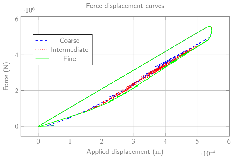
Figure 17: Force displacement curves of the notched bar for three different meshes.
