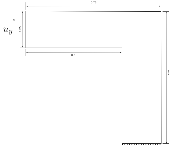
Figure 18: Geometry of the L-beam. All dimensions are in meters.
