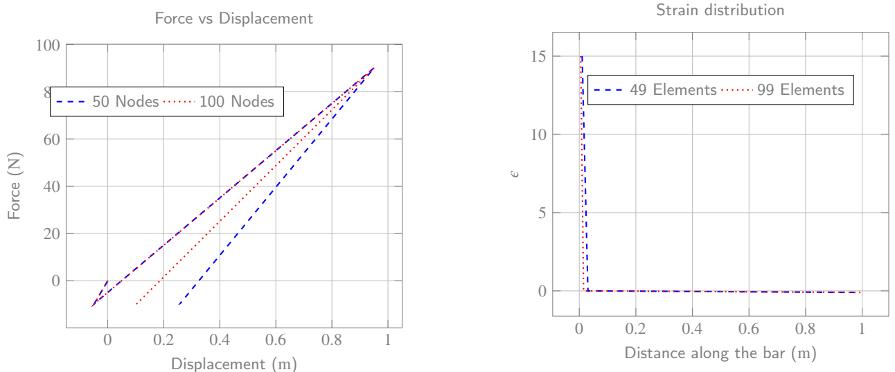
(b) Strain distribution along the bar corresponding to the final load step in the force-displacement response in Figure 8a.
