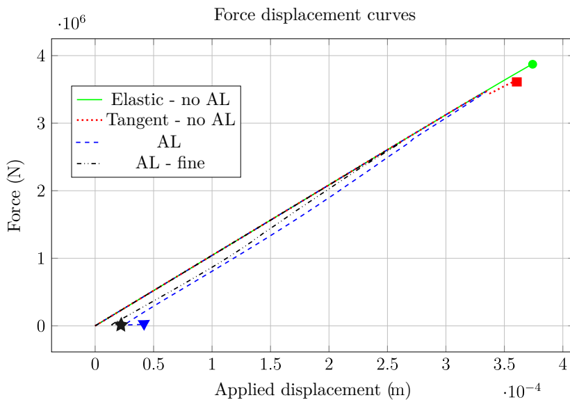
Figure 9: Load - displacement response for the bar with a notch. AL stands for Arc Length. Elastic - no AL corresponds to Figure 10a - scenario 1, Tangent - no AL corresponds to Figure 10b - scenario 2, AL corresponds to Figure 10c - scenario 3, AL - fine corresponds to Figure 10d - scenario 3. The symbols represent the final load-step at which a converged solution is obtained.
