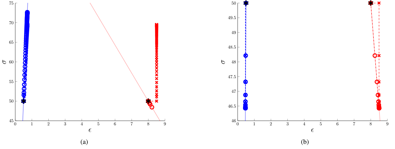
Figure 21: Results from the 1D analysis with a different starting point. Successive mechanical and material states. Snapback and arc-length constraint included. (a) C_2 = g(d)E . (b) C_2 = m .
