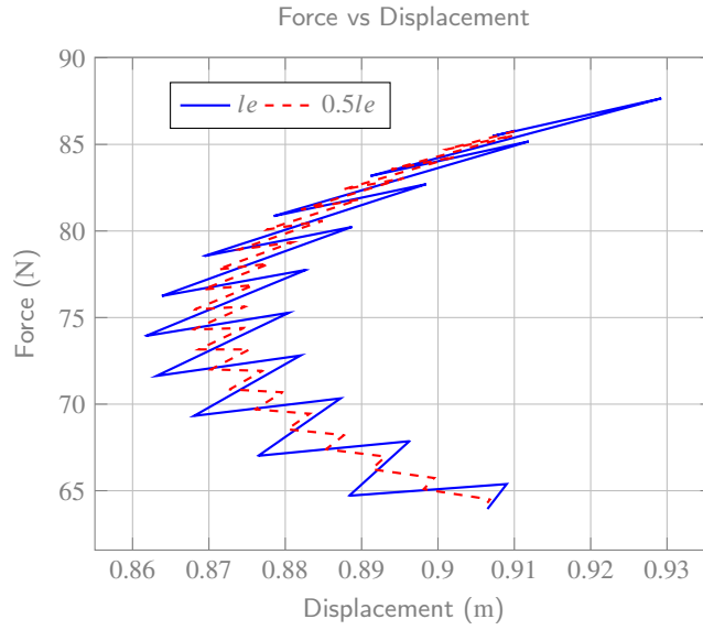
Figure 13: Force vs Displacement curves for two mesh sizes zoomed in.
