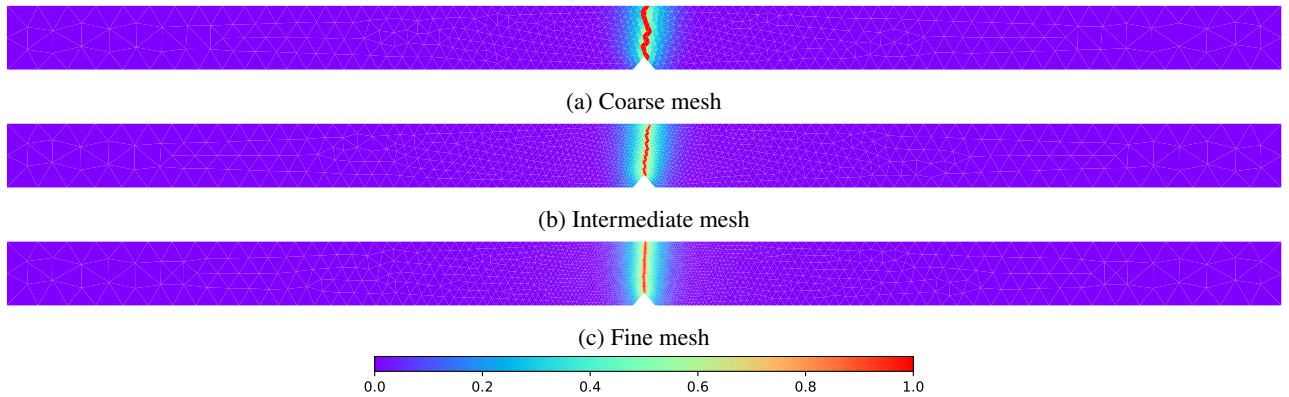
Figure 15: Damage distribution for the notched bar at the final load step, for three mesh sizes
