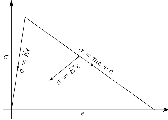
Figure 7: Stress strain database
