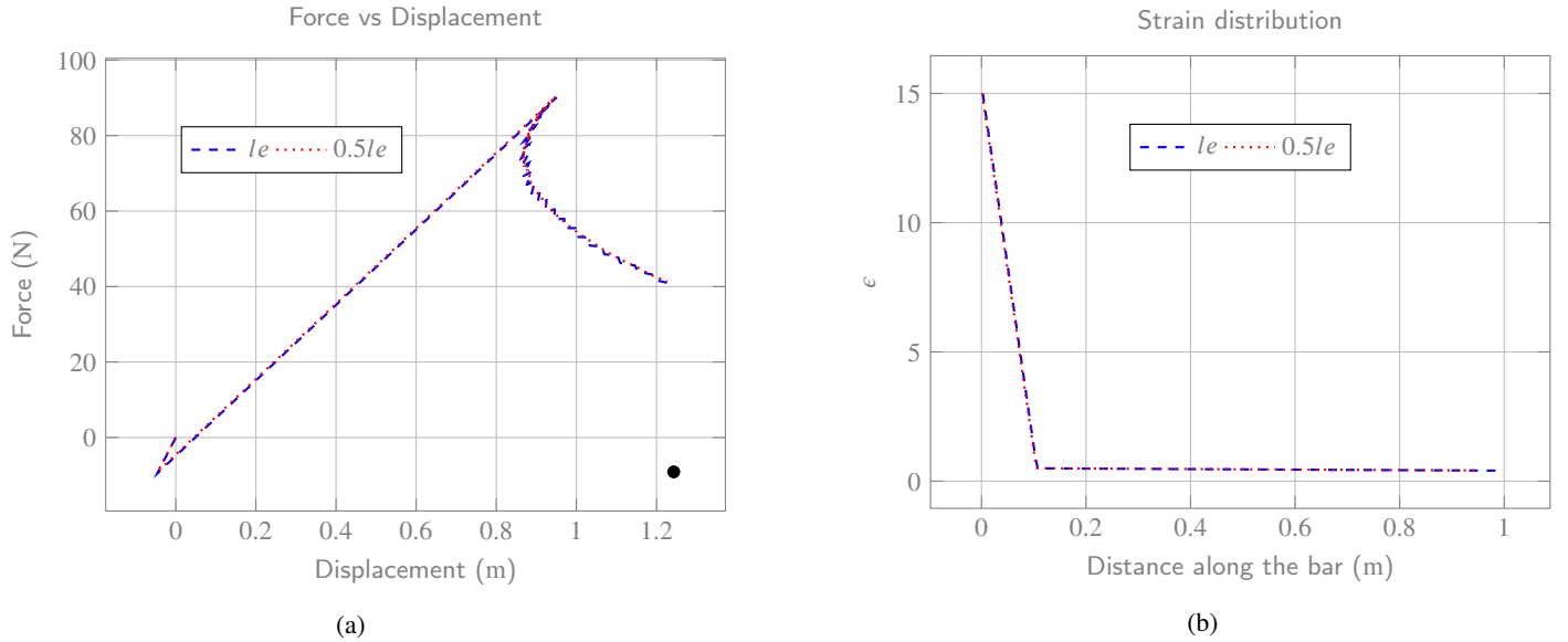
Figure 12: Results with regularization. (a) Force vs Displacement curves for two mesh sizes. (b) Strain distribution along the bar.
