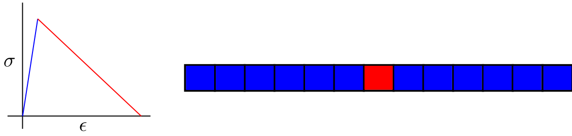
Figure 1: 1D bar with damaged element and the associated elastic (in blue) and damage (in red) branches.
