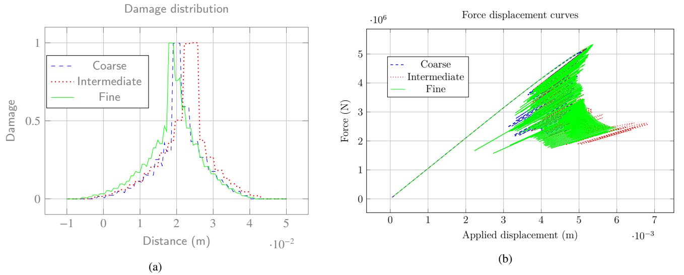
Figure 20: Results for the L beam. (a) Variation of damage along the line x = 0.08 m, y \in [-0.01, 0.05] m. The inner corner of the L-beam is taken as the origin. (b) Force displacement curves for three different meshes.
