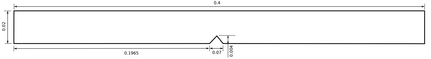
Figure 14: Geometry of the bar with a notch. All dimensions are in meters.
