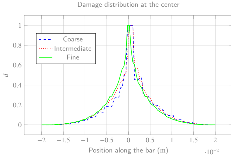
Figure 16: Variation of damage along the center of the bar, y = 0 , x \in [-0.02, 0.02] m.
