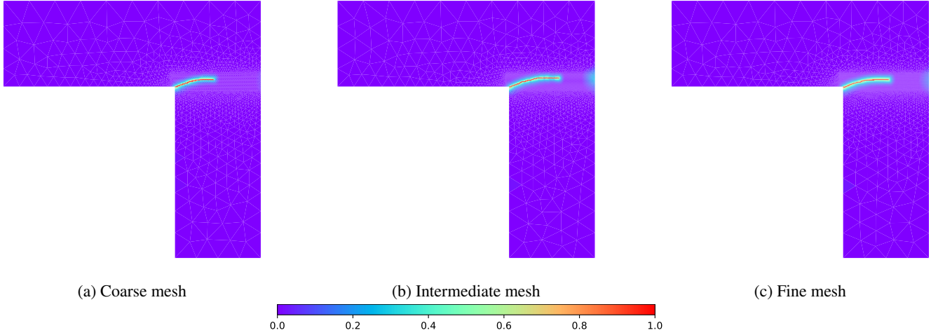
Figure 19: Damage distribution for the L-beam at the final load step, for three mesh sizes
