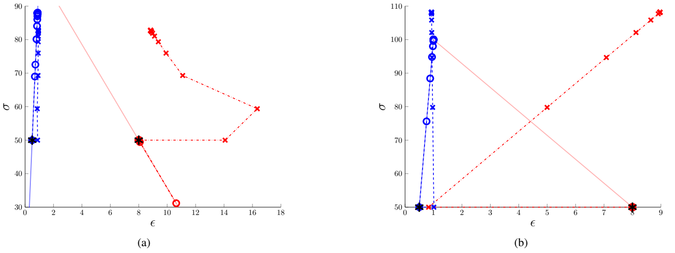
Figure 22: Results from the 1D analysis with a different starting point. Successive mechanical and material states. Displacement control under snapback. (a) C_2 = g(d)E . (b) C_2 = m .
