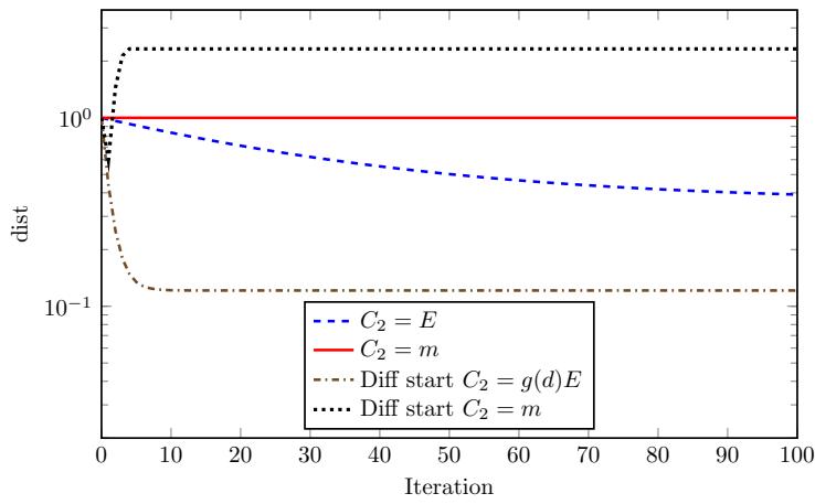
Figure 5: Evolution of the normalized distance functional d_{\text{conv}} under displacement control in the snapback regime ( N = 100 ). Main starting point (near cusp): C_2 = E (dashed blue) stalls near 4 \times 10^{-1} ; C_2 = m (solid red) barely moves from its initial value. Different starting point further down the softening branch (see Appendix B): C_2 = g(d)E (dot-dashed brown) drops and plateaus near 10^{-1} ; C_2 = m (dotted black) diverges and plateaus above 10^0 . All four curves stagnate at finite distances, indicating that the AM iteration fails to reduce the mechanical-material gap under displacement control, independent of the hyper-parameter and the initial state.
