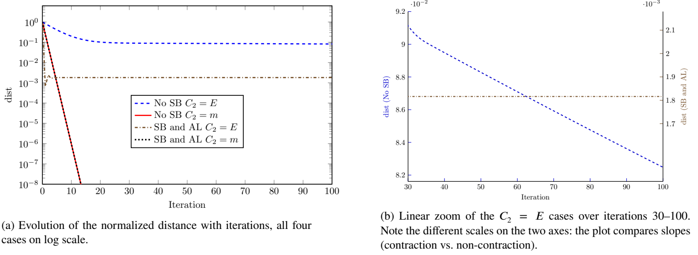
Figure 2: Evolution of the distance functional d_{\text{conv}} (equation 17), normalized by its value at the first iteration, for the four cases studied in Section 3.1. No SB: displacement control with N = 10 (no snapback). SB and AL: arc-length control with N = 100 (snapback regime).
