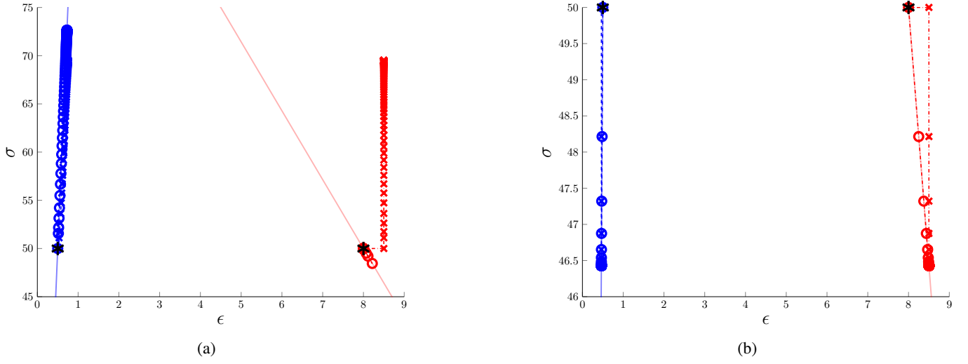
Figure 21: Results from the 1D analysis with a different starting point. Successive mechanical and material states. Snapback and arc-length constraint included. (a) C_2 = g(d)E . (b) C_2 = m .
