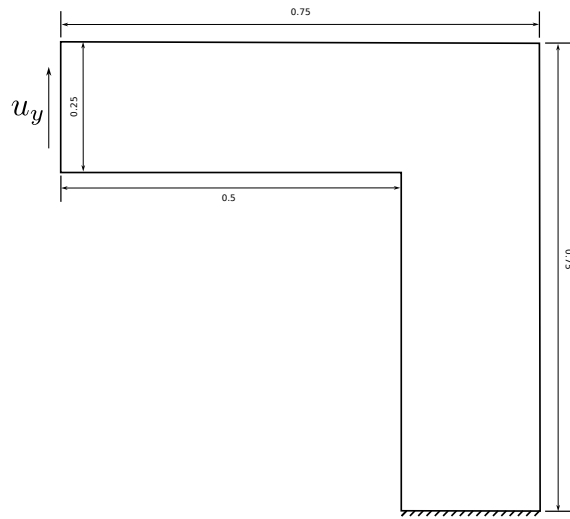
Figure 21: Geometry of the L-beam. All dimensions are in meters.
