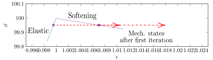
(b) Zoom-in of the first iteration in Figure 7a. Displacement control with C_2 = E .
