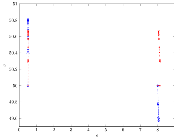
Figure 8: Transition of the mechanical and the material states. Case with snap back, using displacement control, initiated further down the damage branch.
