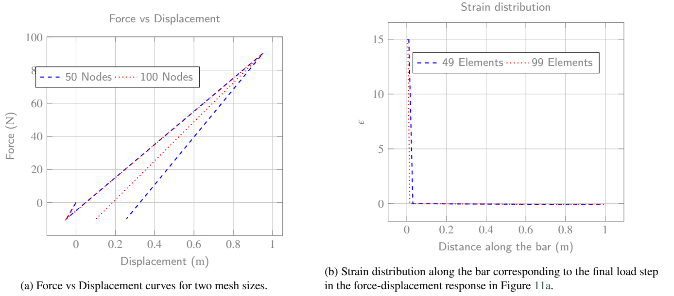
Figure 11: Results for the 1D bar with a body force without regularization.
