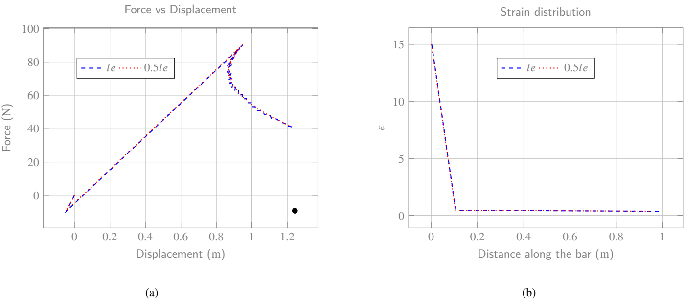
Figure 15: Results with regularization. (a) Force vs Displacement curves for two mesh sizes. (b) Strain distribution along the bar.
