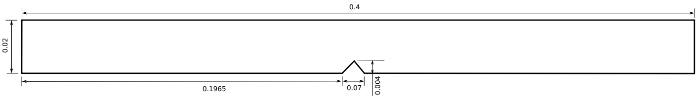
Figure 14: Geometry of the bar with a notch. All dimensions are in meters.
