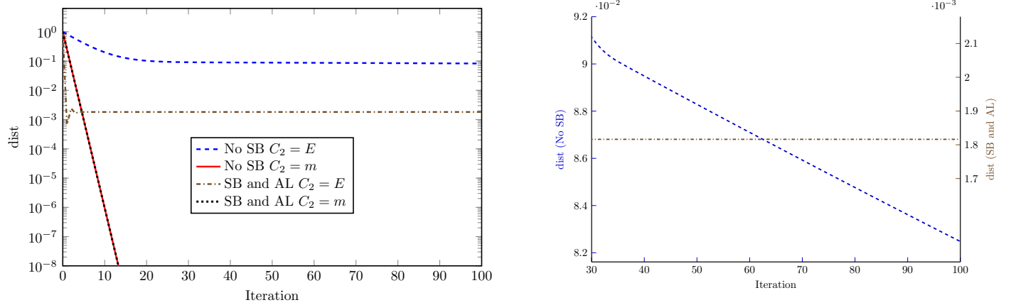
(b) Linear zoom of the C_2 = E cases over iterations 30–100. Note the different scales on the two axes: the plot compares slopes (contraction vs. non-contraction).
