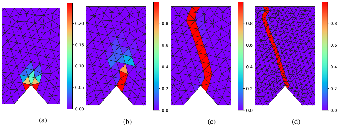
Figure 9: Damage distributions without regularization, each shown at its final converged load step, marked by a solid circle in Figure 10 for the corresponding load-displacement curves. (a) Coarse mesh - Damaged elastic modulus used for hyper-parameter and no AL (scenario 1), (b) Coarse mesh - Tangent modulus used for hyper-parameter and no AL (scenario 2), (c) Coarse mesh - Tangent modulus used for hyper-parameter with AL solver (scenario 3), (d) Fine mesh - Tangent modulus used for hyper-parameter with AL solver (scenario 3).
