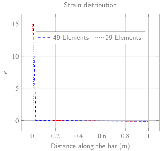
(b) Strain distribution along the bar corresponding to the final load step in the force-displacement response in Figure 8a.
