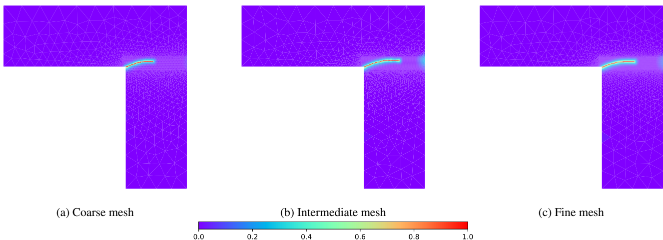
Figure 19: Damage distribution for the L-beam at the final load step, for three mesh sizes
