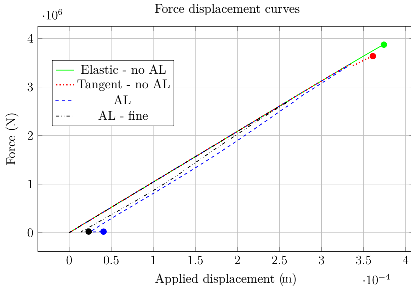
Figure 10: Load - displacement response for the bar with a notch. AL stands for Arc Length. Elastic - no AL corresponds to Figure 9a - scenario 1, Tangent - no AL corresponds to Figure 9b - scenario 2, AL corresponds to Figure 9c - scenario 3, AL - fine corresponds to Figure 9d - scenario 3. Solid circles represent the final load-step at which a converged solution is obtained.
