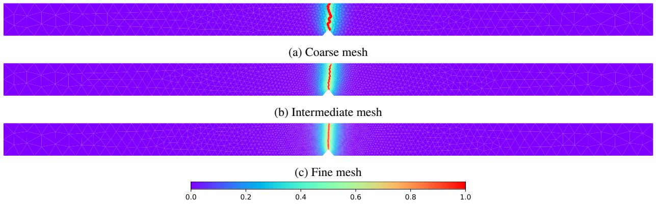
Figure 15: Damage distribution for the notched bar at the final load step, for three mesh sizes
