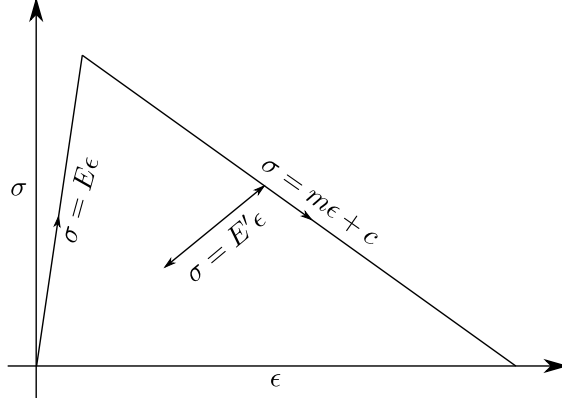
Figure 7: Stress strain database
