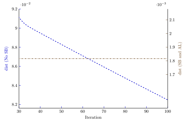
(b) Linear zoom of the C_2 = E cases over iterations 30–100. Note the different scales on the two axes: the plot compares slopes (contraction vs. non-contraction).
