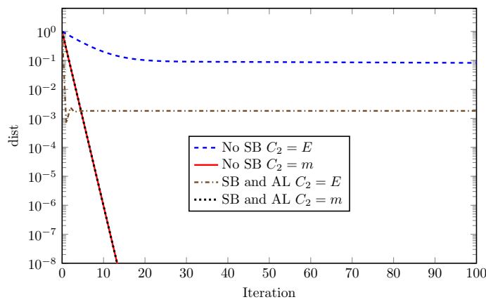
(a) Evolution of the normalized distance with iterations, all four cases on log scale.
