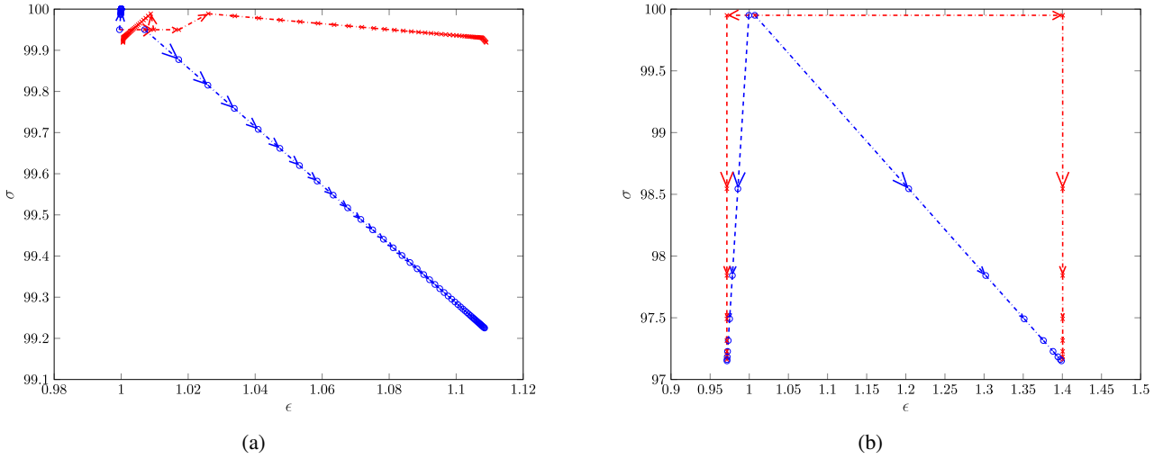
Figure 3: Results from the 1D analysis. Successive mechanical and material states, connected by arrows as indicated in Figure 2. Snapback not expected, and displacement control. (a) C_2 = E . (b) C_2 = m .
