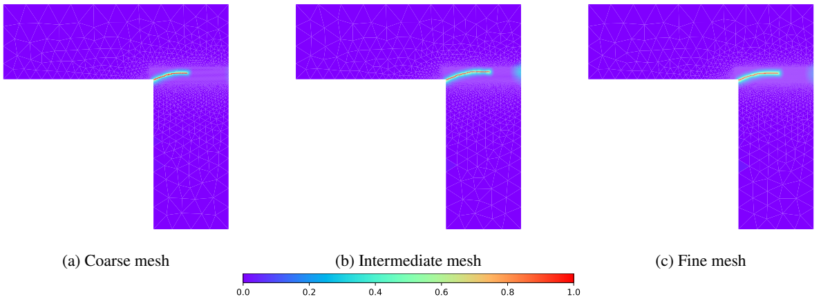
Figure 21: Results of the L beam with regularization
