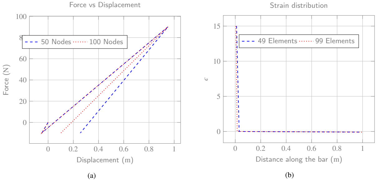
Figure 10: Results without regularization. (a) Force vs Displacement curves for two mesh sizes. (b) Strain distribution along the bar.
