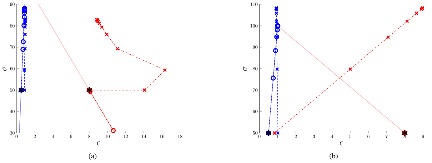
Figure 22: Results from the 1D analysis with a different starting point. Successive mechanical and material states. Displacement control under snapback. (a) C_2 = g(d)E . (b) C_2 = m .
