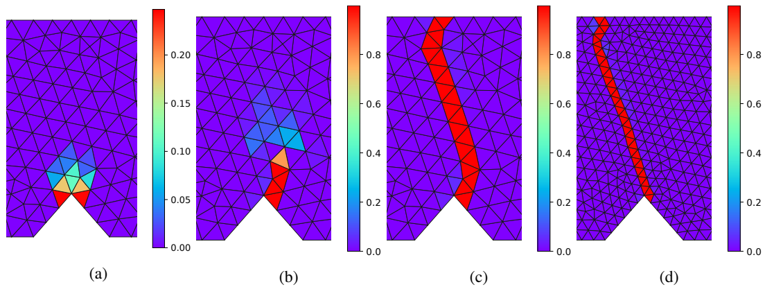
Figure 9: Damage distributions without regularization, each shown at its final converged load step, marked by a solid circle in Figure 10 for the corresponding load-displacement curves. (a) Coarse mesh - Damaged elastic modulus used for hyper-parameter and no AL (scenario 1), (b) Coarse mesh - Tangent modulus used for hyper-parameter and no AL (scenario 2), (c) Coarse mesh - Tangent modulus used for hyper-parameter with AL solver (scenario 3), (d) Fine mesh - Tangent modulus used for hyper-parameter with AL solver (scenario 3).
