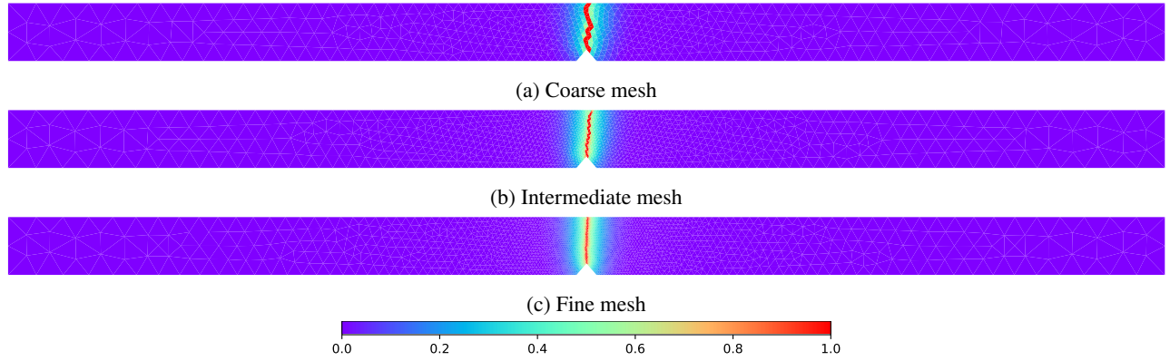
Figure 18: Damage distribution for the notched bar at the final load step, for three mesh sizes
