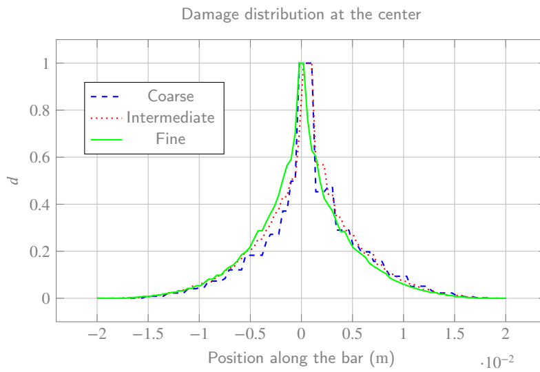
Figure 19: Variation of damage along the center of the bar, y = 0 , x \in [-0.02, 0.02] m.
