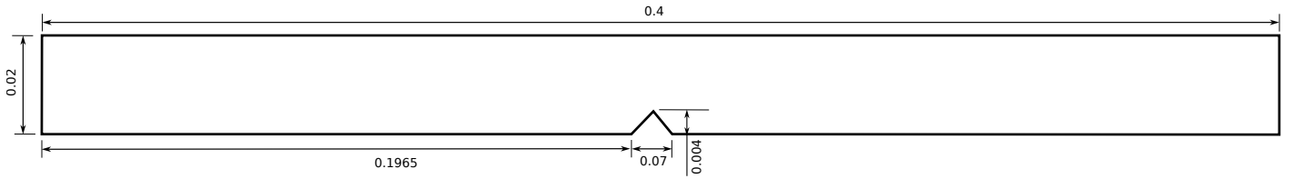
Figure 17: Geometry of the bar with a notch. All dimensions are in meters.
