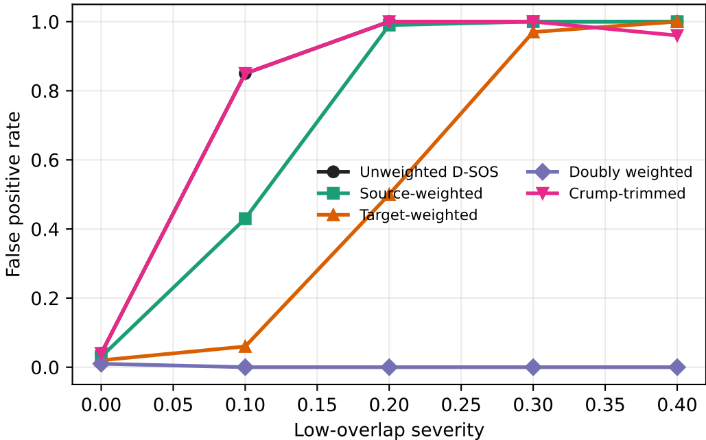
Calibration under support mismatch
