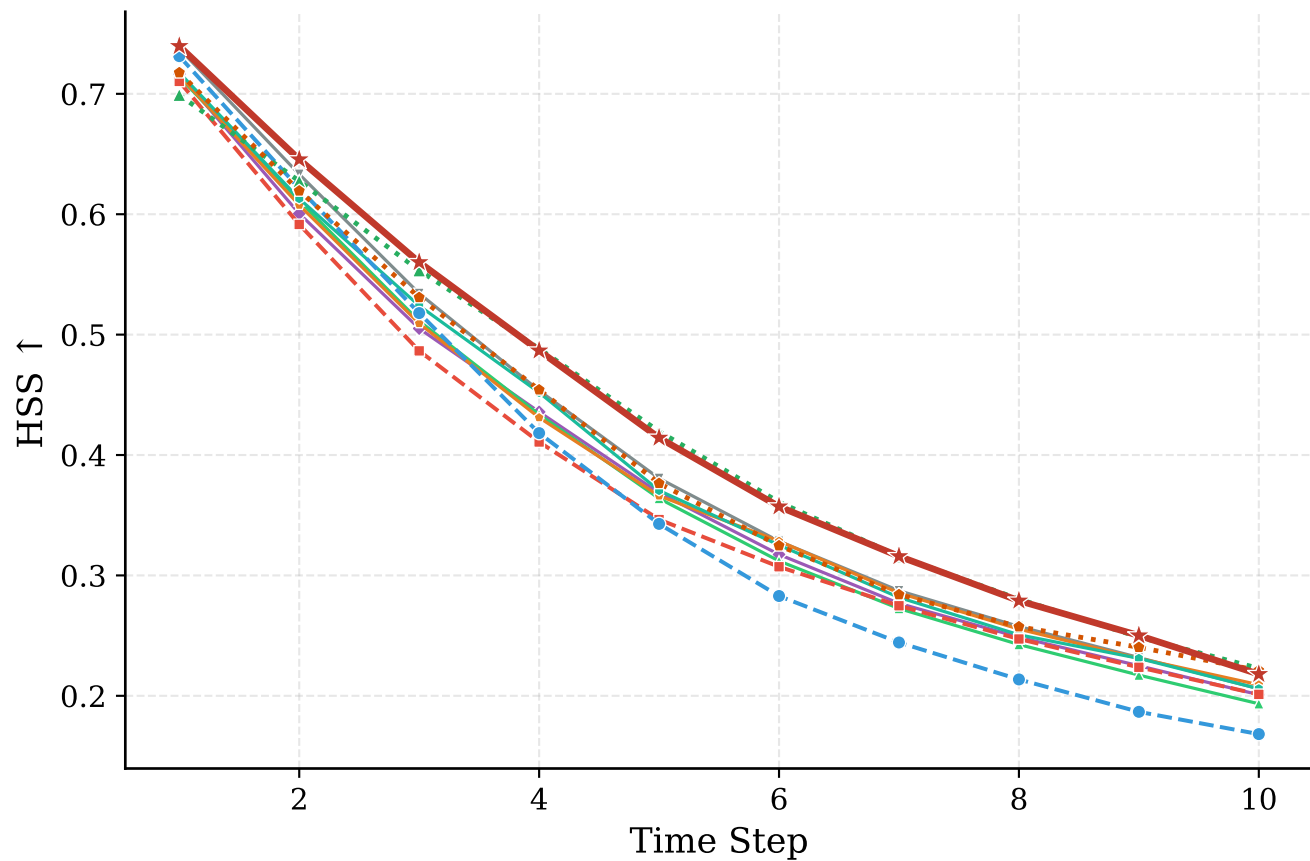
(b) HSS vs Lead Time
