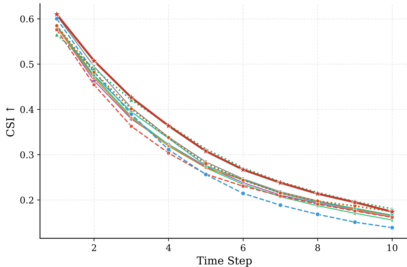
(a) CSI vs Lead Time
