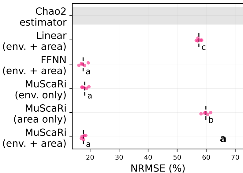
Interpolation performance (spatial block cross evaluation, EVA dataset)
