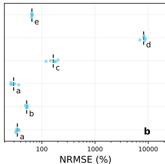
Extrapolation performance (independent evaluation, GIFT dataset)
