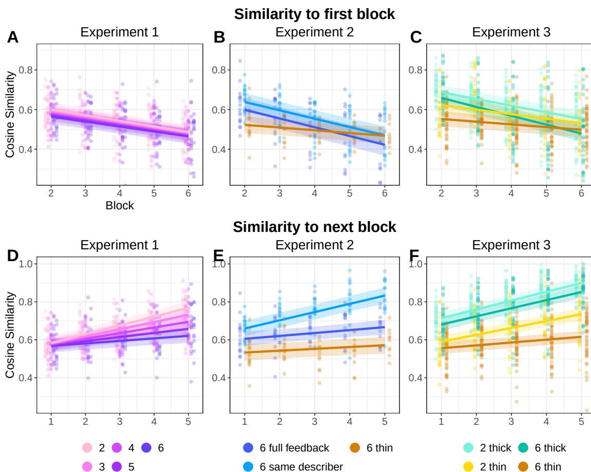
Figure A19: Additional measures of convergence and divergence. A-C is the similarity between utterances on a given block to the first block utterance for the same image, in the same game. Dots are per-game averages, smooths are quadratic. D-F is the similarity between utterances on a given block to the corresponding utterances in the next block. Dots are per-game averages, smooths are quadratic.
