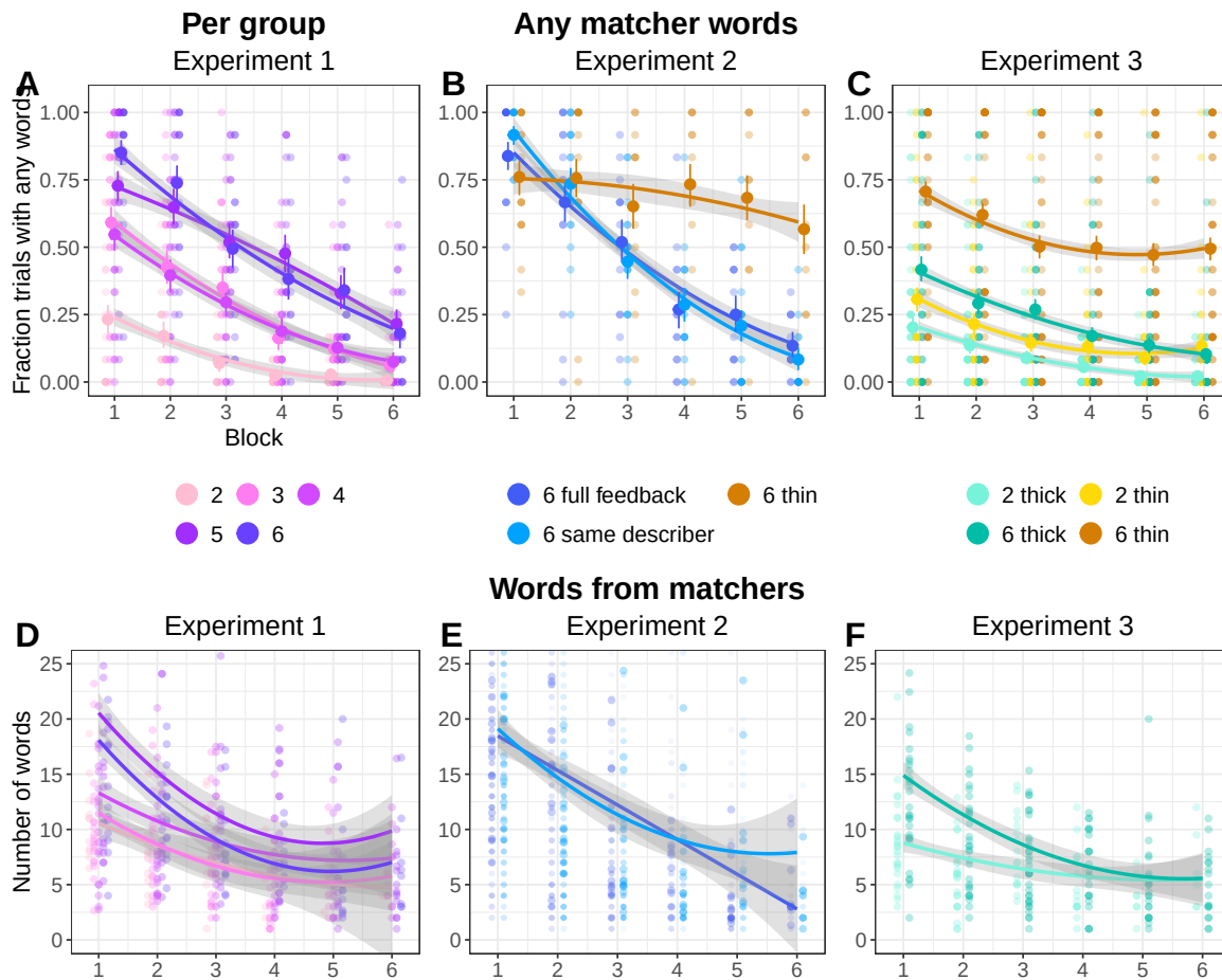
Figure A13: Matcher contributions at the group level. A-C: Fraction of trials where any matcher said anything that was referential. Dots are per game averages. Smooths are binomial fit lines. D-F: On trials where at least one matcher contributed, the number of words of referential language produced by matchers. Dots are per game averages. Smooths are quadratic fit lines. Y-axis is truncated, and a few outliers points are not visible.
