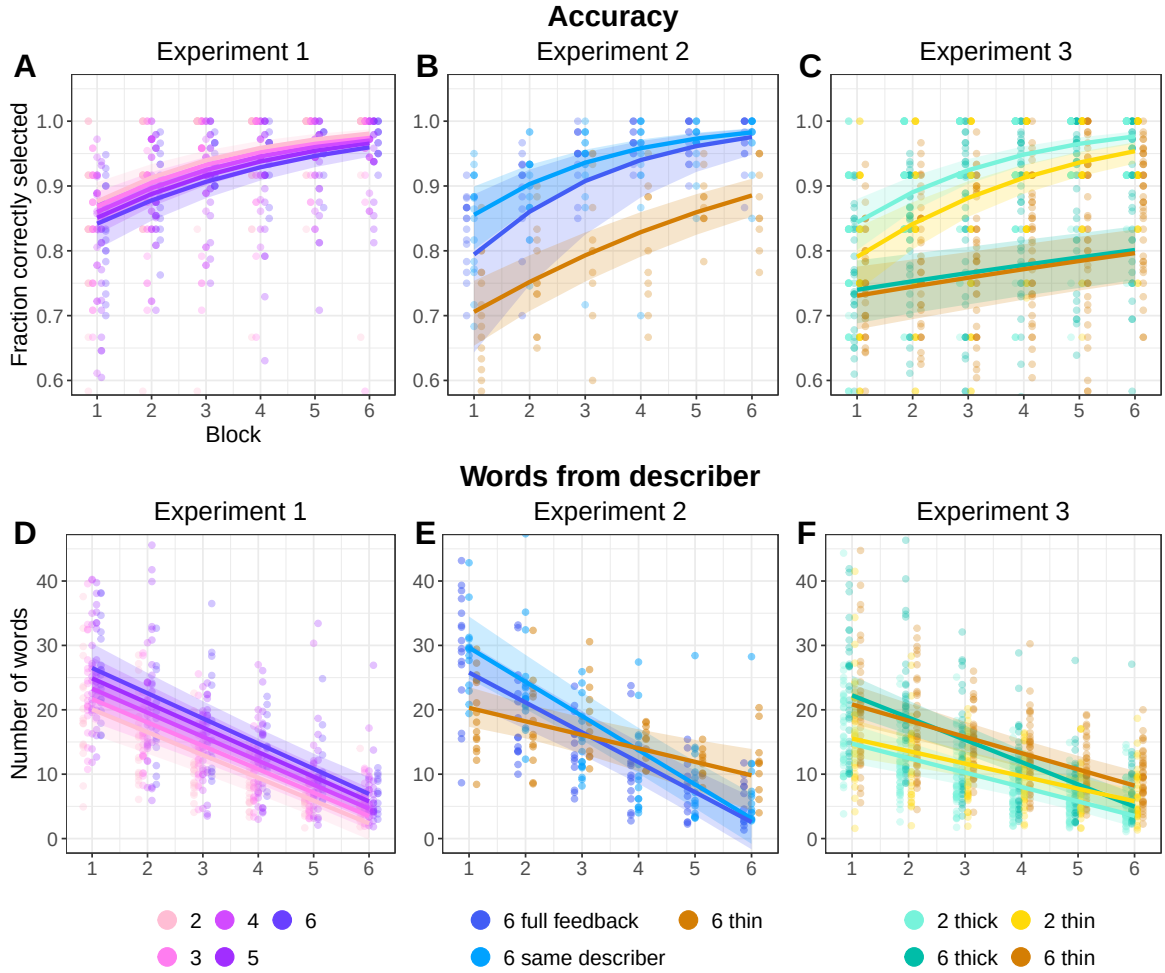
Figure 2.2: Behavioral results across all three experiments. (A-C). Matcher accuracy at selecting the target image. (D-F). Number of words produced by the describer each trial. For all, small dots are per game, per block means, and smooth lines are predictions from model fixed effects with 95% credible intervals. Y-axes are truncated, and a few outliers points are not visible.
