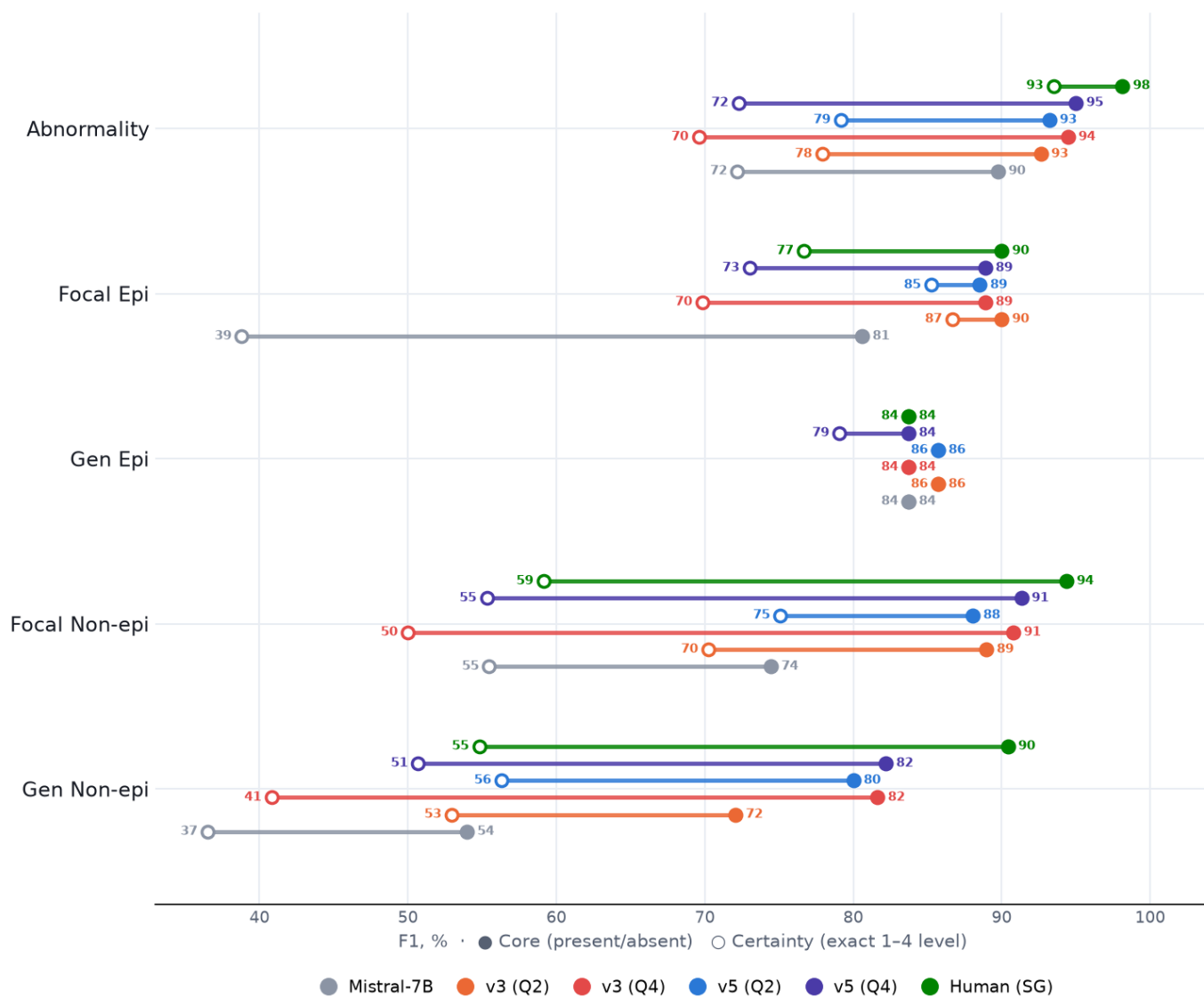
Figure 4: Per-category Core vs Certainty — Maria
