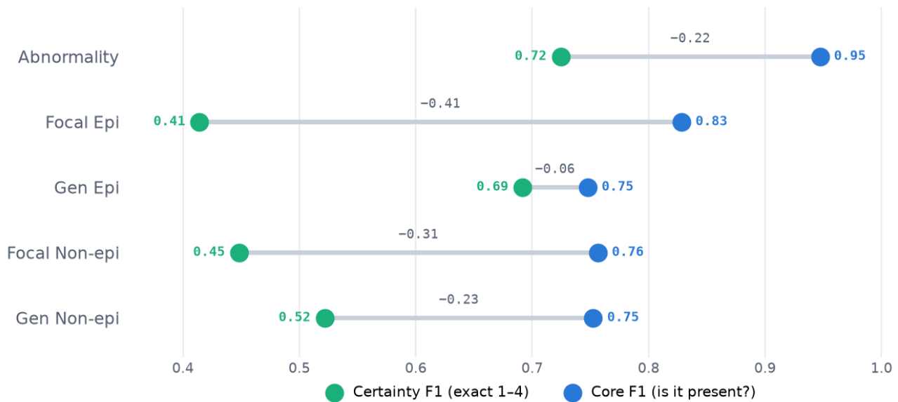
Figure 13: Mistral core vs certainty
