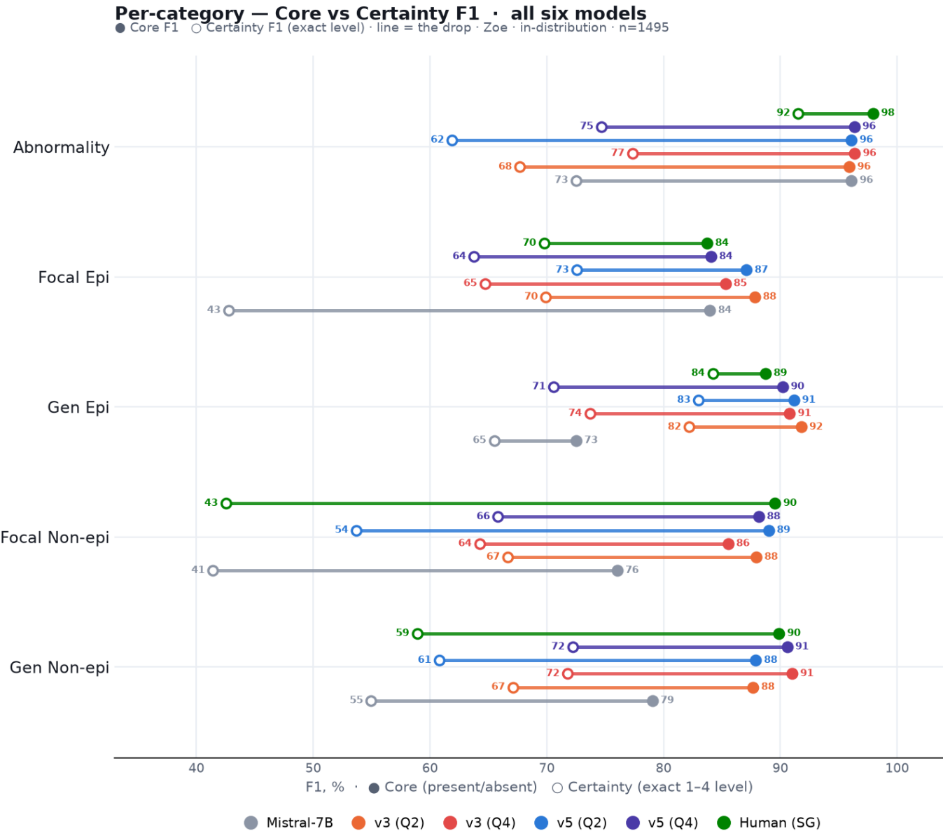
Figure 3: Per-category Core vs Certainty — Zoe
