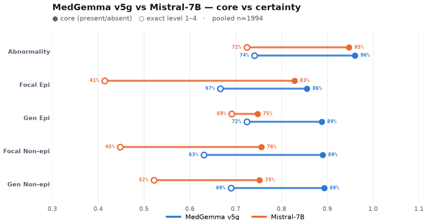
Figure 3: v5g vs Mistral — core vs certainty
