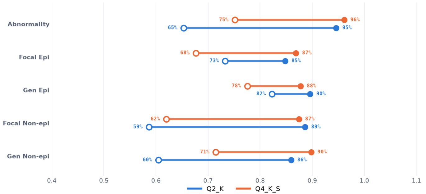
Figure 10: v10g core vs certainty
