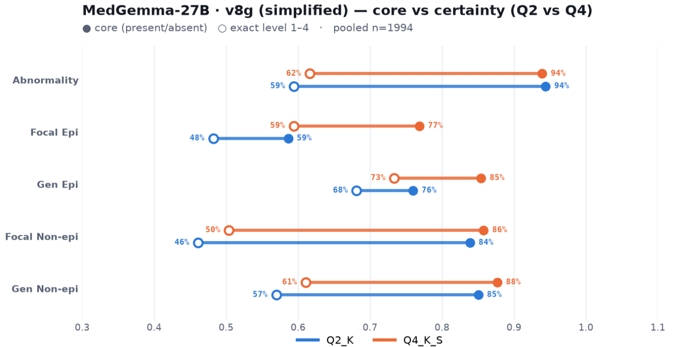
Figure 9: v8g core vs certainty
