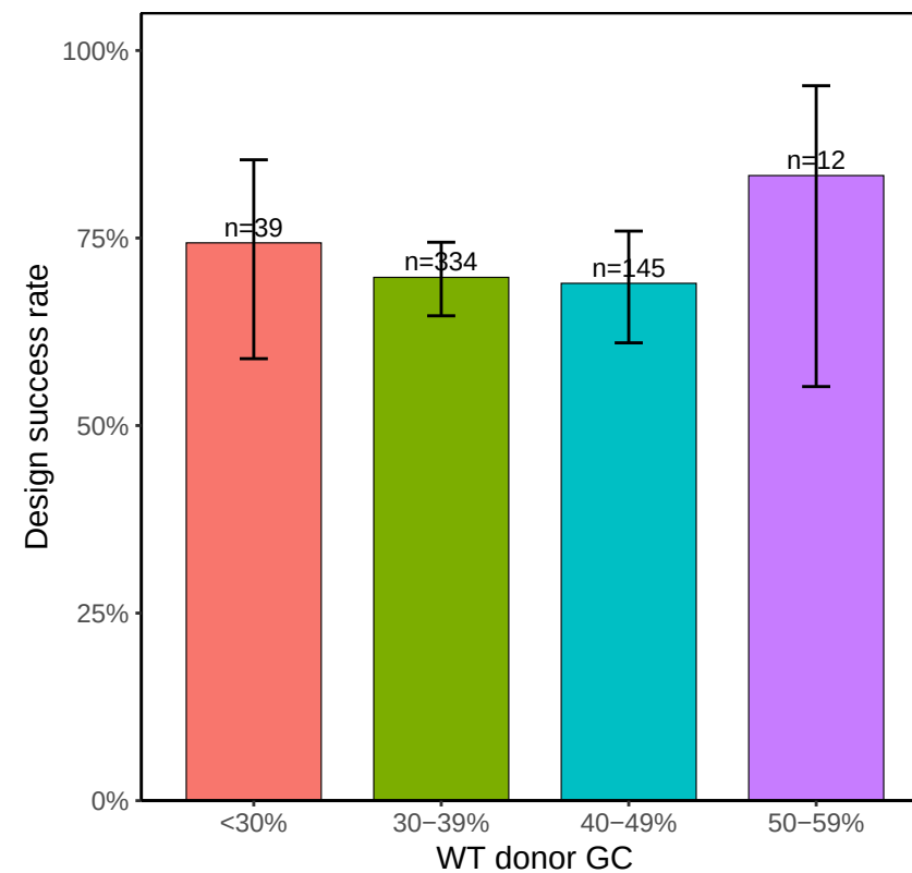
WT donor GC content
