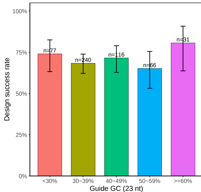
Full spacer GC content
