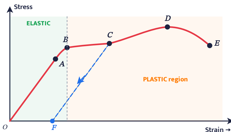
Stress–strain curve of a metal (tensile test). Yield strength \sigma_y at B, ultimate tensile strength \sigma_u at D.
