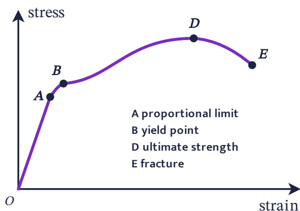
Stress-strain curve of a metal wire
