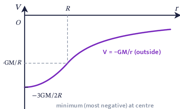
Potential V vs r for a uniform solid sphere
