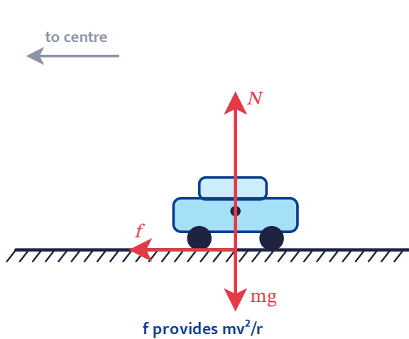
Car on a level road: friction alone
