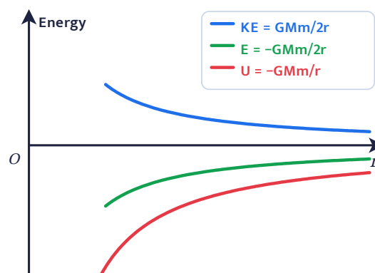
Energies of a satellite vs orbit radius r
