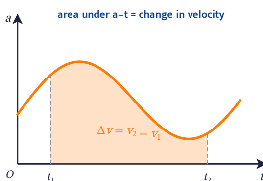
a-t graph: shaded area = \Delta v
