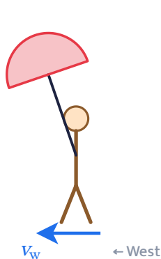
Umbrella tilted forward, along the relative velocity of rain
