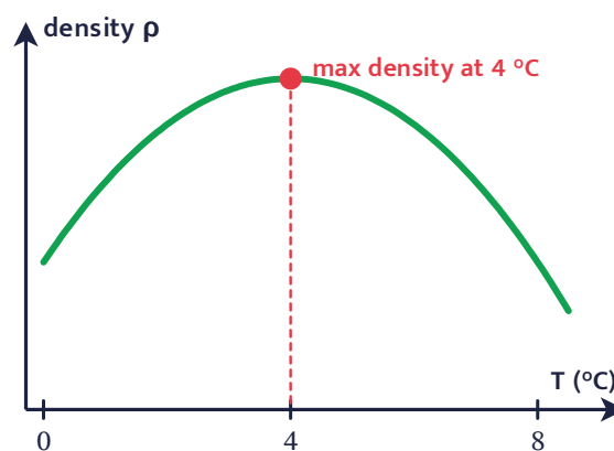
Density of water vs temperature
