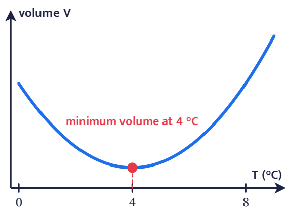
Volume of water vs temperature
