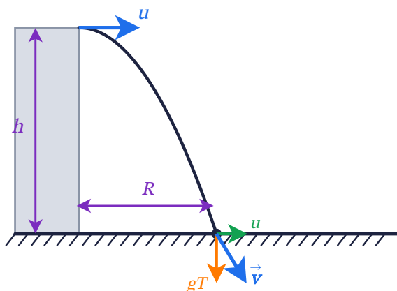
Horizontal projection from a cliff
