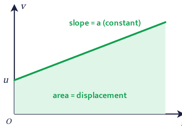
v-t , uniform acceleration: straight line
