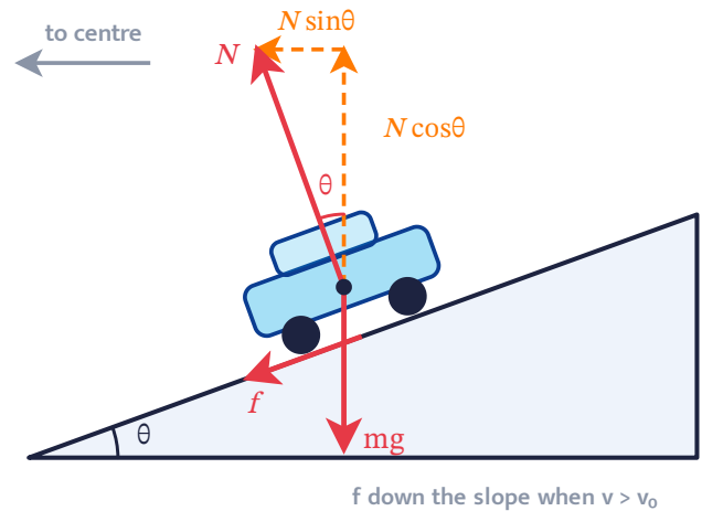
Banked road: N \sin \theta (+ f \cos \theta) gives mv^2/r
