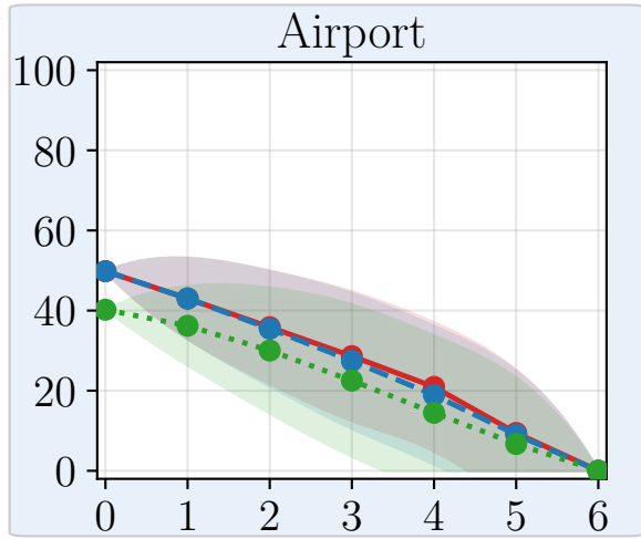
Dependency Leakage (%)
