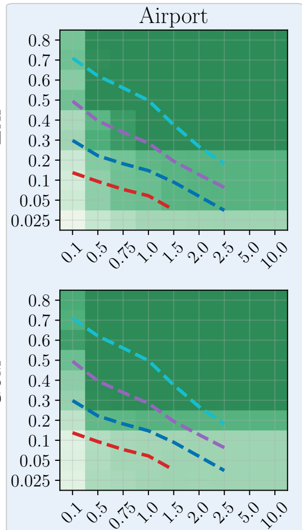
Dependency Leakage Threshold L_0
