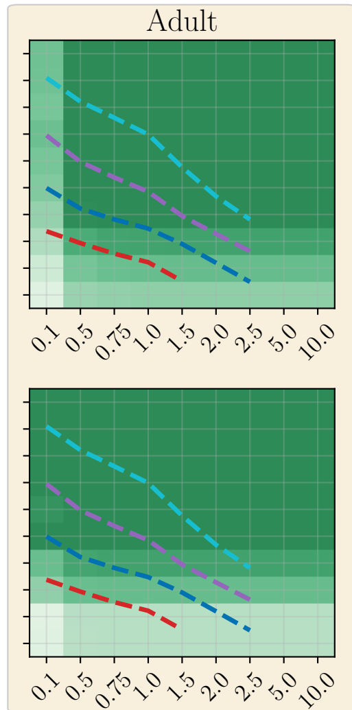
Mask-Pattern Privacy Budget \epsilon_m
