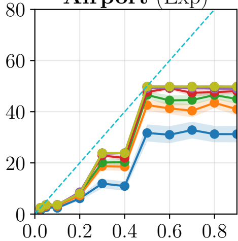
Achieved Re-inference Leakage (%)
