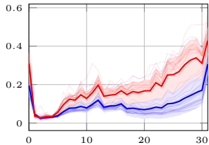
HFER (High Freq Energy Ratio)
