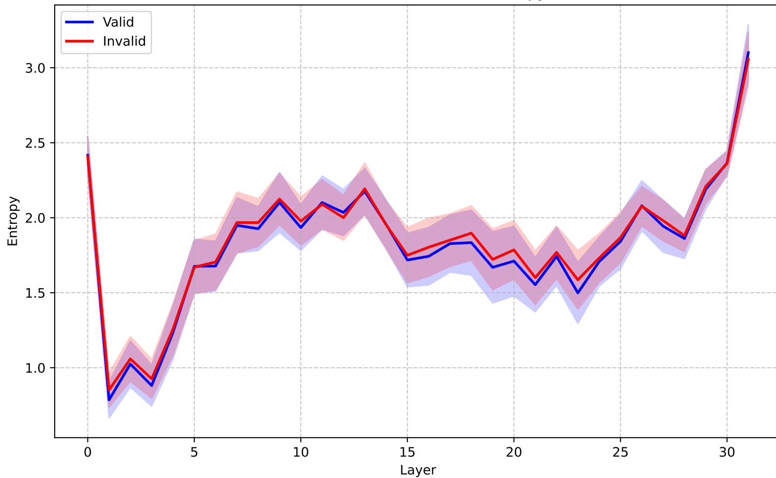
Llama-3.1-8B (Finance) - Entropy
