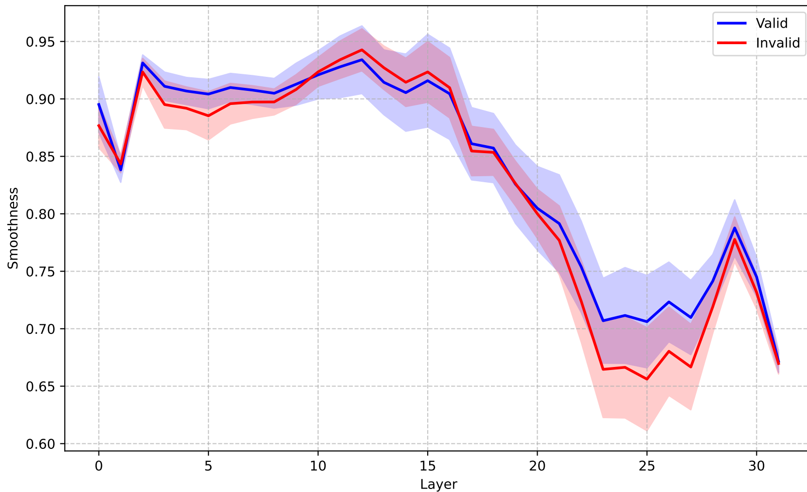
Mistral-7B (General) - Smoothness
