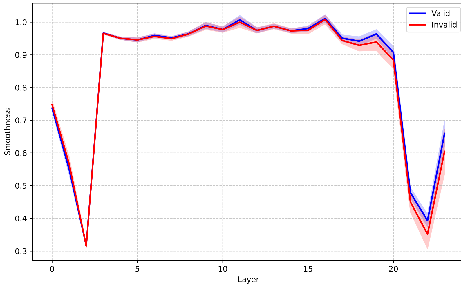
Qwen-2.5-7B (General, T=0.7) - Smoothness
