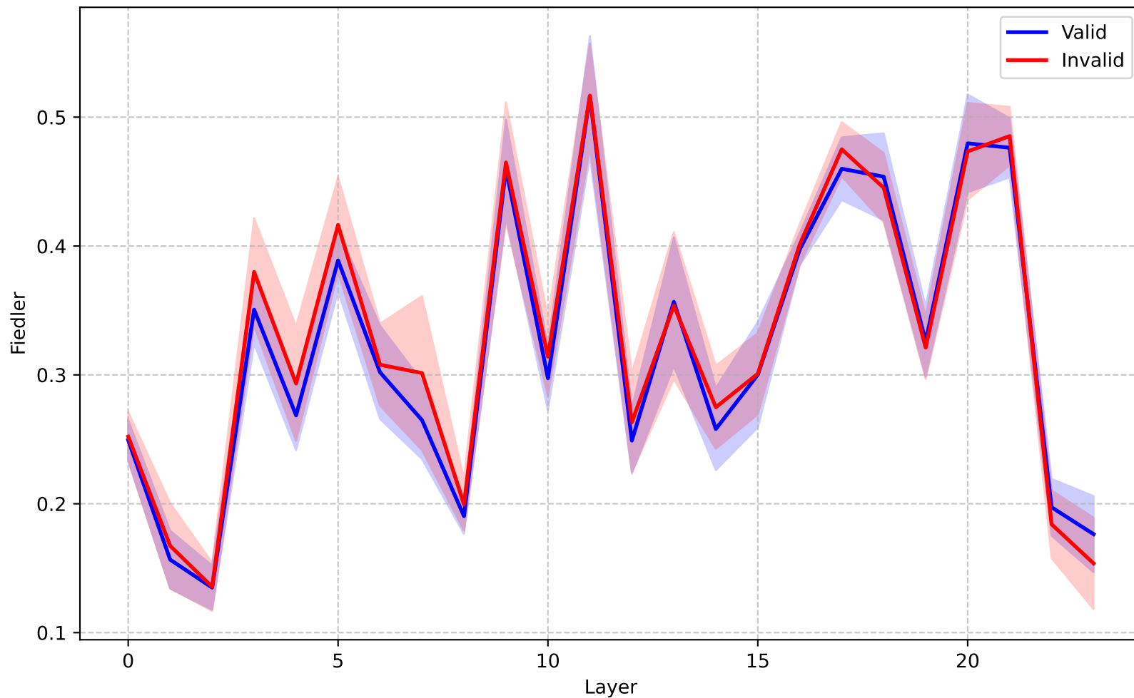
Qwen-2.5-7B (General, T=0.7) - Fiedler
