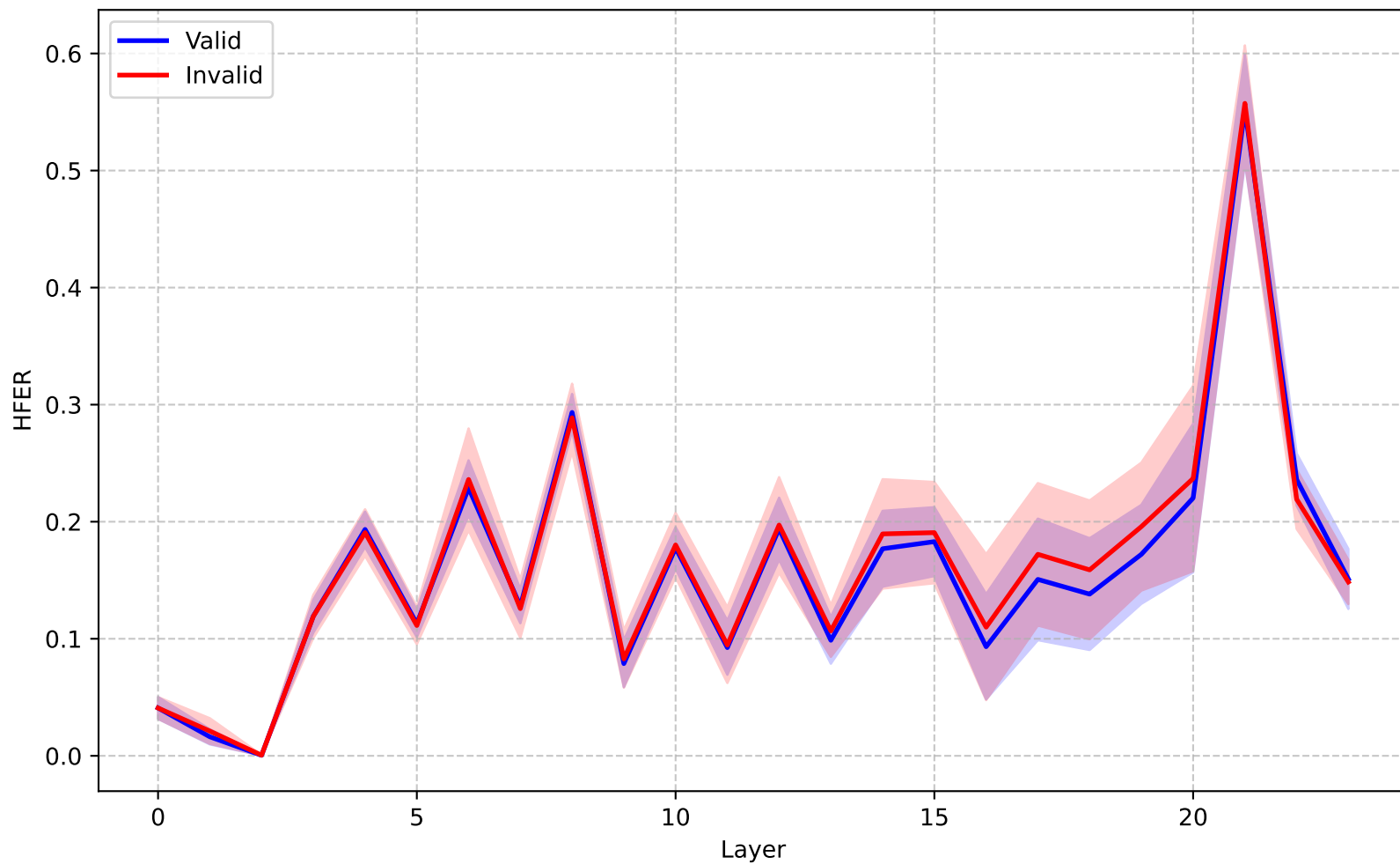
Qwen-2.5-7B (General, T=1.0) - HFER
