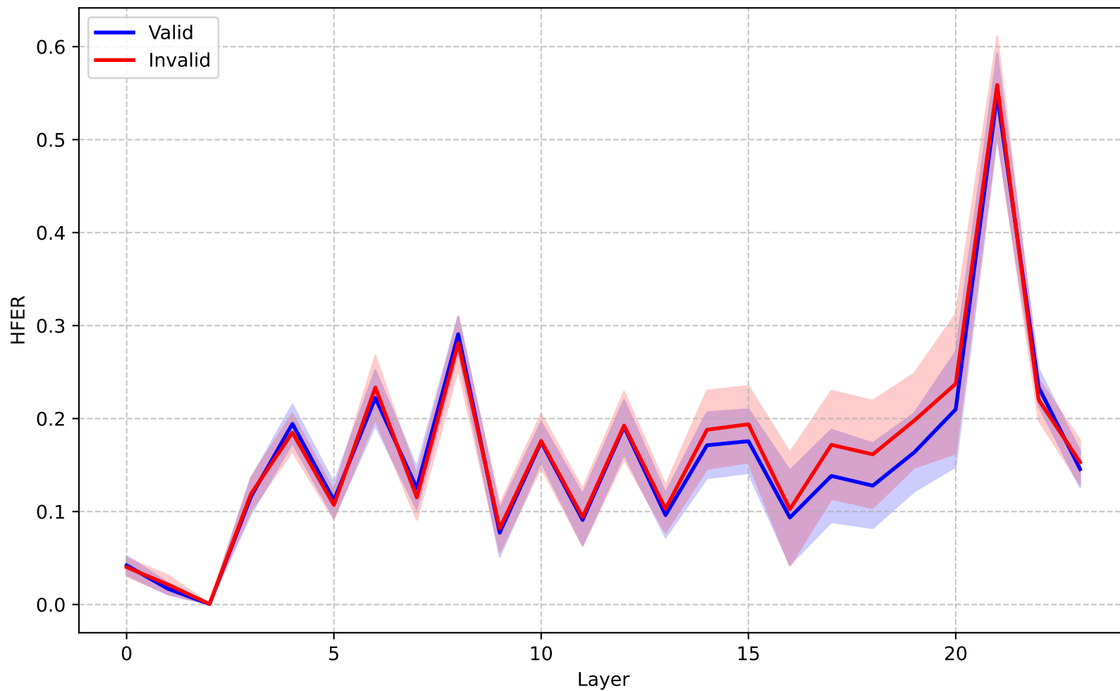
Qwen-2.5-7B (General) - HFER
