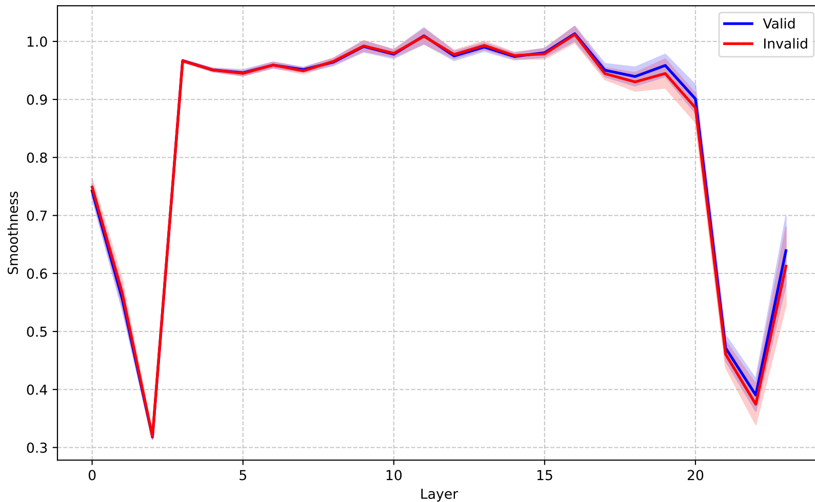
Qwen-2.5-7B (General, T=1.5) - Smoothness
