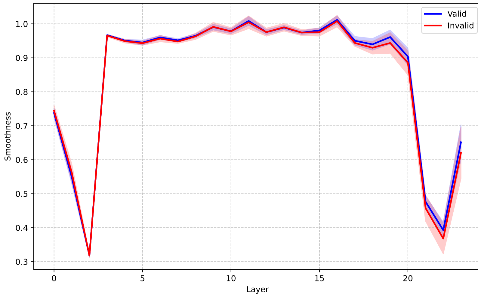
Qwen-2.5-7B (General, T=1.0) - Smoothness
