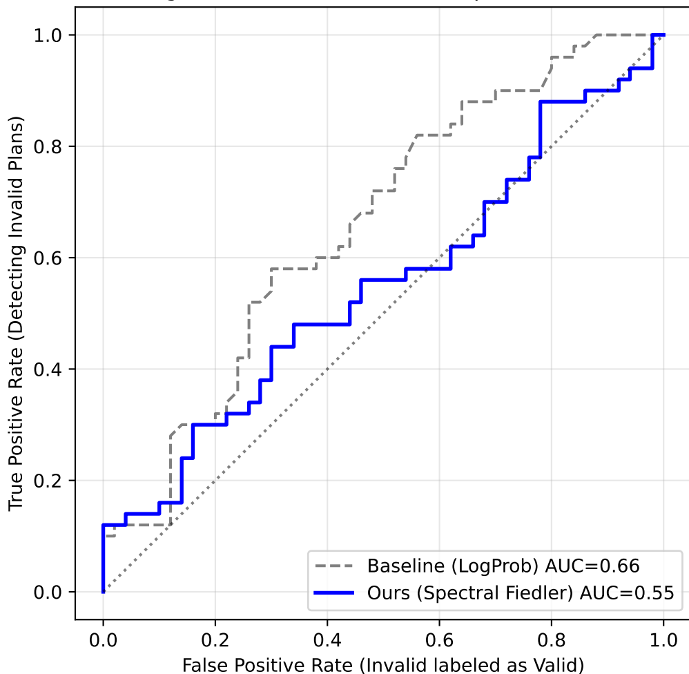
Planning Hallucination Detection: Spectral vs Baseline
