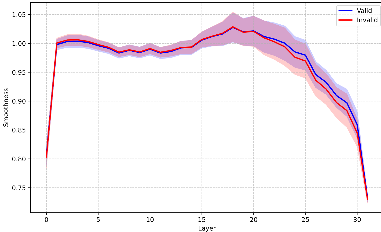
Llama-3.1-8B (Finance) - Smoothness
