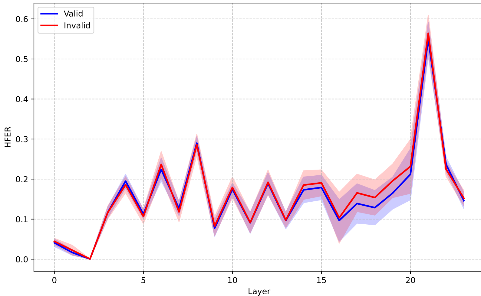
Qwen-2.5-7B (General, T=0.7) - HFER
