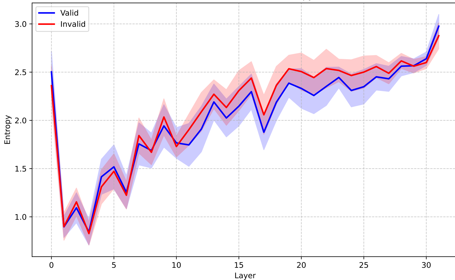
Mistral-7B (General) - Entropy
