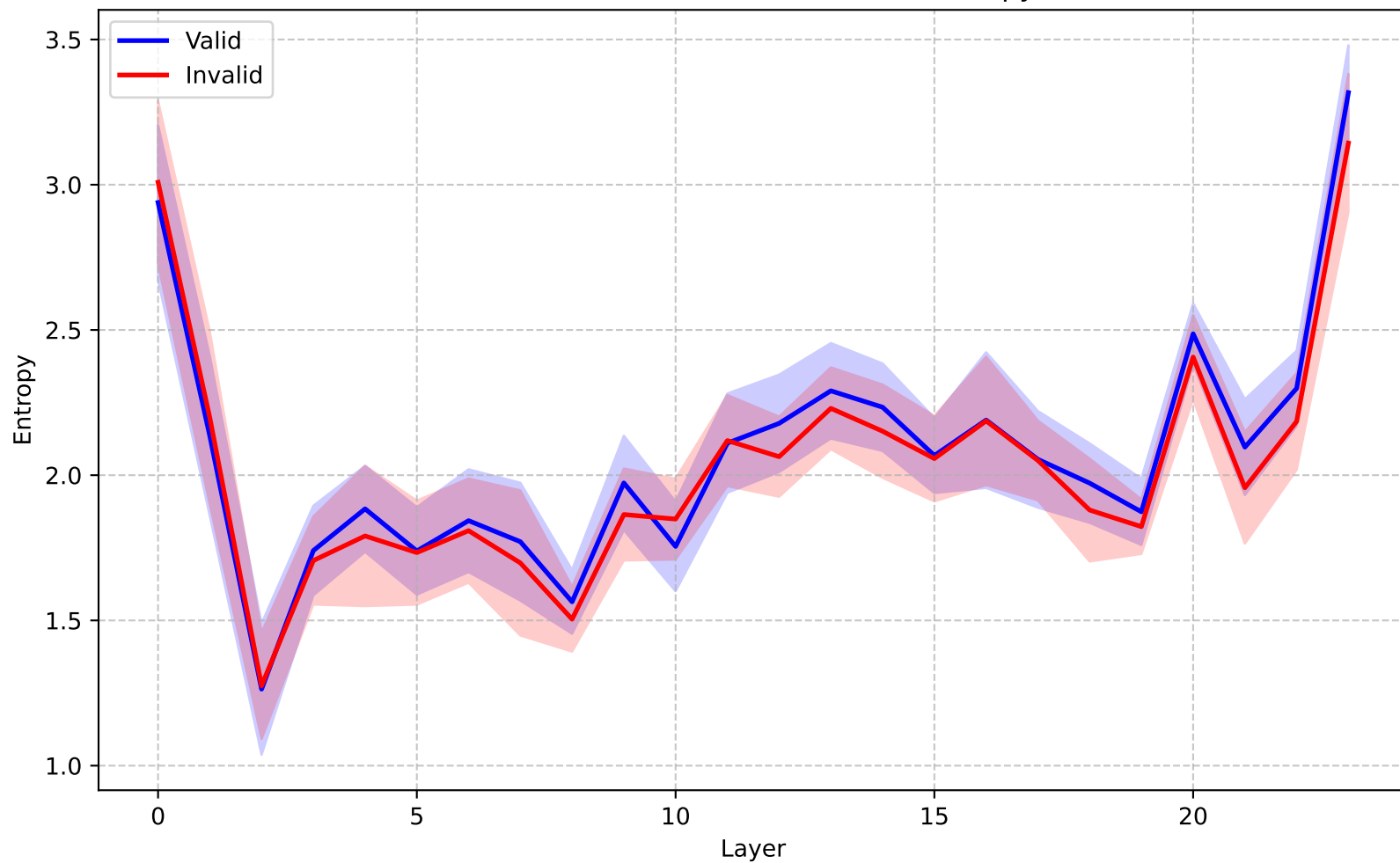
Qwen-2.5-7B (General, T=0.7) - Entropy
