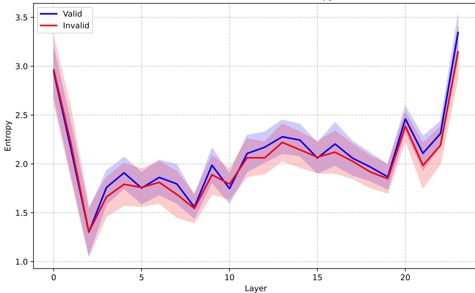
Qwen-2.5-7B (General) - Entropy
