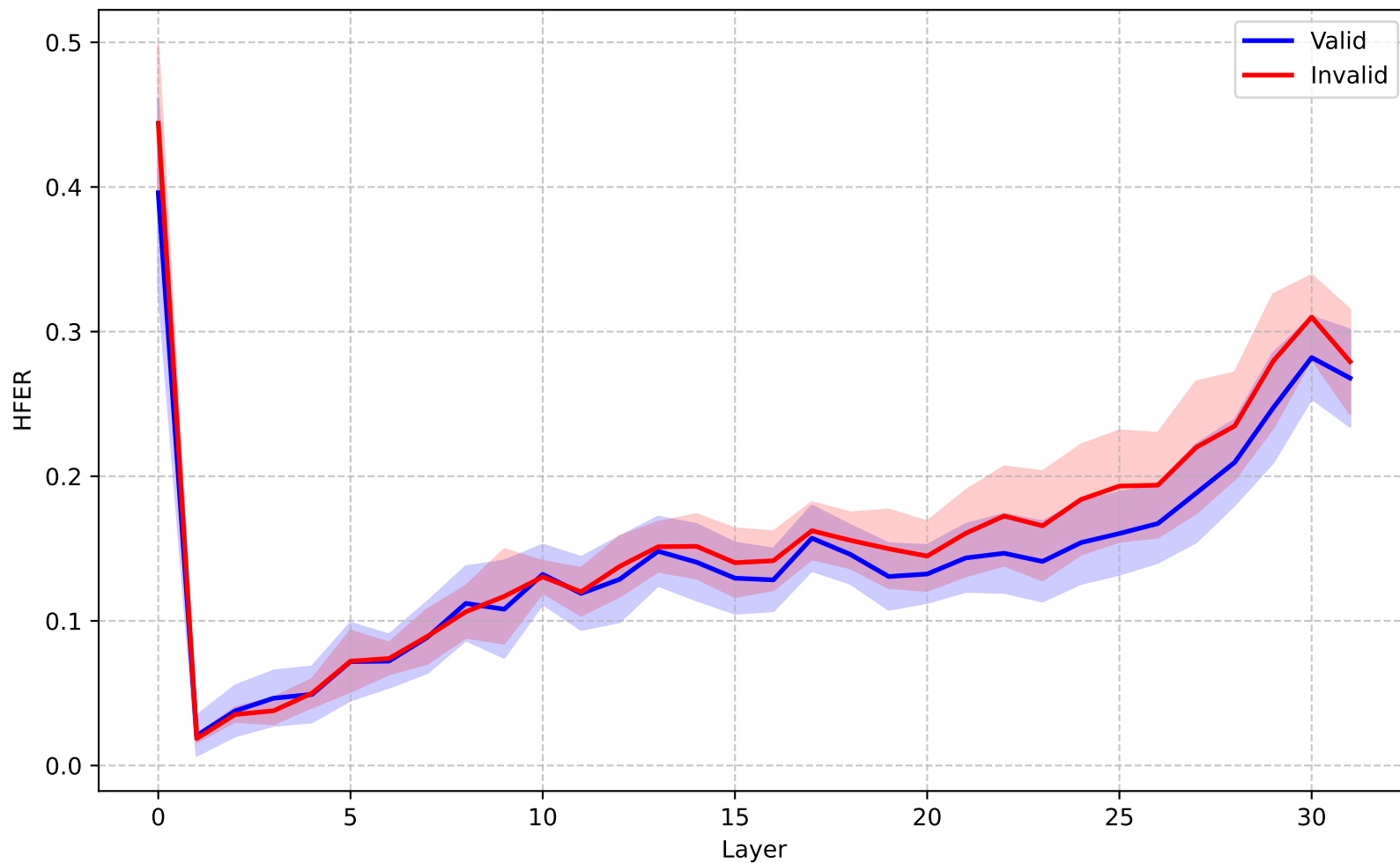
Mistral-7B (General) - HFER
