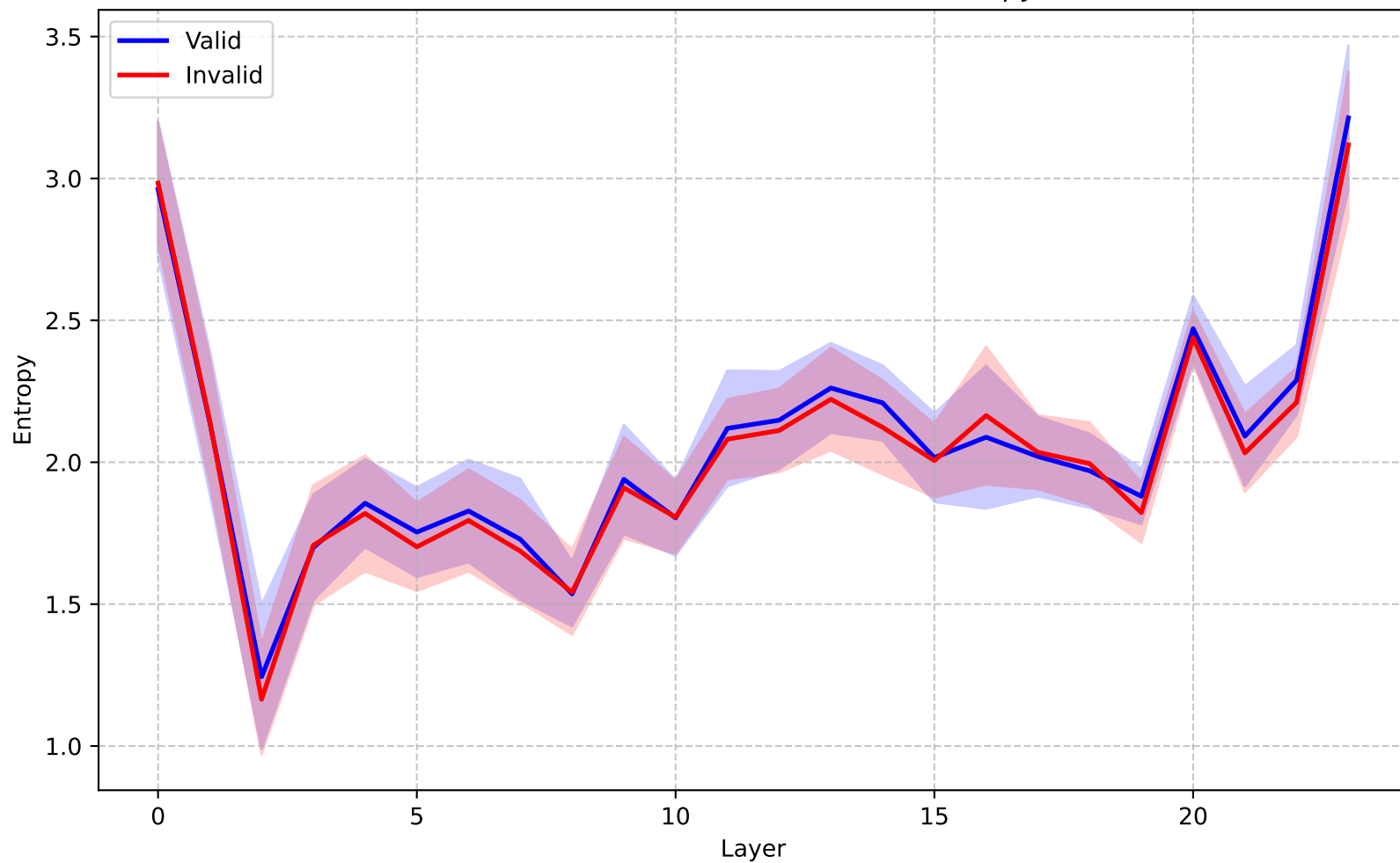
Qwen-2.5-7B (General, T=1.5) - Entropy
