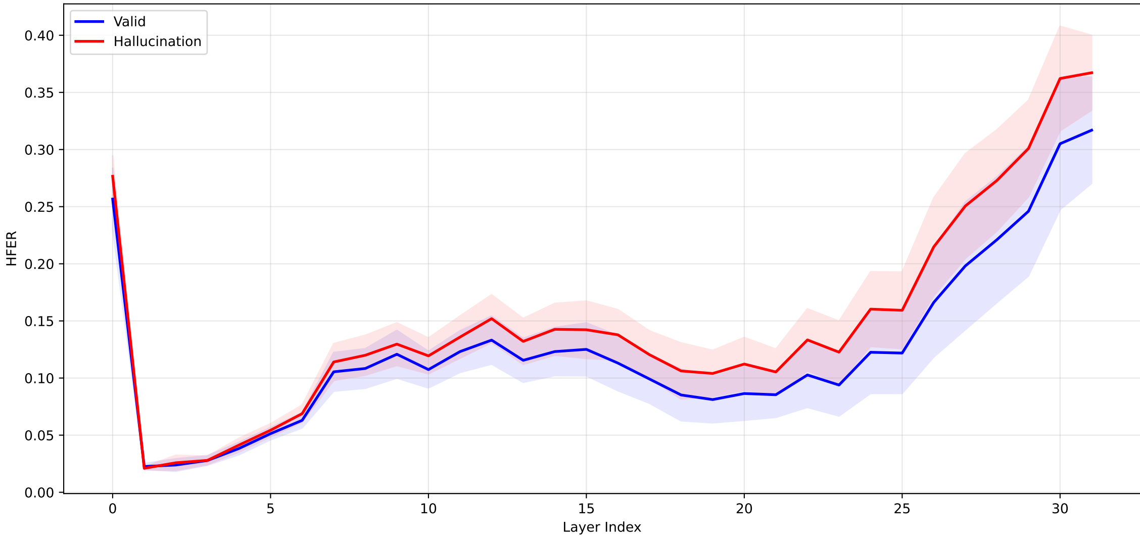
HFER across Layers (N=2261)
