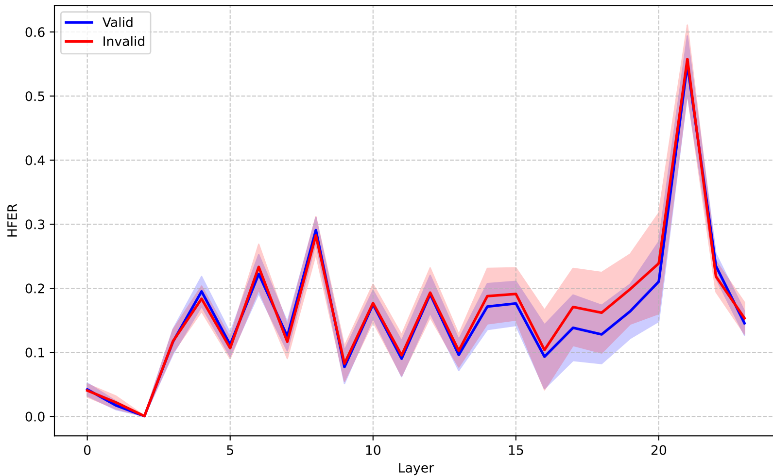
Qwen-2.5-7B (Finance) - HFER
