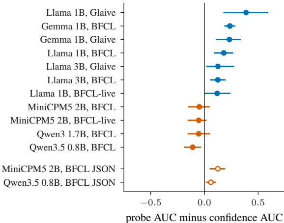
(a) every scored failure
