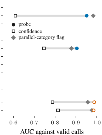
(c) dropped parallel calls, AUC
