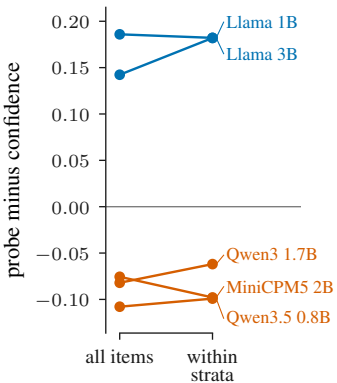
(a) difficulty held fixed
