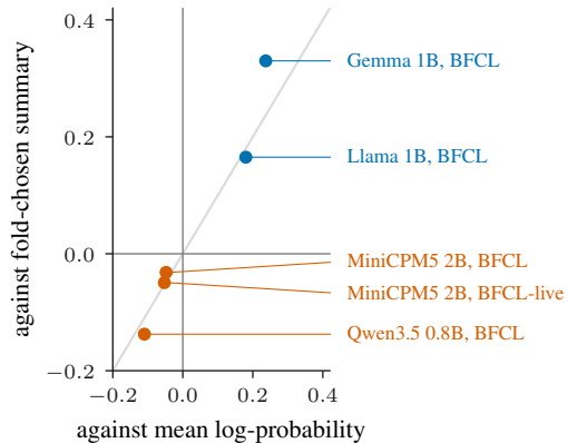
(c) confidence summary
