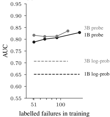
(b) failures thinned on Llama
