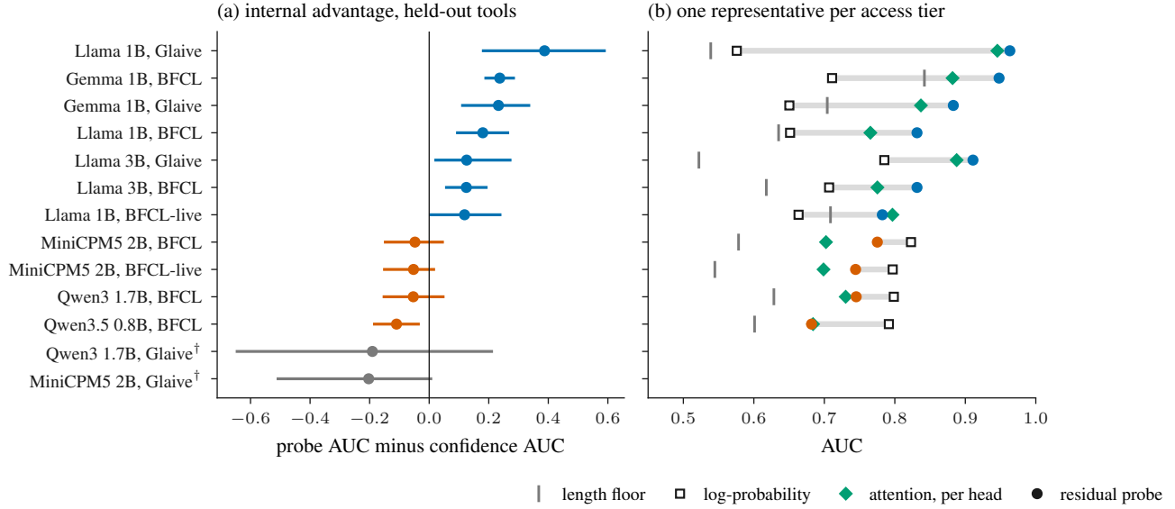
Figure 1. (a) Token-role probe AUC minus mean log-probability AUC per run on held-out tools, dot at the mean over five split seeds, bar the 95% interval from resampling tools. Blue Llama-3.2 and Gemma-3, orange Qwen3, Qwen3.5 and MiniCPM5, grey runs with fewer than thirty failures (†). (b) Per run, the length floor, the mean log-probability, the better of the per-head profile and LapEigvals, and the probe, with the interval between log-probability and probe shaded.
