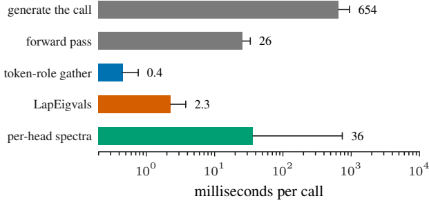
Figure 4. Cost per call of each path on Llama-3.2-1B, bar at the median over 20 BFCL prompts, line to the 90th percentile, log scale, one consumer GPU.
