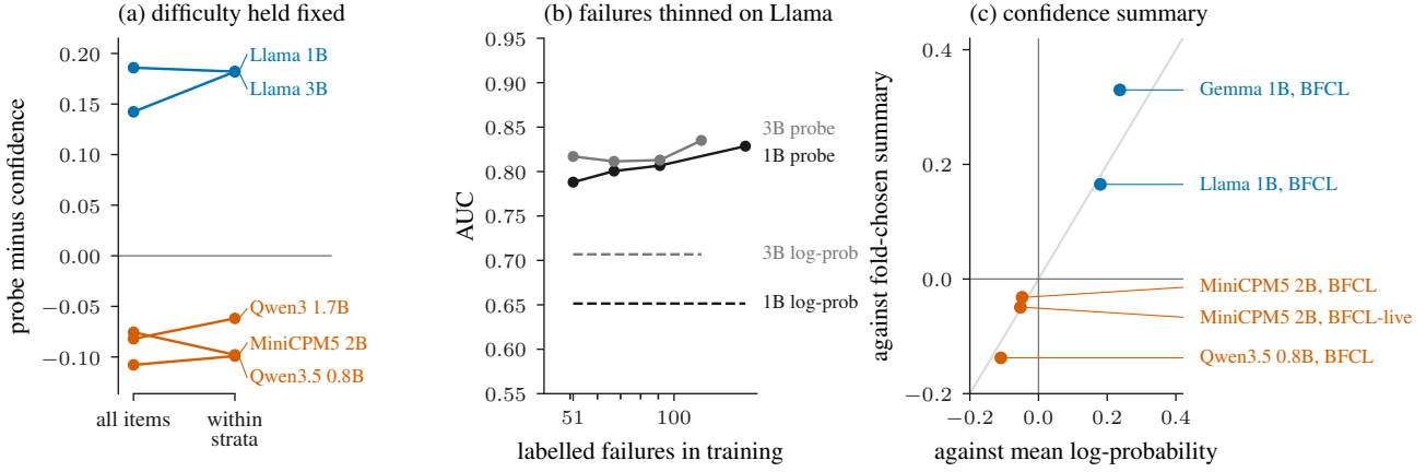
Figure 2. (a) Internal advantage per BFCL checkpoint over all items and within strata of item difficulty, where difficulty is the share of the other checkpoints that fail the item. (b) Token-role probe AUC (solid) and mean log-probability AUC (dashed) against the labelled failures available for training on Llama-3.2-1B and 3B, log scale. (c) Internal advantage against the mean log-probability and against the confidence summary chosen on training folds, one point per run that stores several summaries, identity line grey.
