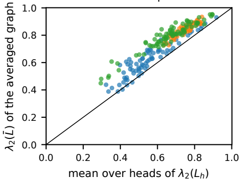
normalised Laplacian
