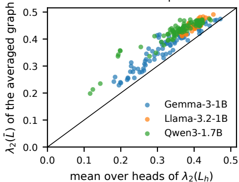
combinatorial Laplacian
