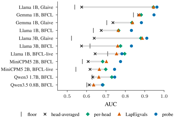
(a) attention readouts by run
