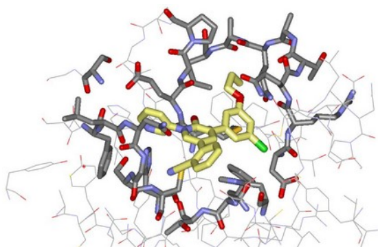
Figure 1. Rendering from a 1.8-Å crystal structure for a complex with the main protease of SARS-CoV-2 (PDB ID 7L11). Carbon atoms of the ligand are in yellow.
