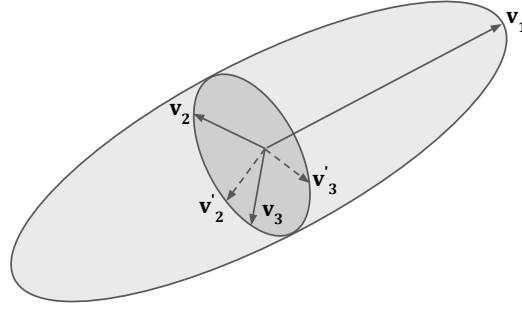
Figure 9.1: The eigenvectors associated to identical eigenvalues are not uniquely identified.
