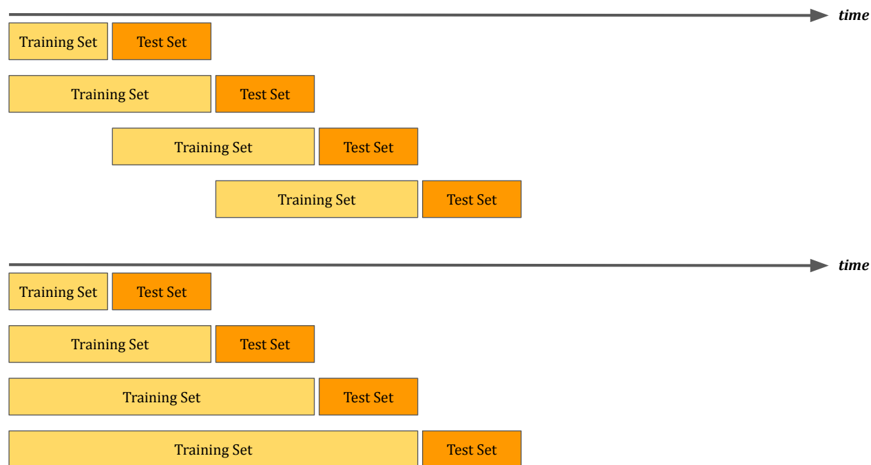
Figure 6.4: Two common walk-forward schemes. The top one uses fixed-length training data, thus preserving the estimation procedure. The bottom one uses all the available data up to certain epoch, possibly weighting data differently based on the interval from the decision epoch.
