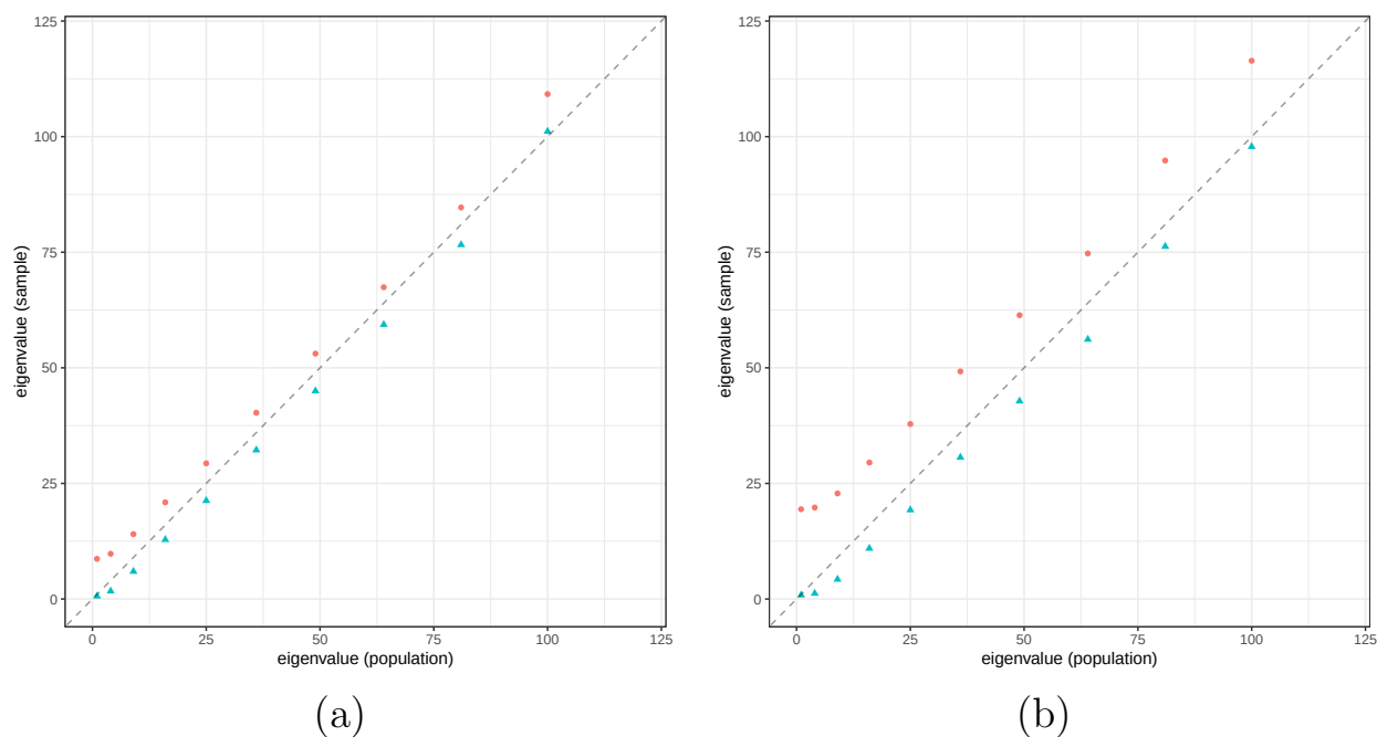
Figure 9.2: (a): Probabilistic PCA for a universe of 1000 assets, with 10 factors with volatilities 1, 2, \dots, 10 . Circle-shaped points are the sample factor variances against the true variances; triangle-shaped are the shrunk factor variances against the true variances. (b): All parameters are unchanged, with the exception of the number of assets, here equal to 3000.
