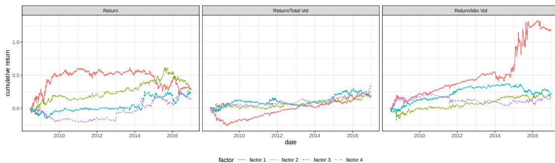
Figure 9.10: Factor returns for the first four eigenvectors. The eigenfactors are generated by PCAs on total returns, total returns/total vol, and total return/idio vol.
