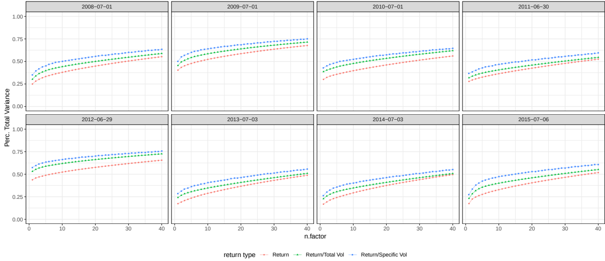
Figure 9.7: Cumulative percentage of variance described by the first n factors, for different covariance matrices.
