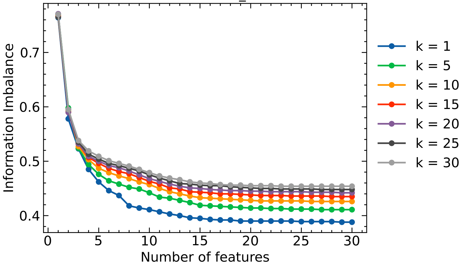
Beam search with 'n_best' = 1
