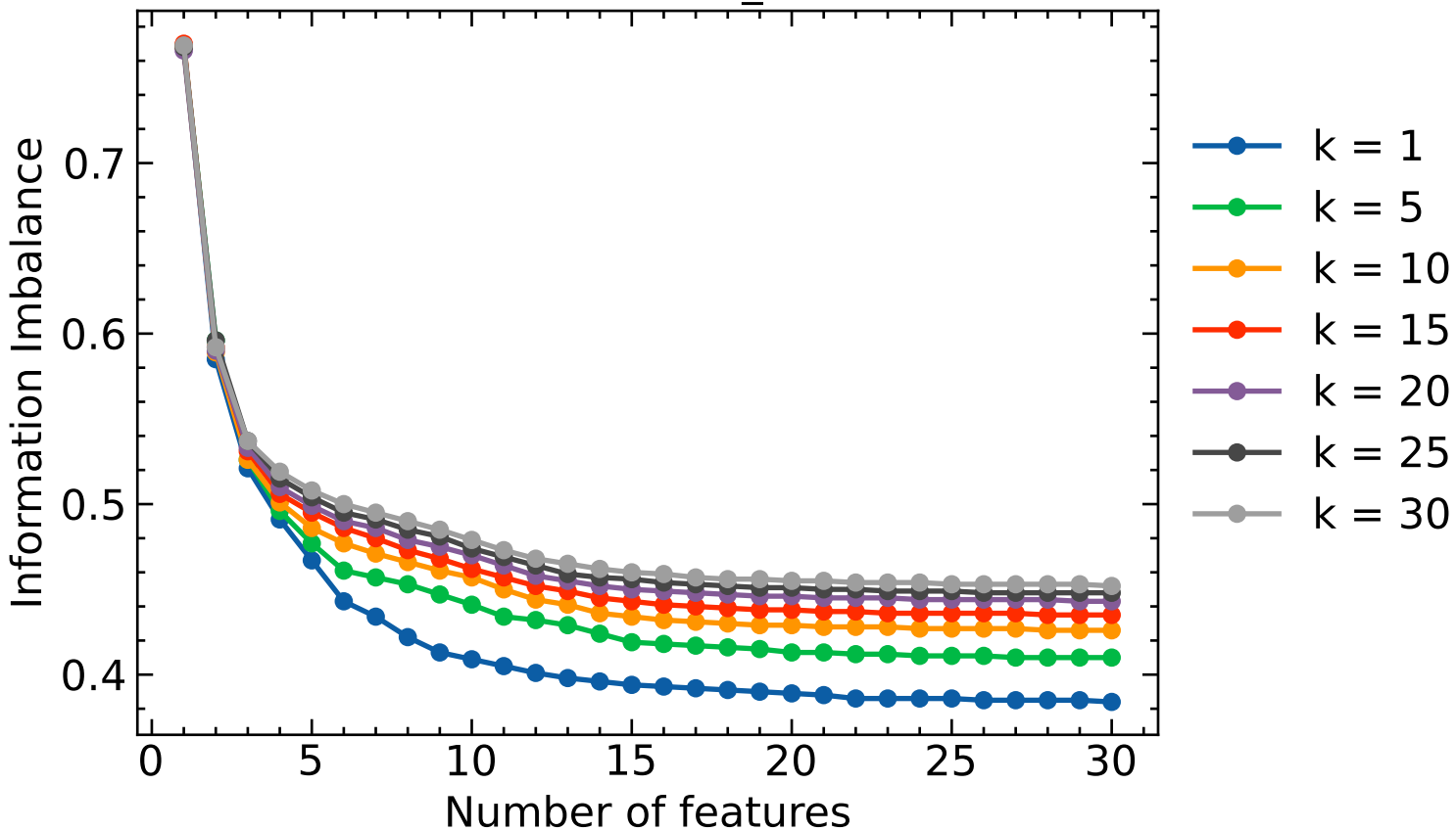
Beam search with 'n_best' = 20
