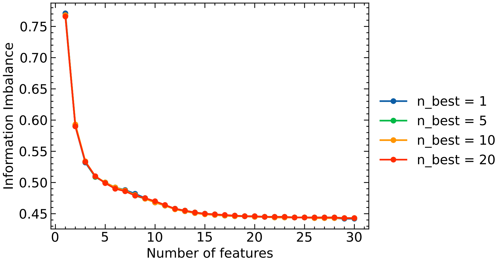
Beam search with 'k' = 20
