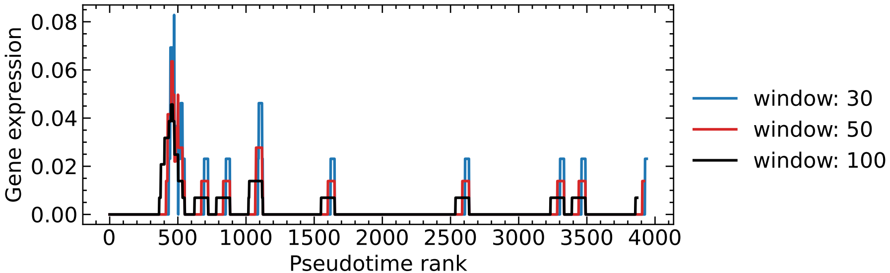
Gene CALML6
