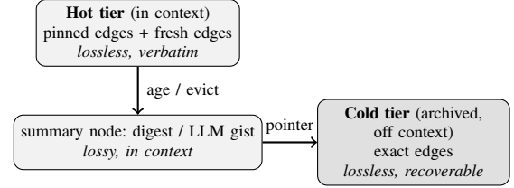
Fig. 2. Two-tier edge aging. Pinned and fresh edges stay verbatim in context; aged ephemera collapse to an in-context summary that points to their byte-exact edges in a cold archive, so the in-context state shrinks while nothing is lost.
