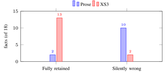
Fig. 1. Budgeted compaction (Study S7). Prose retains few facts and silently corrupts many; XS3 retains most and, when it sheds, omits whole edges rather than corrupting what it keeps.
