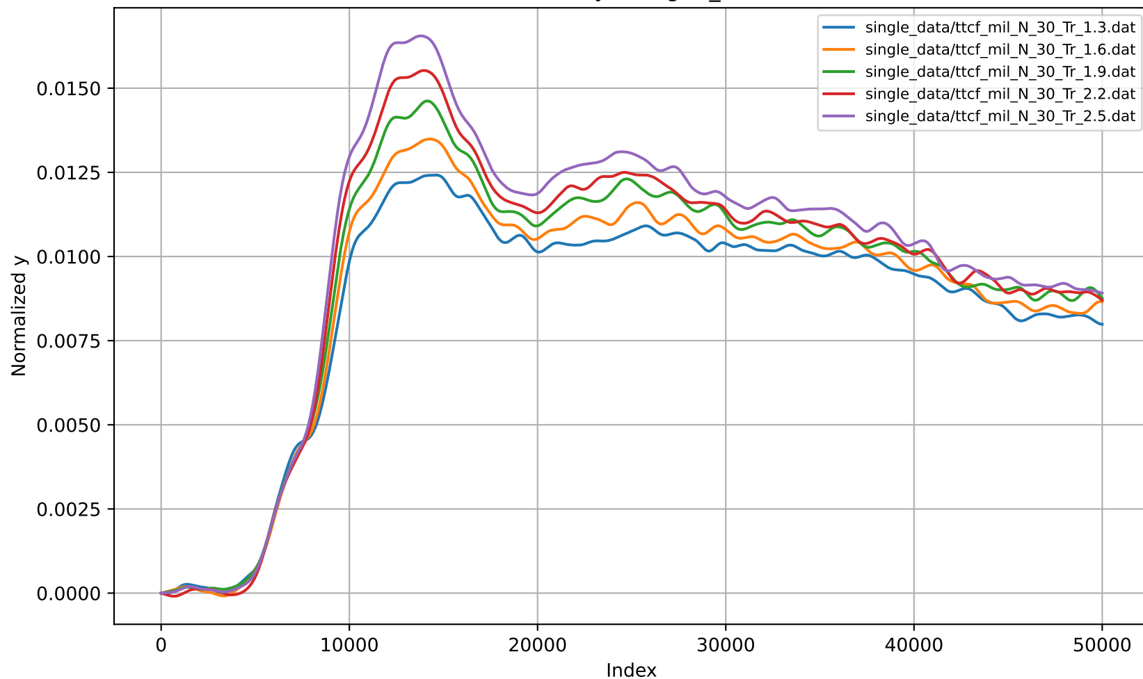
All Normalized y (integral_df) - N=30
