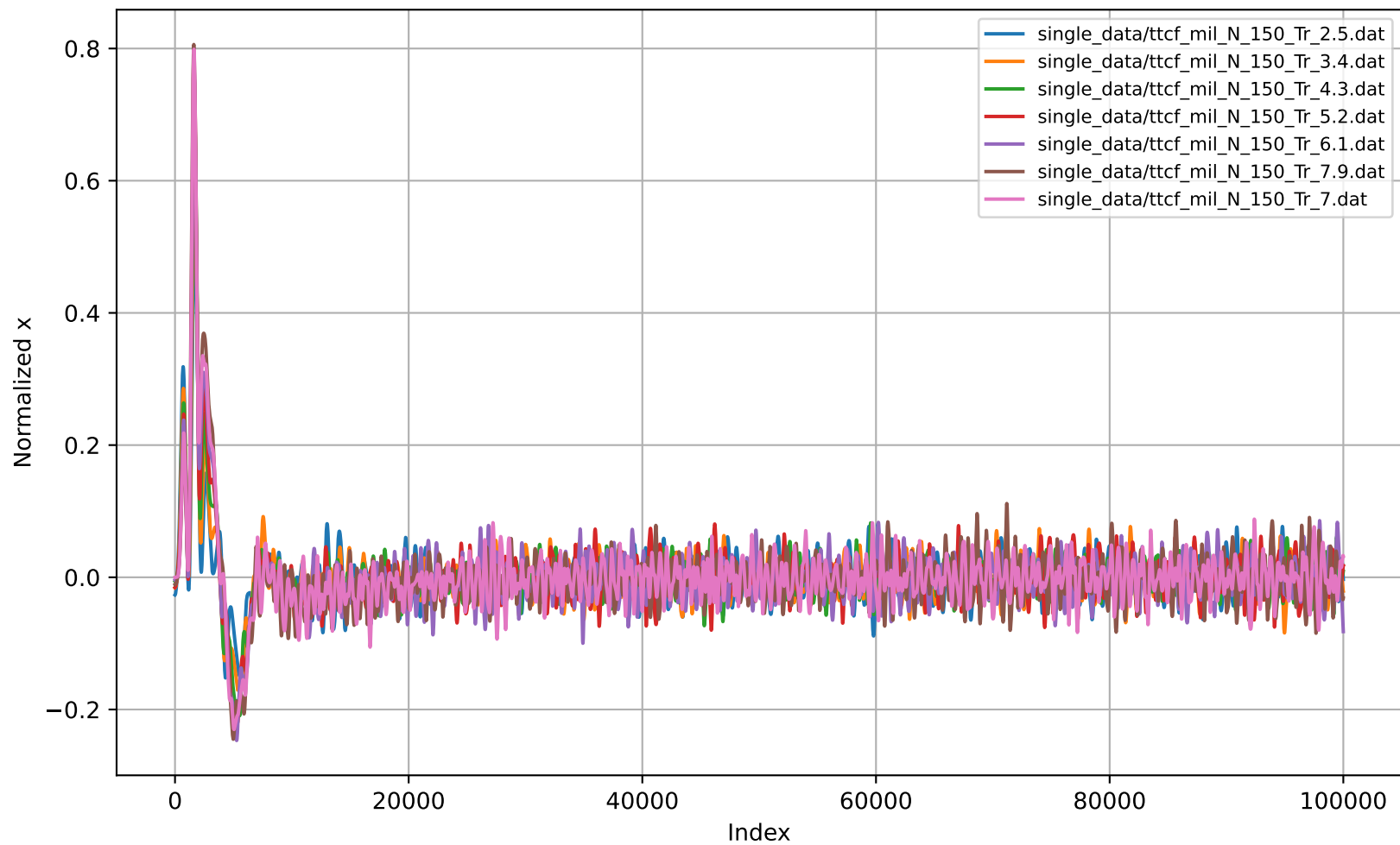
All Normalized x (df) - N=150
