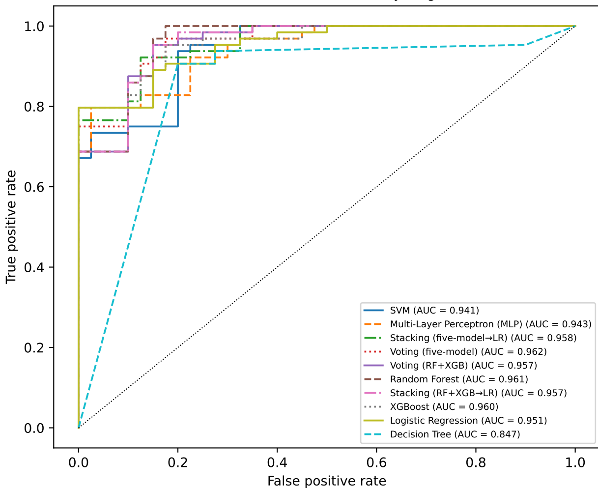
Hold-out ROC curves — Early Stage
