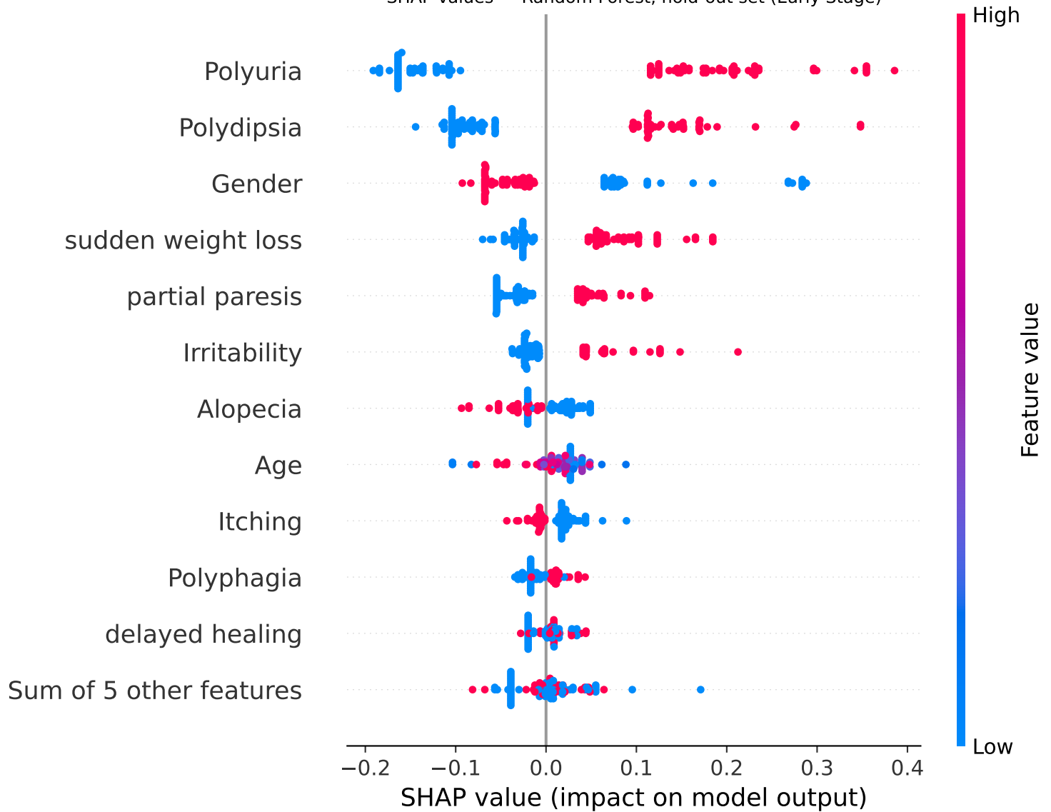
SHAP values — Random Forest, hold-out set (Early Stage)
