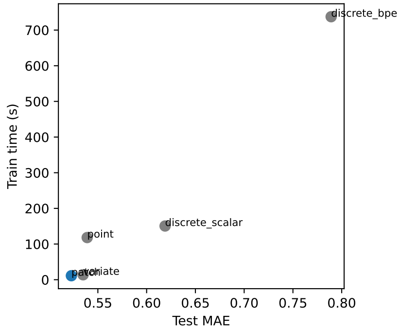
ETTh1/H=336: MAE vs. time
