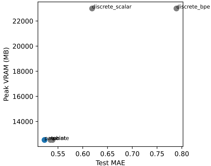
ETTh1/H=336: MAE vs. VRAM
